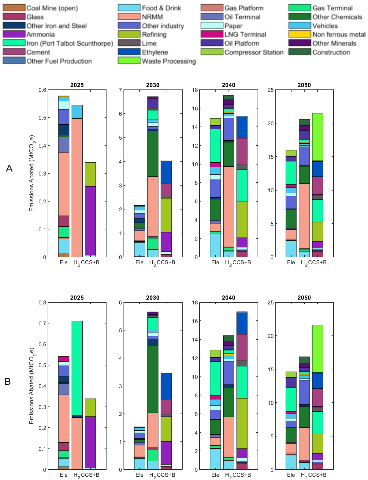
Figure A 5 Abated emissions for sectors by technology type per year- (A): Discount rate 3%, (B): Discount rate 15%
