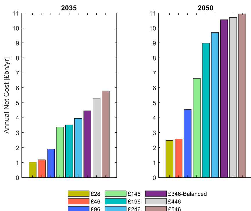
Figure 19: Effect of carbon price on net cost
