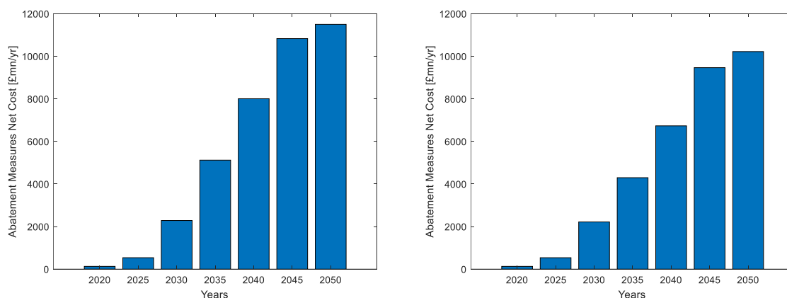
Figure A 2 Abatement measures annual net cost - (left): Resource Efficiency 0%, (right): Resource Efficiency 150%
