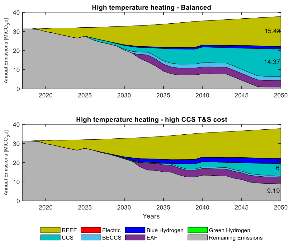
Figure 37: Abatement for high temperature processes
