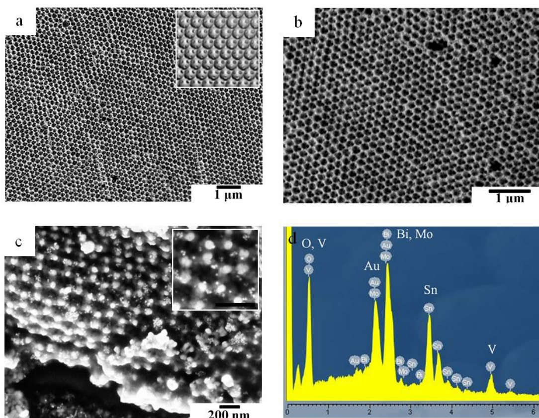
Figure 2. (a-b) SEM images of io-Mo:BiVO 4 prepared from colloidal crystal templates of polystyrene spheres with (a) 260 nm diameter and (b) 320 nm diameter. (c) Cross-sectional SEM image of io-Mo:BiVO 4 after introducing 20 nm Au NPs (The scale bar in the inset is 200 nm). (d) Energy dispersive spectrometry (EDS) of the as-prepared io-Mo:BiVO 4 (elemental Sn derives from FTO-coated glass). Inset of a is a computed top view inverse opal structure.
