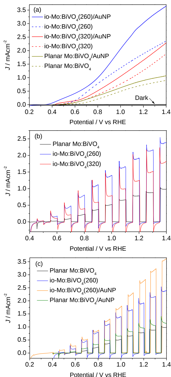
Figure 5. (a) LSV under AM 1.5G illumination ( 100 \text{ mW cm}^{-2} ) and dark response (dash lines). (b) LSV recorded under chopped illumination. (c) LSV of the electrodes with and without Au NPs recorded under chopped illumination. All runs were recorded with a scan rate of 10 \text{ mV s}^{-1} at 25^\circ \text{C} in an aqueous phosphate buffer as electrolyte at pH 7.
