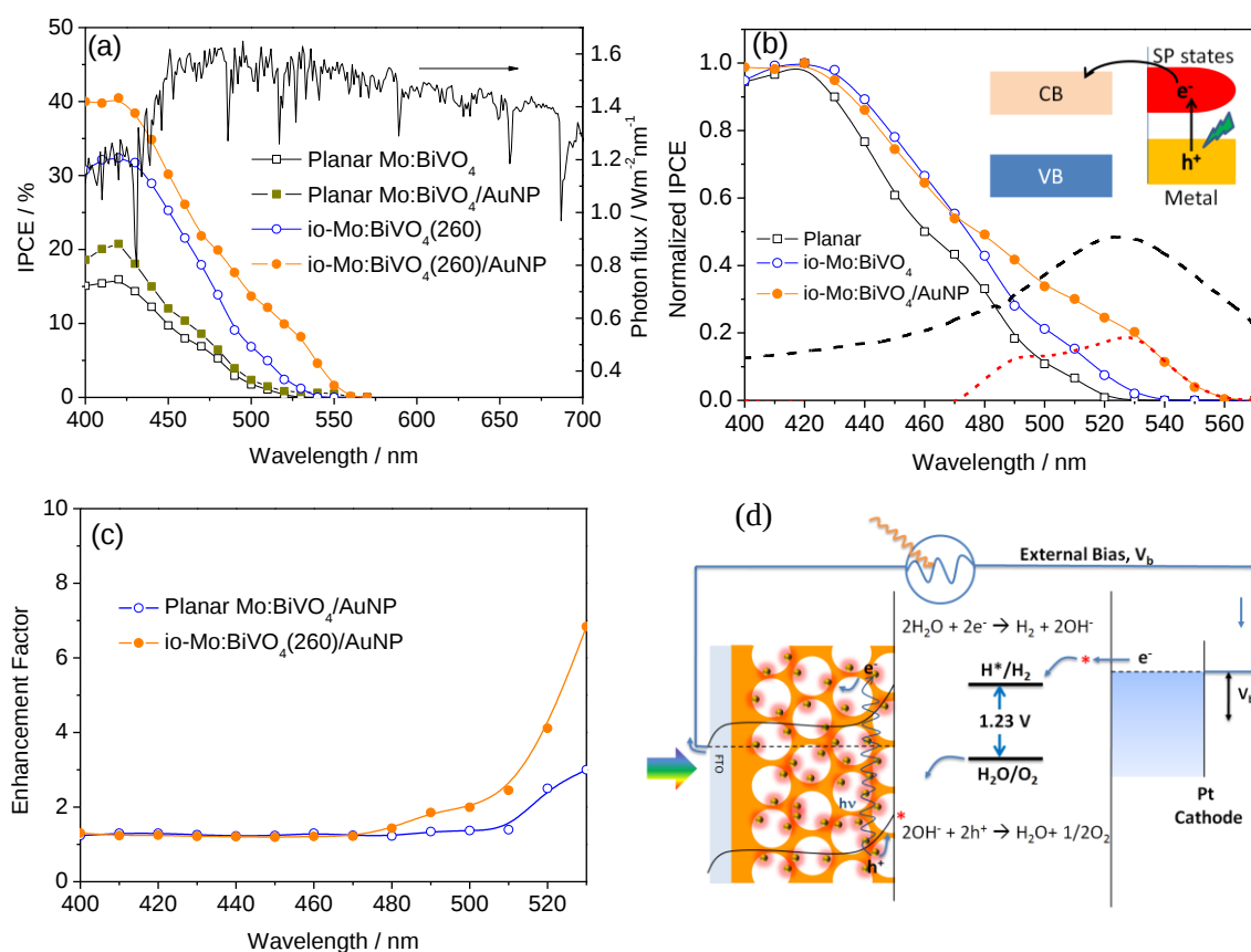
Figure 6. (a) IPCE spectra of the different electrodes at an applied potential of 1.1 V and the AM 1.5 G 100 mW cm -2 solar spectrum. (b) IPCE normalized to the IPCE maximum at 420 nm, red dash line is the difference in normalized IPCE spectra after Au NPs infiltration, black dash line shows localized surface plasmon extinction of the 20 nm Au NPs. Inset is an illustration of LSPR-induced charge transfer mechanism. (c) IPCE enhancement factor (see text). (d) Schematic illustration of solar water splitting with io-Mo:BiVO 4 /AuNP nanophotonic photoanode.
