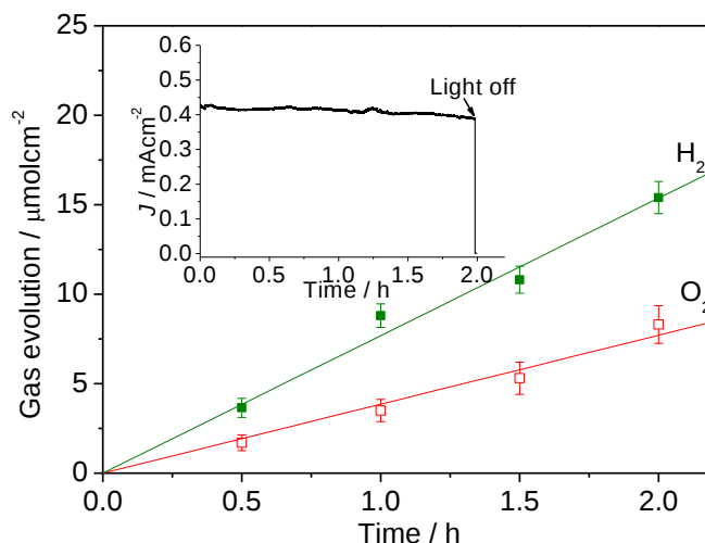
Figure 8. Gas evolution at an applied potential of 0.6 V (vs. RHE), inset is the photocurrent response measured during water splitting.
