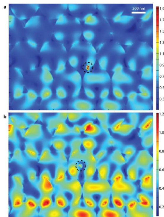
Figure 7. The simulated electric field distribution for gold nanoparticle (in the black dashed circles) modified BiVO 4 inverse opal at \lambda = 533 nm. The 20 nm gold nanoparticle is either (a) on the inverse opal wall, or (b) in the centre of one of the pores in the inverse opal away from the wall.
