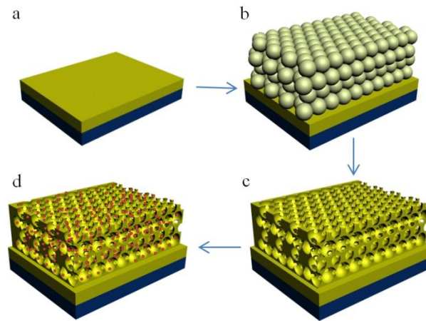
Figure 1. Illustration of synthetic strategy. (a) An un-patterned layer of Mo:BiVO 4 with thickness of 150 nm is deposited on FTO-coated glass. (b) A colloidal crystal template is formed on the top surface by evaporation-induced self-assembly. (c) The precursor is infiltrated, and the template removed to form an inverse opal structure. (d) Surface plasmon effects are introduced by infiltrating Au NPs into the io-Mo:BiVO 4 .
