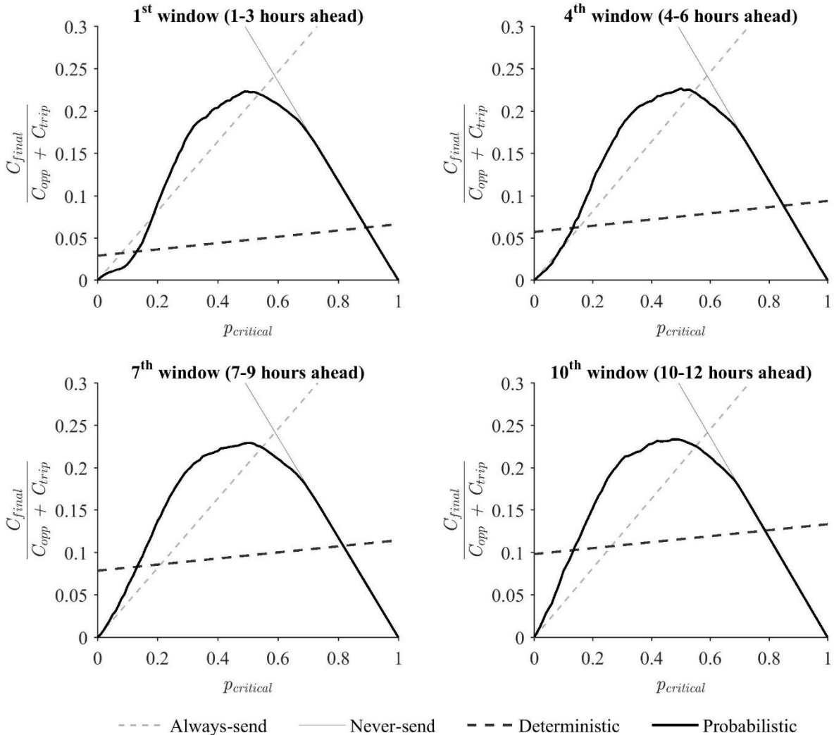
Fig. 5. The comparison of the costs based on four approaches: (a) always send the vessel, (b) never send the vessel, (c) use the deterministic point forecasts of KDE with a window length of 4 hours, and (d) use probabilistic forecasts from this method.
