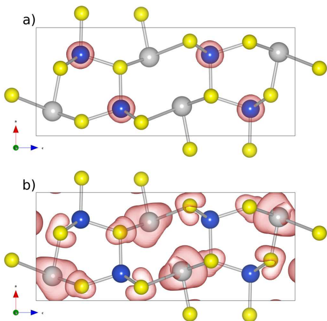
Fig. 3 (Colour online) Charge density calculated for a) the top of the valence band ( E - E_F = -3.5 \rightarrow 0 \text{ eV} ) and b) the bottom of the conduction band ( E - E_F = 1 \rightarrow 5 \text{ eV} ) in \text{CuSbS}_2 . Colours are similar to Figure 1; Cu (blue), Sb (grey), S (yellow), charge density (red)
