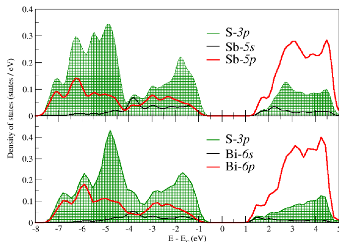
Fig. 4 (Colour online) Partial orbital-projected density of states for CuSbS 2 (top) and CuBiS 2 (bottom)
