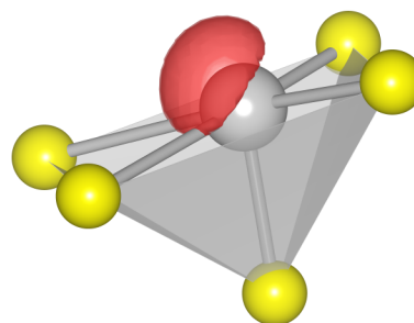
Fig. 5 (Colour online) SbS 5 square pyramid with lone pair electron density shown in red, Sb in grey and S in yellow
