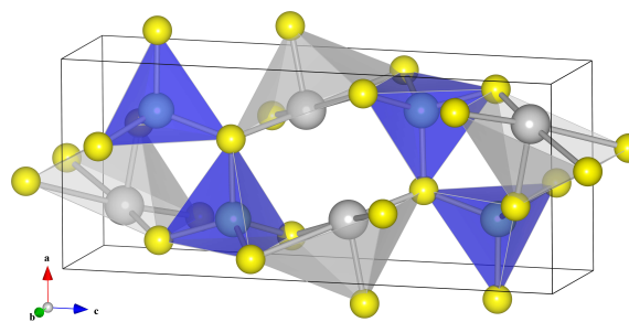
Fig. 1 (Colour online) Structure of CuMS 2 (where M = Sb or Bi) showing CuS 4 tetrahedra (blue), MS 5 square pyramidal units (grey) and S atoms (yellow).
