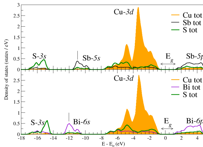
Fig. 2 (Colour online) Orbital-projected density of states for CuSbS 2 (top) and CuBiS 2 (bottom) indicating the Cu, Sb, Bi and S states.
