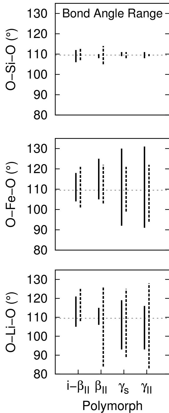
Figure 4: Range of bond angles in the \text{LiO}_4 , \text{FeO}_4 and \text{SiO}_4 tetrahedra of the \text{Li}_2\text{FeSiO}_4 and delithiated \text{LiFeSiO}_4 structures (filled and dashed lines respectively) as a measure of the tetrahedral distortion. The horizontal dashed line is the ideal tetrahedral angle.
