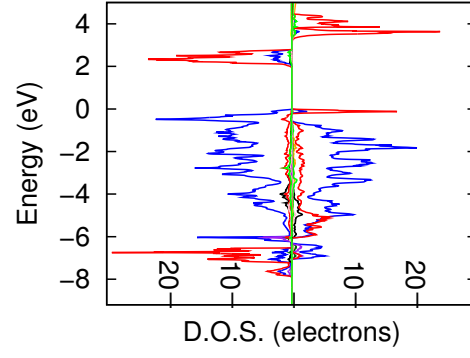
(a) \beta_{II} -phase
