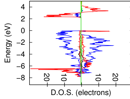
(b) \gamma_s -phase
