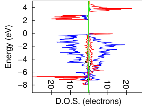
(c) \gamma_{II} -phase
