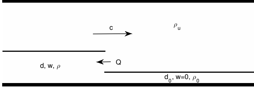
FIGURE 5. Schematic of steady shock travelling at speed c into a quiescent fluid of density \rho_0 . The shock entrains fluid of density \rho_u which is assumed to mix behind the shock.
