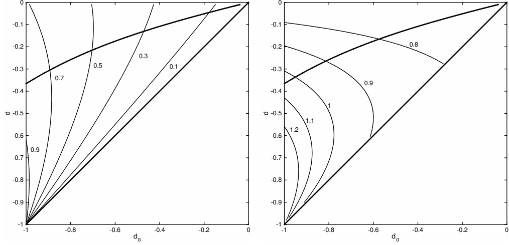
FIGURE 6. Properties of an energy conserving shock of amplitude d moving into a quiescent state of amplitude d_0 Left: Contours of the downstream (oncoming flow) Froude number u/\sqrt{h} . Right: Contours of the shock Froude number c/\sqrt{h} . The upper bold curve corresponds to the limiting shock satisfying the Lax condition. Thus allowable shocks are inside the region bounded by the bold curves.
