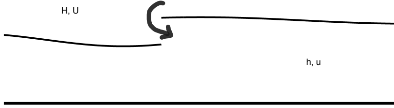
FIGURE 2. Schematic of the two-layer, one interface flow. A shock is shown entraining lighter fluid into heavier fluid, a situation considered later in the paper.
