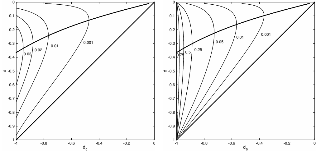
FIGURE 7. Properties of an energy conserving shock of amplitude d moving into a quiescent state of amplitude d_0 Left: Contours of the entrainment of upper fluid into the lower layer. Right: Contours of the density change across the shock in units of the mean density difference between the layers. The region bounded by the bold curves are allowable shocks.
