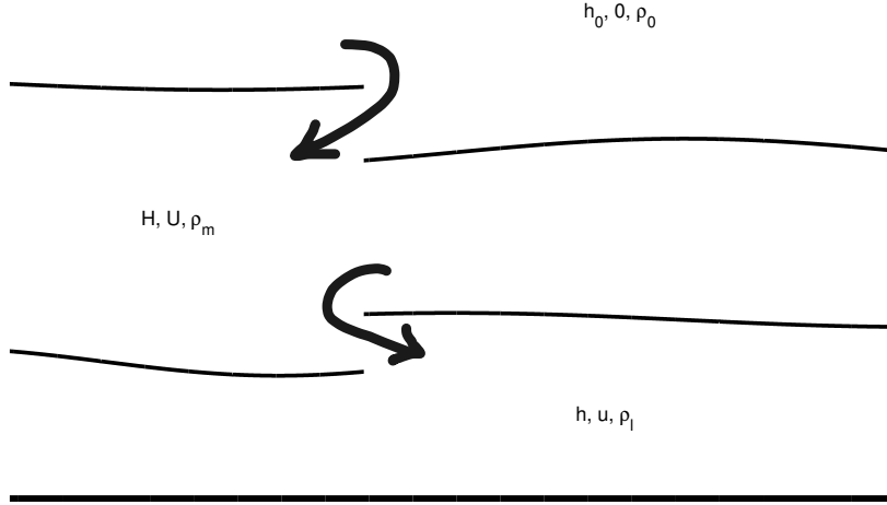
FIGURE 1. Sketch of the physical problem. Shown are the free surfaces and a baroclinic entraining shock. The horizontal bottom is at z = 0 .
