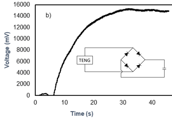
Figure 2. (a) Open-circuit voltage for the flat samples of copper and polyimide. (b) Charging a 0.1\ \mu\text{F} capacitor and schematic of the rectifying circuit.
