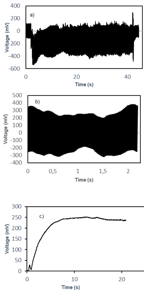
Figure 8. (a) Open circuit voltage obtained with the one-piece device. (b) Open circuit voltage in a short time scale (c) Charge of a capacitor of 0.1μF.
