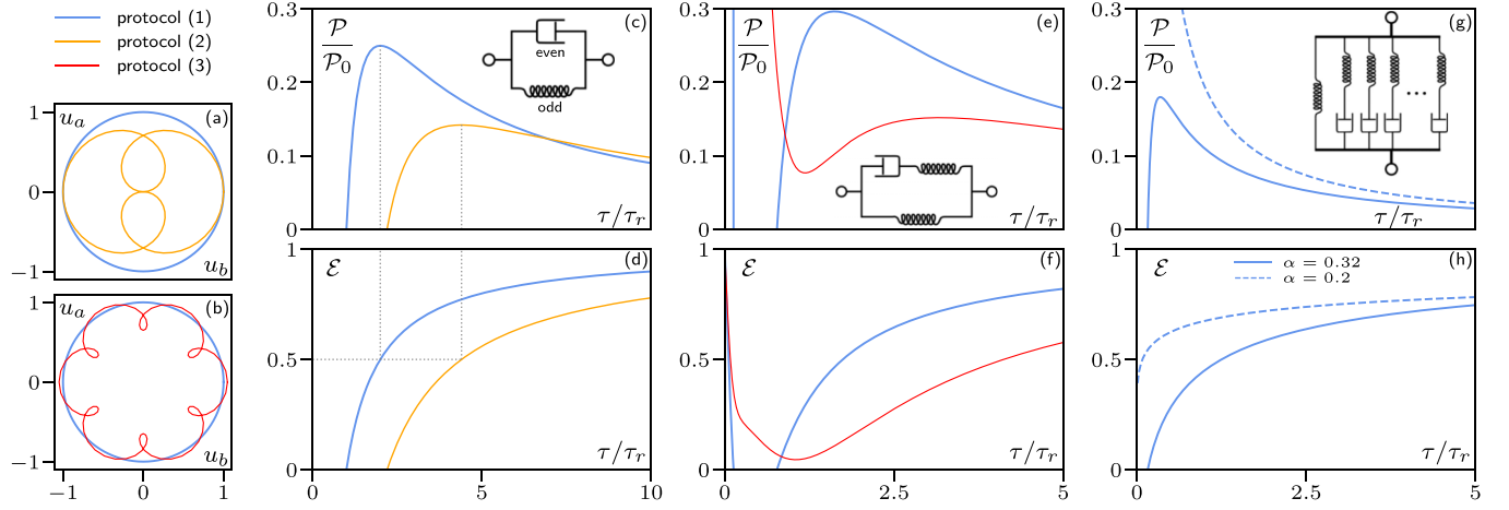
FIG. 2. Performances of odd materials under various protocols. (a), (b) Three cyclic protocols in strain space \{u_a, u_b\} with same quasistatic work ( \mathcal{W}_{qs} = 2\pi K \sum_n n a_n^2 ): (1) circular protocol, a_n = \delta_{n,1} , (2) noncircular protocol, a_n = (1/2)(\delta_{n,1} + \delta_{n,3}) , and (3) noncircular protocol, a_n = (1/5)(3\sqrt{2}\delta_{n,1} + \delta_{n,7}) , see Eq. (7). (c)–(h) Power and efficiency, respectively, \mathcal{P} and \mathcal{E} , as functions of the cycle time \tau , where \tau_r is a relaxation time scale and \mathcal{P}_0 = \mathcal{W}_{qs}/\tau_r is a reference power. We compare these metrics \{\mathcal{P}, \mathcal{E}\} for three materials subject to the protocols in panels (a), (b). The material mechanics is characterized by the odd storage modulus g' and even loss modulus g'' [see Eq. (6)]: (c), (d) odd Kelvin-Voigt (KV) solid [Eq. (9)], (e), (f) odd standard linear (SL) solid [Eq. (11)], and (g), (h) odd power-law (PL) solid [Eq. (12)]. The insets display some schematic representations of each material in terms of even/odd dampers and springs. (c), (d) KV solids exhibit a tradeoff between power (maximum at intermediate \tau ) and efficiency (maximum at large \tau ). The efficiency at maximum power is always 1/2 independently of the protocol details, see dotted lines. Noncircular protocols systematically reduce both the efficiency at all times and the maximum power. (e), (f) SL solids have diverging power at small \tau , and maximum efficiency at both small and large \tau . The engine cannot extract work in an intermediate regime of \tau (where \mathcal{P} < 0 and \mathcal{E} < 0 ) for circular protocols (blue line), yet it can extract work at all \tau for some noncircular protocols (red line). (g), (h) PL solids have either diverging power at small \tau (when \alpha < 1/4 ), or maximum power at intermediate \tau (when \alpha > 1/4 ). The efficiency is always maximum at large \tau . Parameters: K = 1 , \tau_r = 1 , \lambda = 0.1 .
