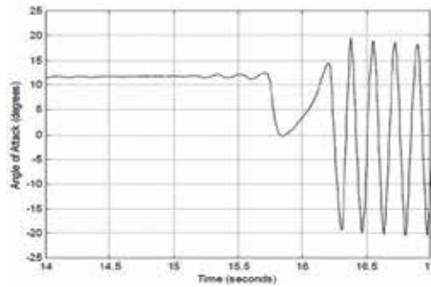
Figure 28. Flutter response- an excerpt from [23]
