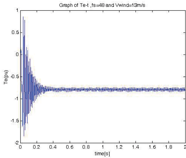
Figure 13. Electrical torque when f_s = 48 and u_w = 13\text{m/s} .
