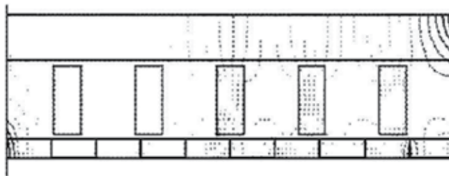
Figure 7. Flux lines in maximum force position
