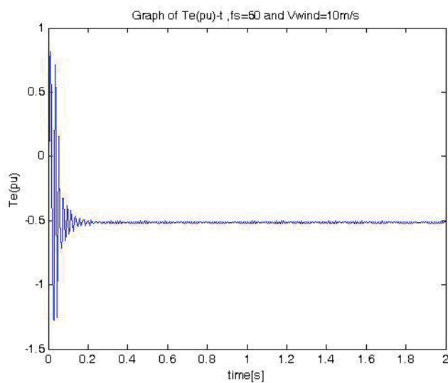
Figure 11. Electrical torque when f_s = 50 and u_w = 10\text{m/s} .
