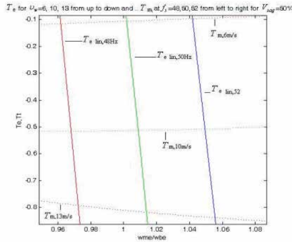
Figure 6. Mechanical and electrical torque versus frequency per unit with V_{\text{sag}} = 50\% .
