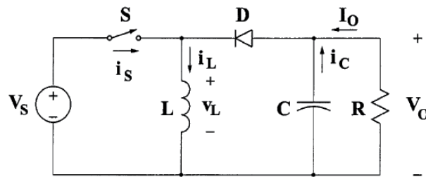
Figure 9. Basic circuit of a buck-boost switching regulator
