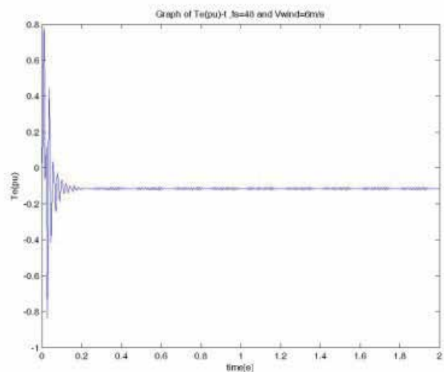
Figure 7. Electrical torque when f_s = 48 and v_w = 6 m/s.
