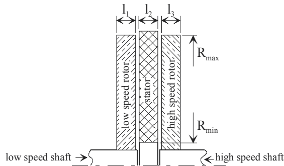
Figure 16. Main dimensions of the speed multiplier
