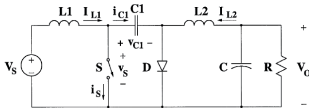
Figure 11. Basic circuit of a cuk switching regulator
