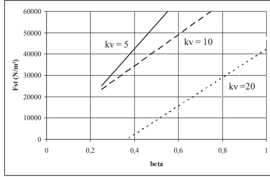
Figure 8. Tangential force density for different values of k_v ( B_{ar} = 1.2 T)
