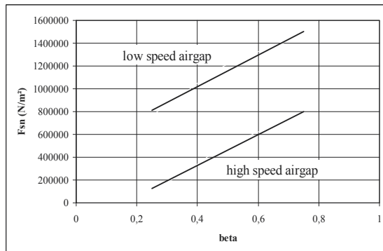
Figure 9. Normal force density ( k_v = 10 )
