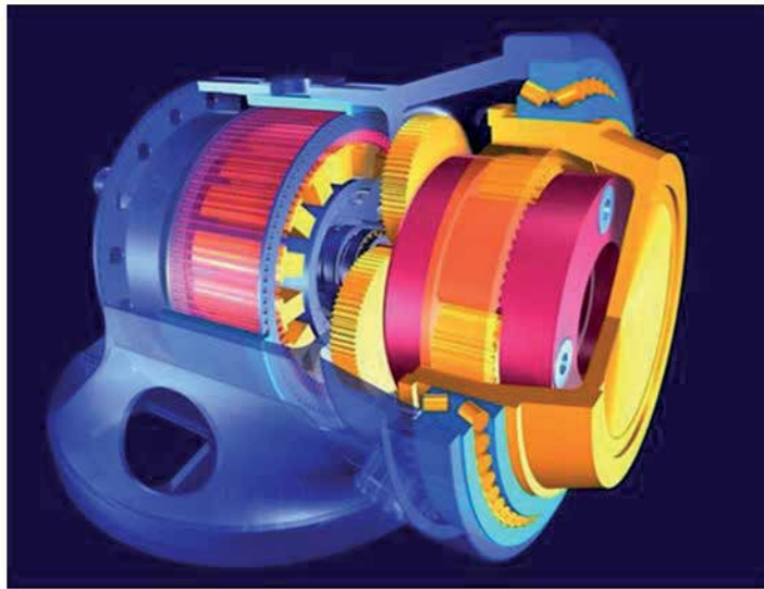
Figure 8. Cutaway of a permanent magnet synchronous generator [18].
