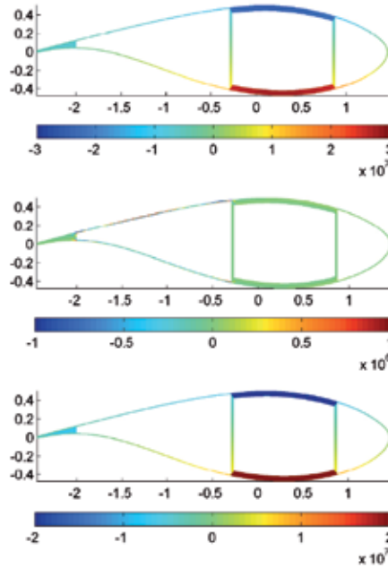
Fig. 11. Components of the Jaumann-Biot-Cauchy stress tensor \mathbf{Z} = \mathbf{S}\boldsymbol{\Gamma} for the section located at 40% of the blade span (referred to the undeformed coordinate system (X^1, X^2, X^3) in Pa). From top to bottom: Z_{22} , Z_{23} and Z_{33} .
