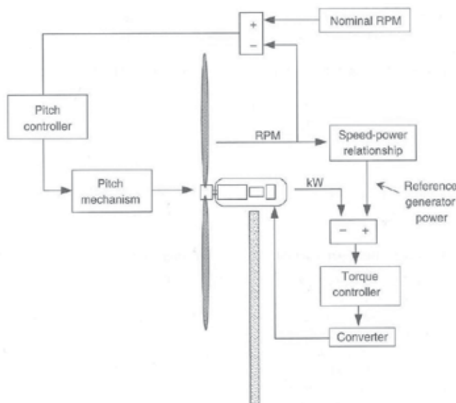
Figure 15. Variable speed control system [35].
