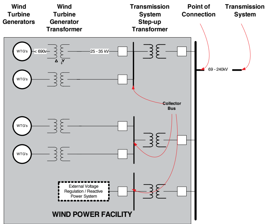
Figure 2. Wind power facility diagram – AESO [7].
