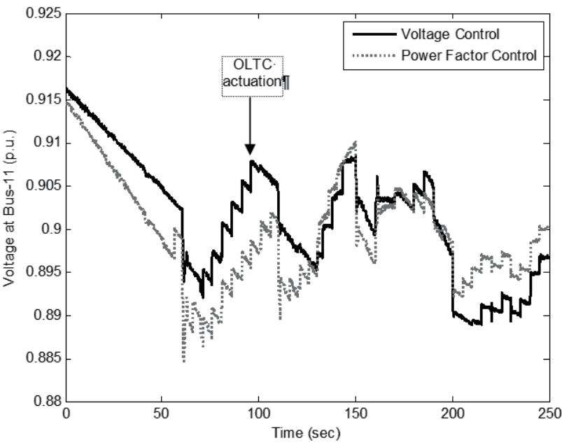
Figure 7. Voltage at bus 11
