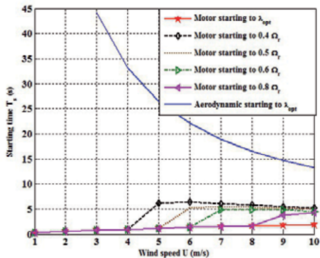
Figure 12. Starting time for aerodynamic and motor starting.
