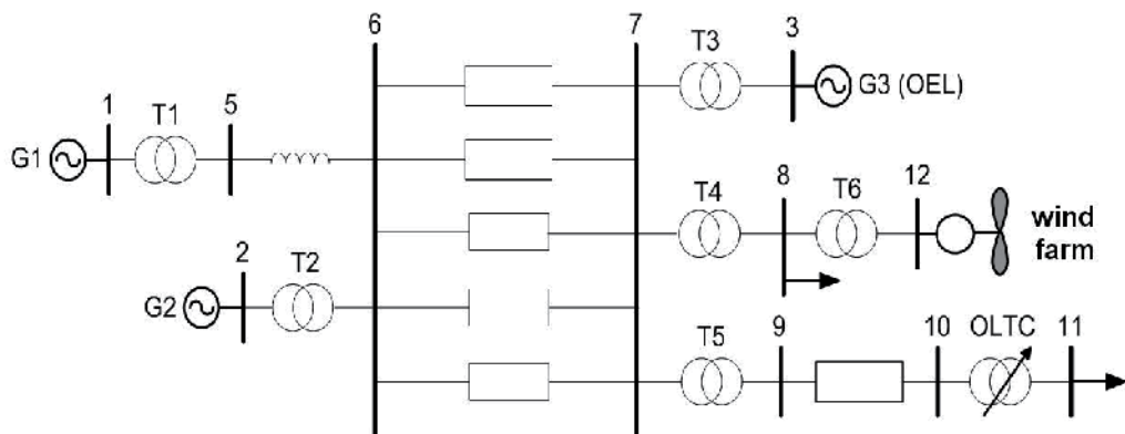
Figure 5. Test system diagram.
