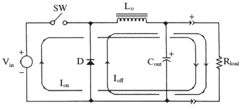
Figure 4. Basic circuit of a buck switching regulator
