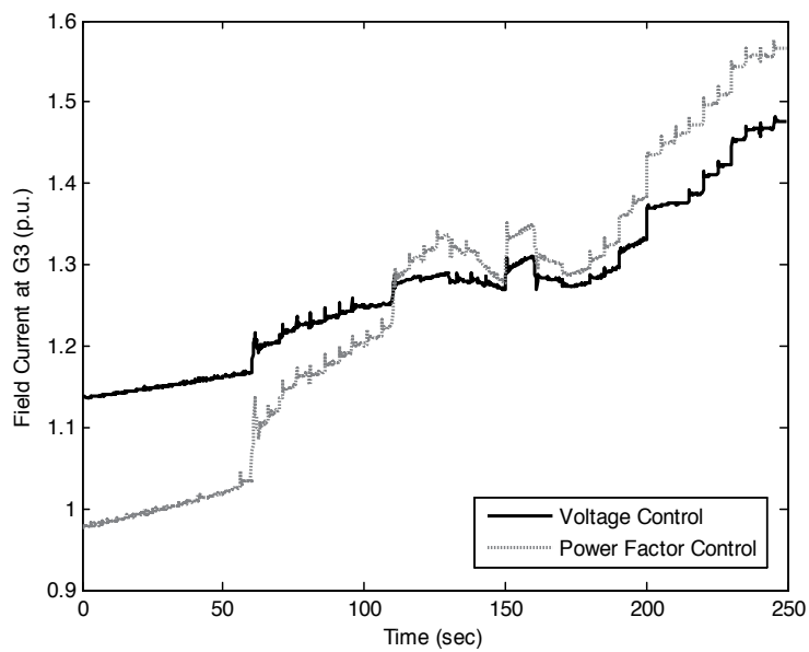
Figure 10. Field current at G3.
