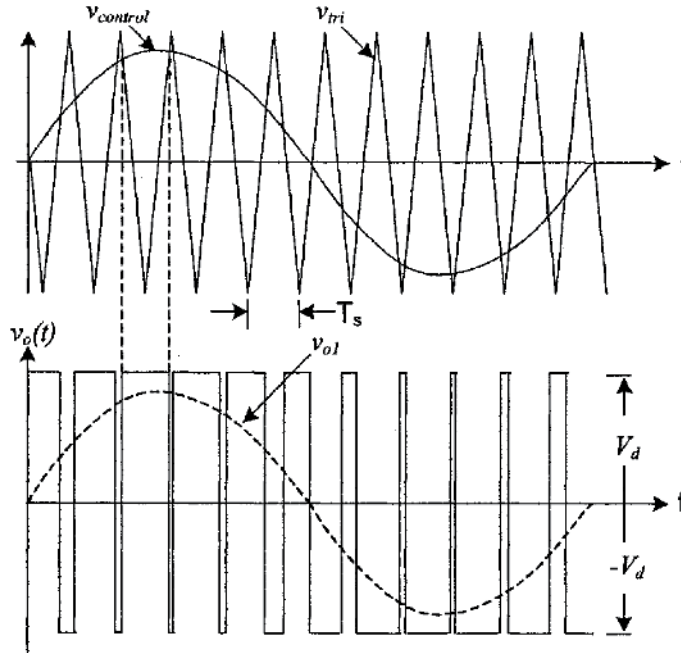
Figure 15. Unidirectional SPWM.
