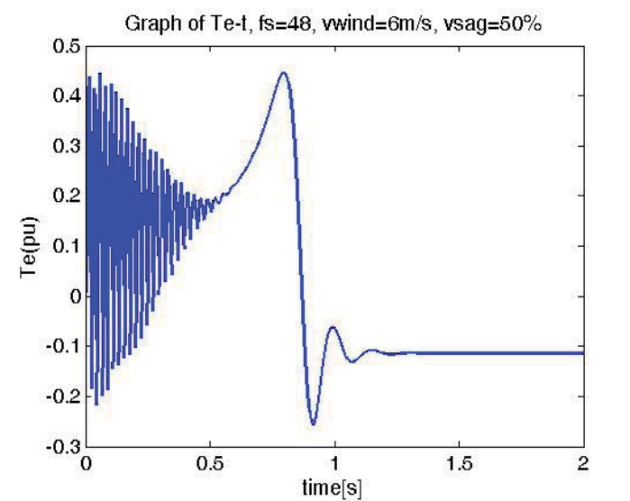
Figure 22. Torque-time in per unit while V_{sag}=50\% and u_w=6\text{m/s} , f_s=48
