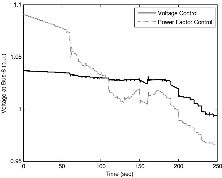
Figure 8. Voltage at bus 8
