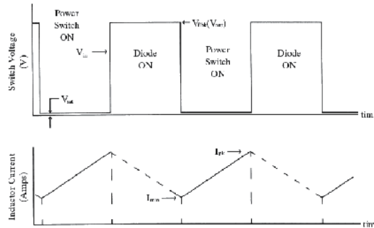
Figure 8. Waveforms for a continuous-mode boost converter.
