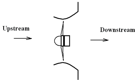
Figure 2. Schematics of the shrouded wind turbine. There is a vertical element at the exit of the wind turbine. This element contributes to reducing the power at the downstream side of the turbine, an effect that extracts more air through the wind turbine. (Idea reproduced similar to the description given by Ohya [40].)
