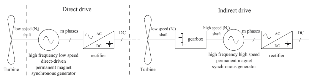
Figure 1. Linking the wind turbine to the generator
