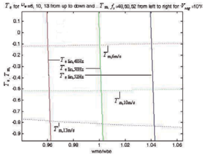
Figure 4. Mechanical and electrical torque versus frequency curves per unit with V_{sag} = 10\% .
