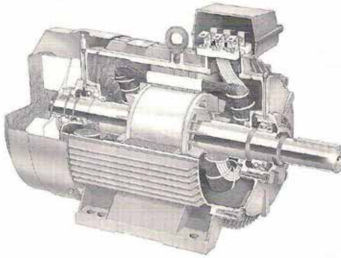
Figure 10. Cutaway of a squirrel-cage induction generator [22].
