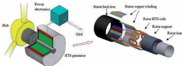
Figure 9. Schematic of a HTS synchronous generator system [11].
