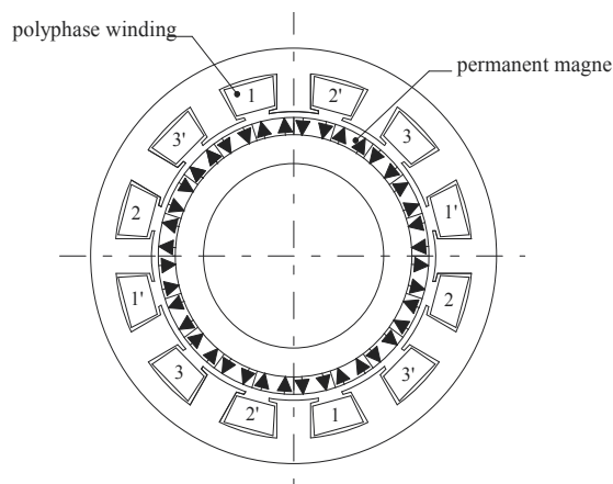
Figure 10. Vernier permanent magnet synchronous generator
