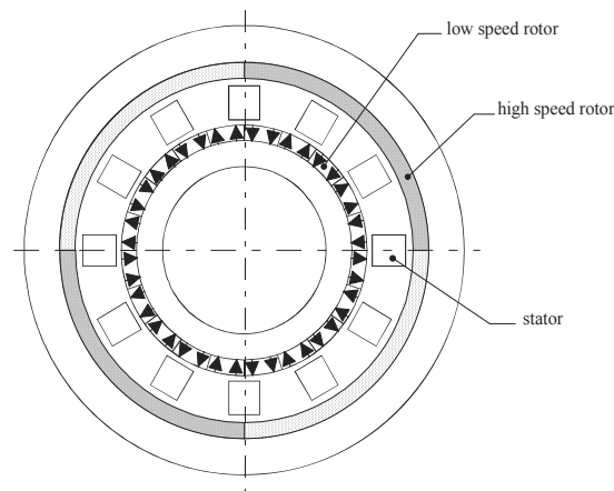
Figure 11. Magnetic speed multiplier with cylinder design
