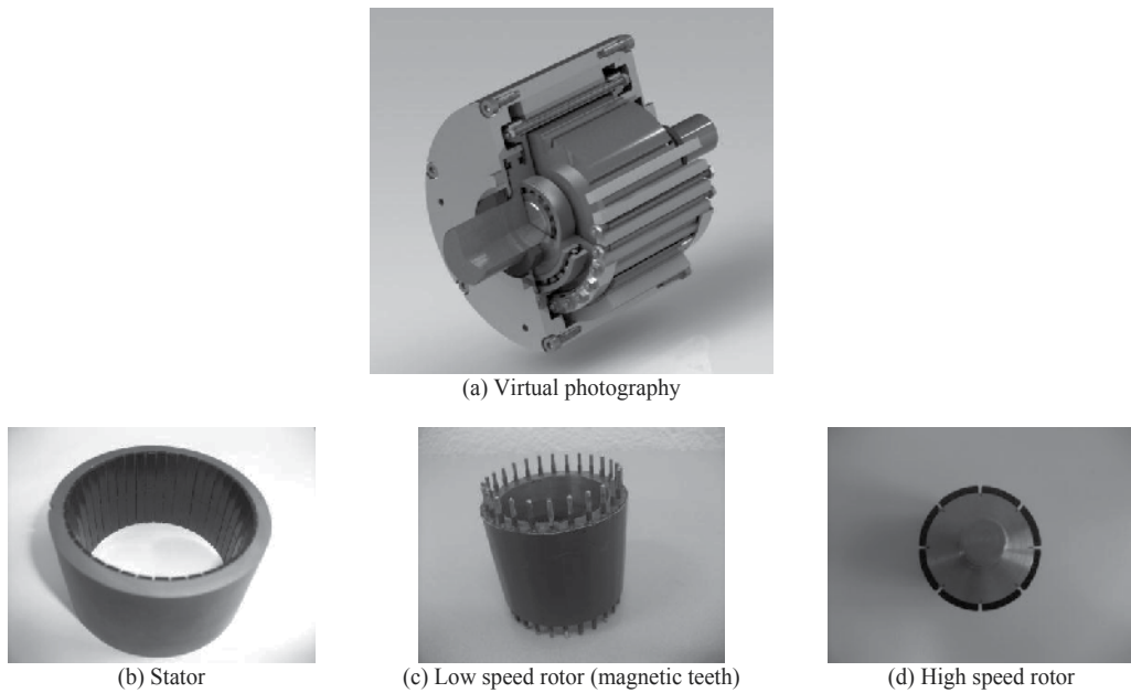
Figure 13. Prototype of a magnetic gear
