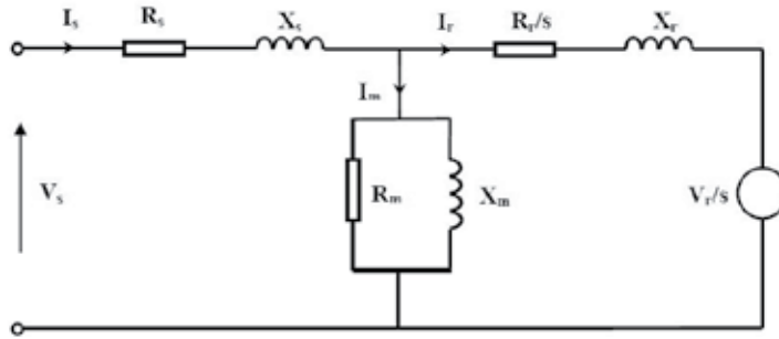
Figure 13. Per-phase equivalent circuit of the DFIG.
