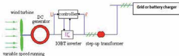
Figure 6. Schematic of a DC generator system [33].
