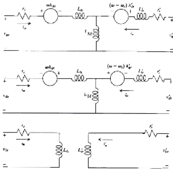
Figure 43. Induction machine Model in dqo system
