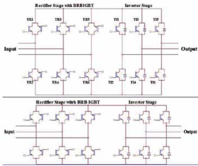
Figure 2. Alternative implementation of the backward VSMC using BRB-IGBT devices.
