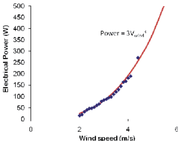
Figure 13. Electrical power versus wind speed at 9 degree attack angle with 6 ohm load
