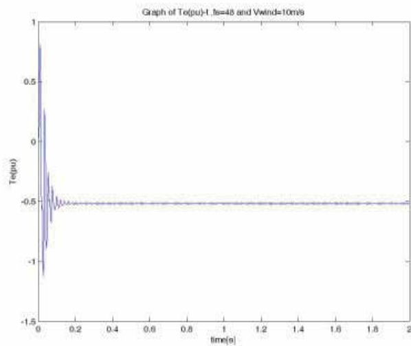
Figure 10. Electrical torque when f_s=48 and u_w=10m/s .
