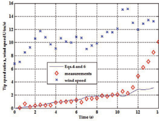
Figure 4. Measured starting sequence of a 5.0 kW two bladed wind turbine which corresponds to the starting torque of Figure 2.
