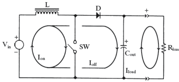
Figure 6. Basic circuit of a boost switching regulator
