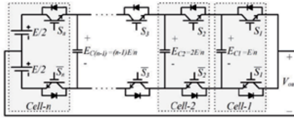
Figure 18. The n cells ( n + 1 levels) FCM inverter.
