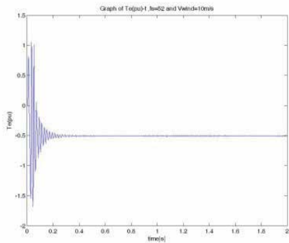
Figure 12. Electrical torque when f_s = 52 and u_w = 10\text{m/s} .
