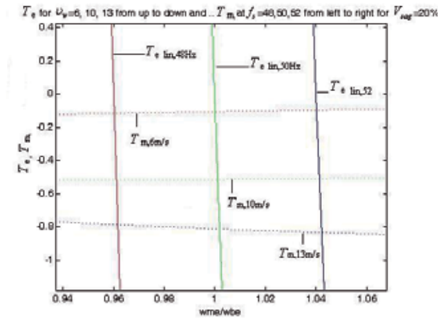
Figure 5. Mechanical and electrical torque versus frequency per unit with V_{\text{sag}} = 20\% .
