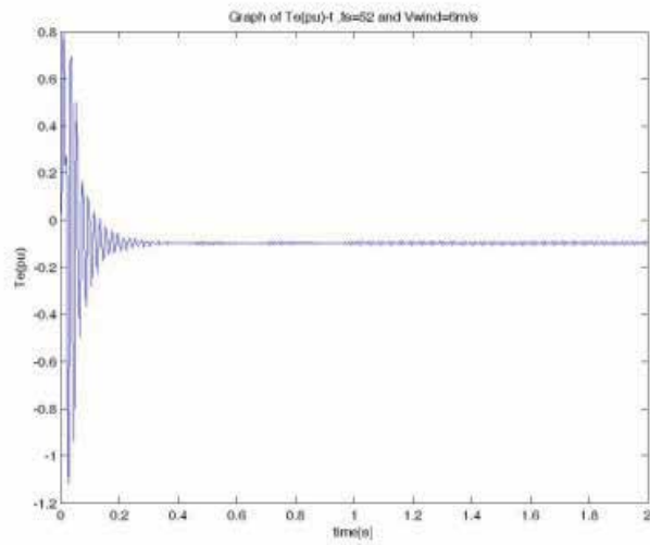
Figure 9. Electrical torque when f_s=52 and u_w=6m/s .
