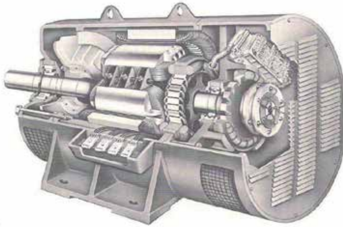
Figure 7. Cutaway of a synchronous generator [22].
