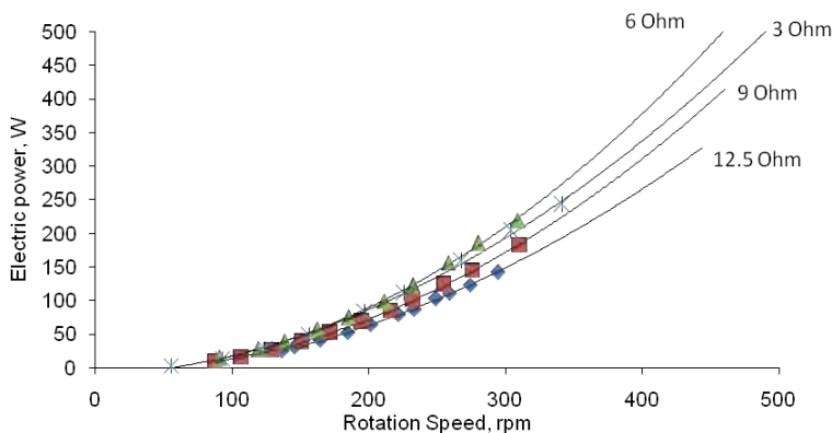
Figure 9. Power versus rotational speed for various loads
