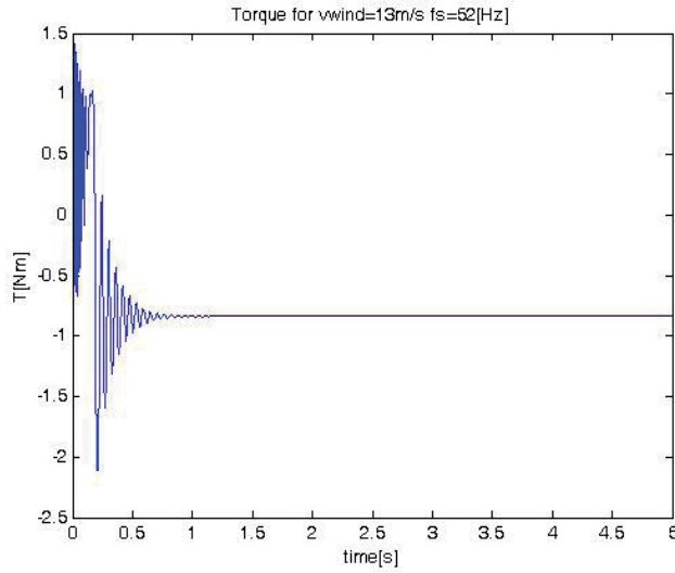
Figure 15. Electrical torque when f_s = 52 and u_w = 13 m/s.
