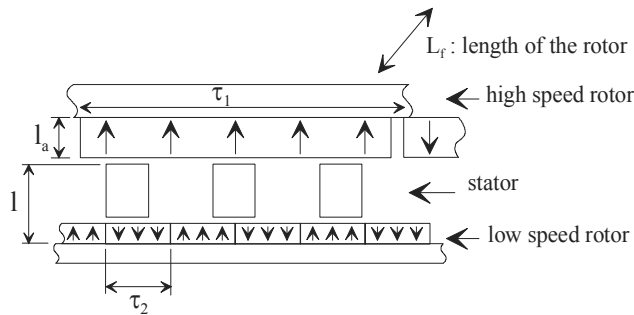
Figure 6. Position at maximum force
