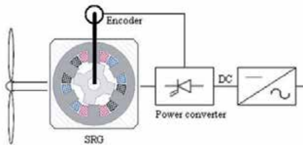
Figure 14. Schematic of a switched reluctance generator system [12].
