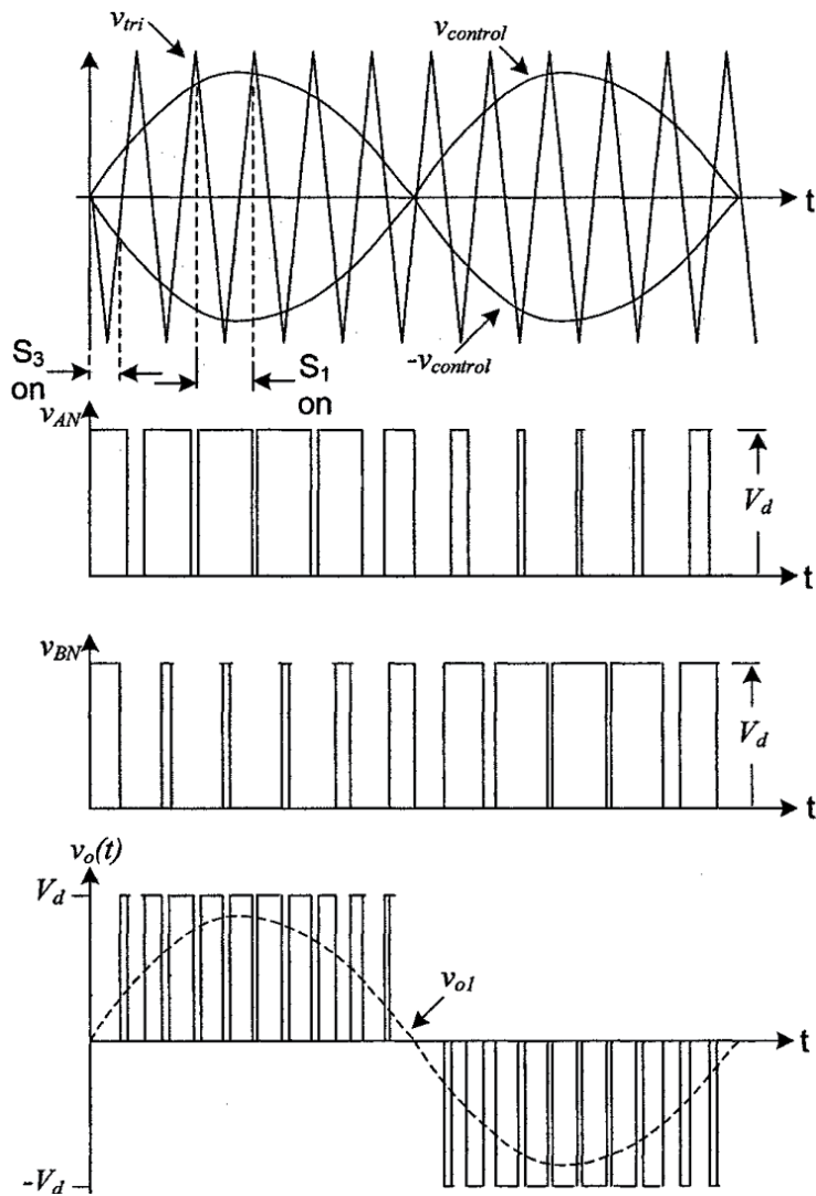
Figure 14. Bidirectional SPWM.
