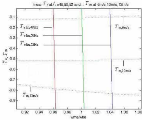
Figure 3. Mechanical and linear electrical torque versus slip.
