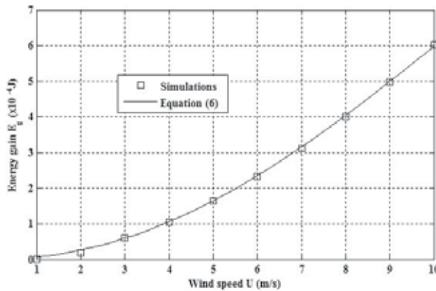
Figure 13. Energy gain by motor-starting to \lambda_{opt} .
