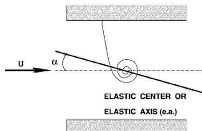
Figure 10. Simplified aeroelastic model to illustrate divergence phenomenon
