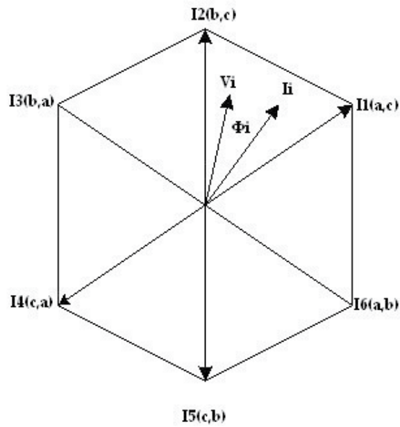
Figure 6. Rectifier stage space vector diagram
