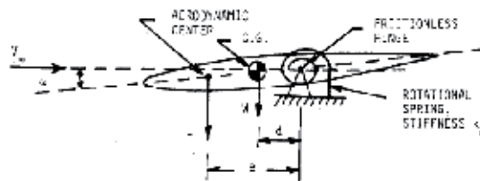
Figure 2. Airfoil model to illustrate aerodynamic flutter
