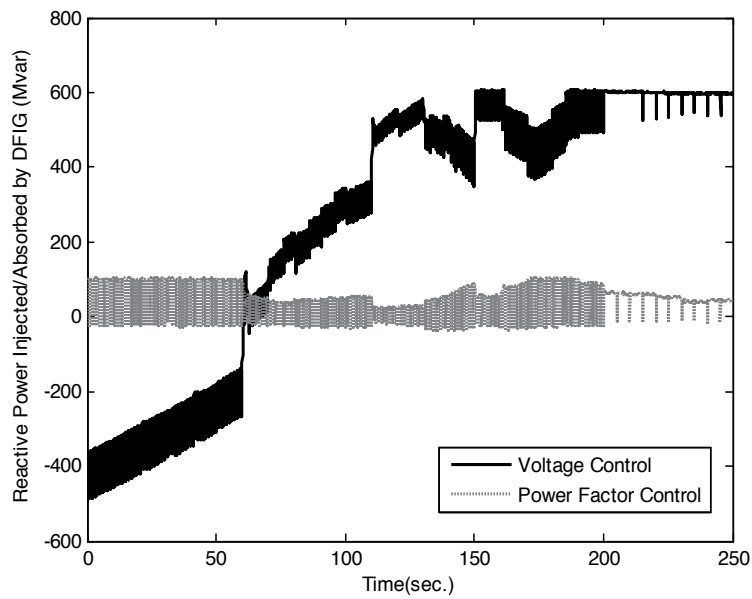
Figure 9. Reactive power injected / absorbed by DFIG.
