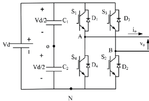
Figure 13. Single-phase full bridge inverter
