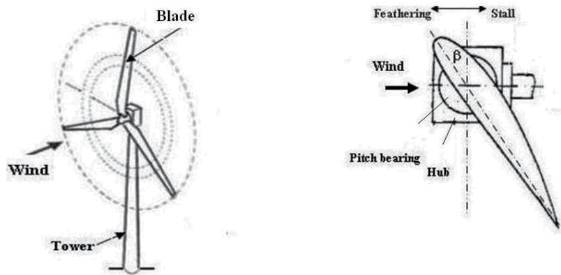
Figure 1. Limiting power output using pitch control.
