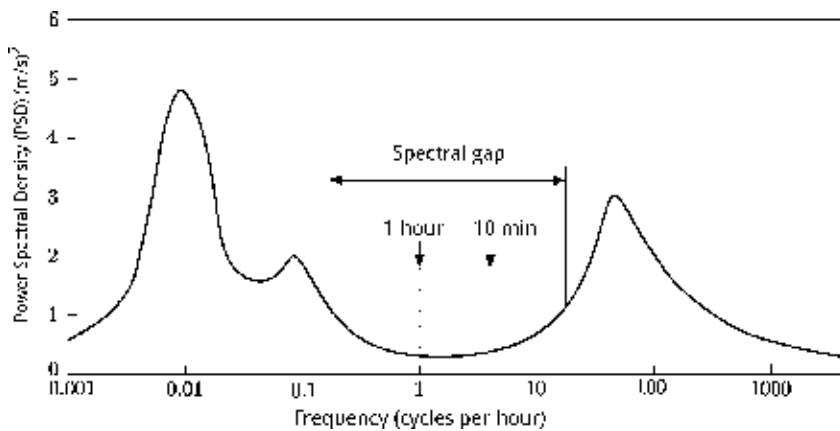
Figure 3. Spectrum estimated by Van der Hoven [4]
