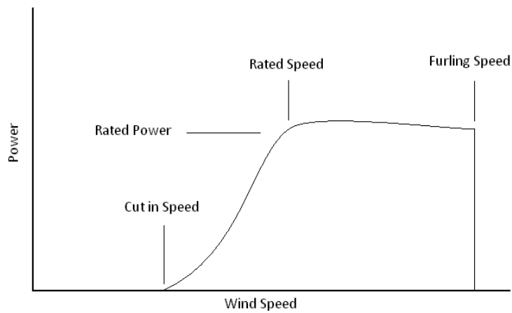
Figure 4. Turbine power versus wind speed.
