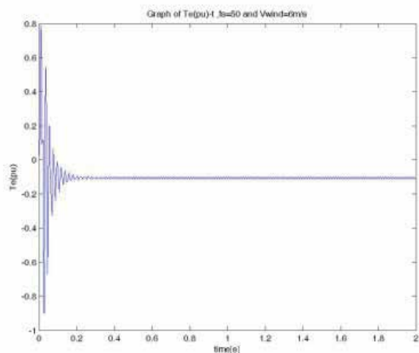
Figure 8. Electrical torque when f_s = 50 and v_w = 6 m/s.
