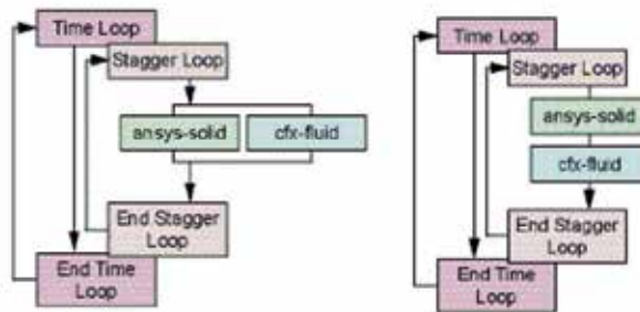
Figure 23. Simultaneous or sequential resolution of CFX and ANSYS
