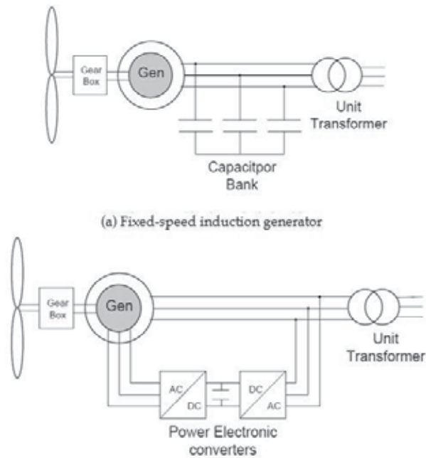
Figure 12. Schematic of two induction generator systems.
