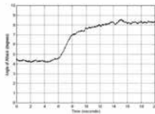
Figure 25. Divergence of wind tunnel model configuration #2
