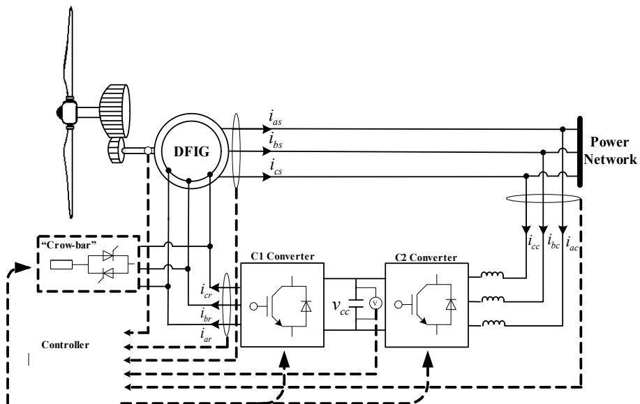
Figure 1. DFIGs Scheme
