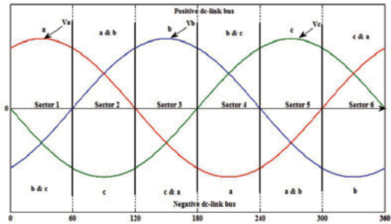
Figure 5. Modulation strategy of the rectifier stage.
