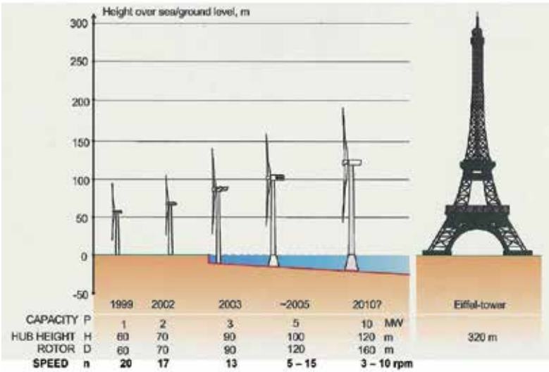
Figure 1. Ever-growing size of horizontal-axis wind turbines [36].
