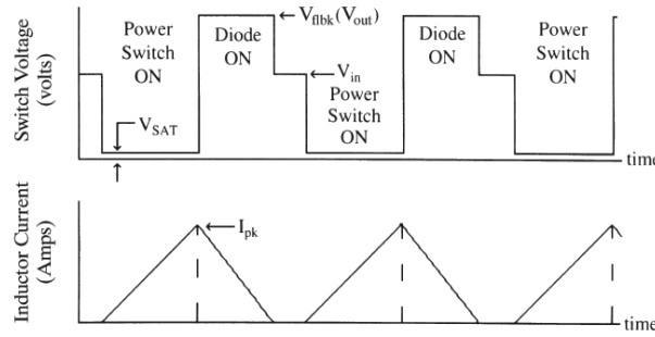
Figure 7. Waveforms for a discontinuous-mode boost converter.
