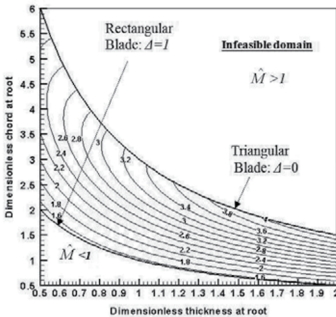
Figure 7. Augmented frequency-mass contours ( \hat{\omega}_1 ) for a blade with flexible blade root: \hat{K}_s = 10 ( \hat{M} = 1 )
