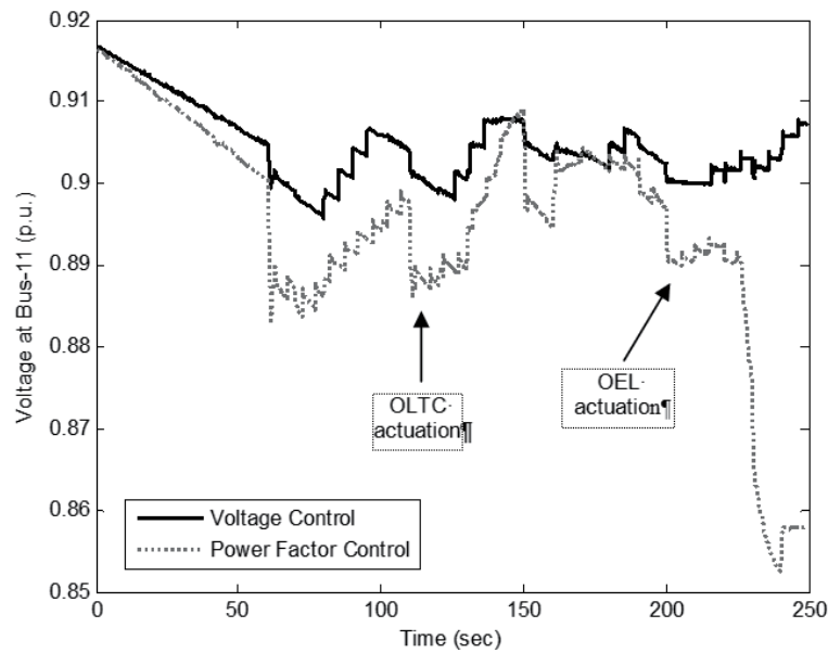
Figure 13. Voltage at Bus 11.
