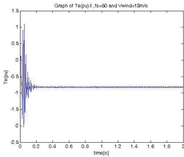
Figure 14. Electrical torque when f_s = 50 and u_w = 13\text{m/s} .
