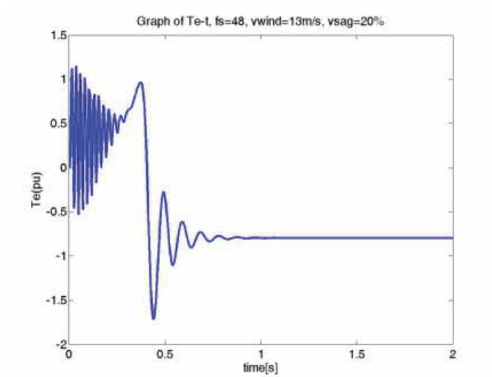
Figure 21. Torque-time in per unit while V_{sag}=20\% and u_w=13\text{m/s} , f_s=48
