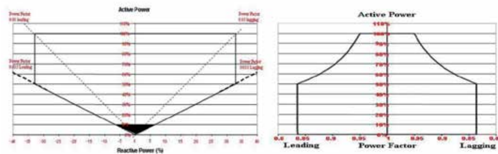
Figure 10. Requirements for reactive power capability of wind plants - Irish code [26].
