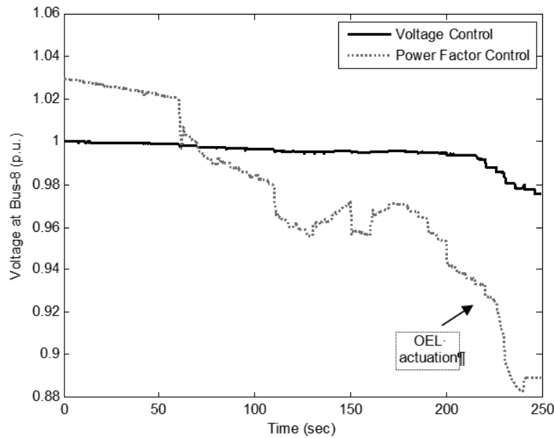
Figure 14. Voltage at Bus 8.
