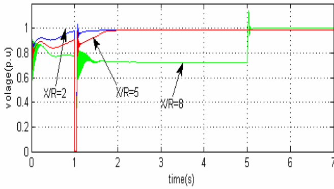
Fig. 11. Terminal voltage variation following a three phase fault for different A=1/SCR_{WF}
