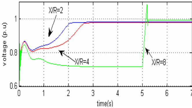
Fig. 8. Effect of different X/R values on the terminal voltage of the induction generator
