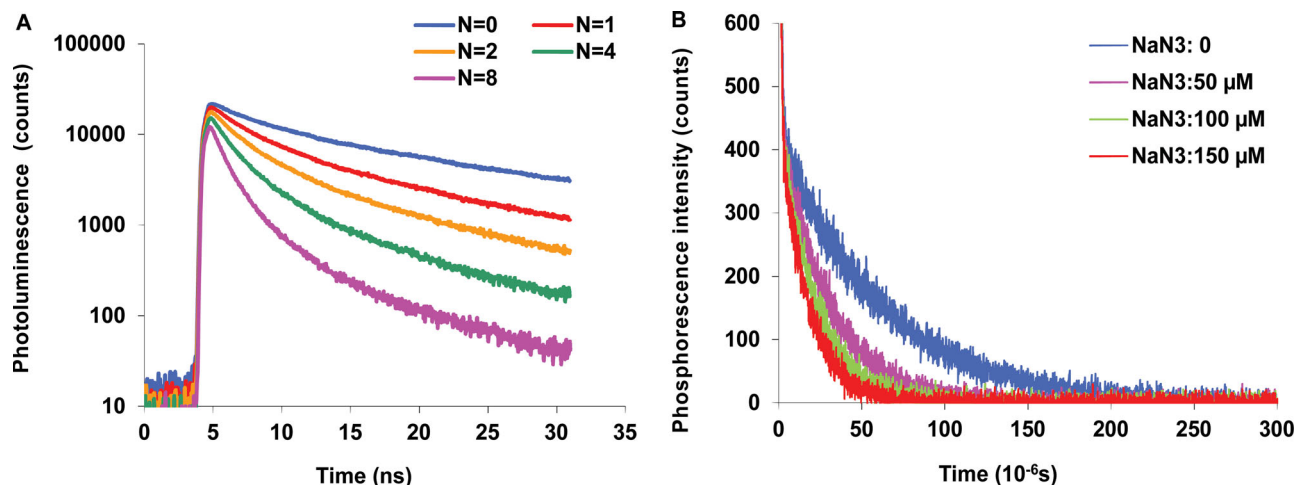
Figure 1. (A) Logarithmic plots of time-resolved QD PL decays of Tat-QD-AlPcS 2a complexes, measured using time-correlated single photon counting with excitation at 405 nm. The molar ratio of AlPcS 2a /QD varies from N = 0 to 8 with a QD concentration of 100 nM; (B) Time-resolved singlet oxygen phosphorescence decays for air-saturated deuterated solutions of Tat-QD-AlPcS 2a complexes (molar ratio of AlPcS 2a /QD of 8, QDs at 100 nM) at increasing NaN 3 concentrations (0–150 \mu M).
