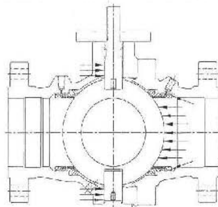
TRUNNION BALL VALVE
