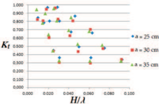
Figure 9. The relationship between wave steepness and transmission coefficient at different water depths.
