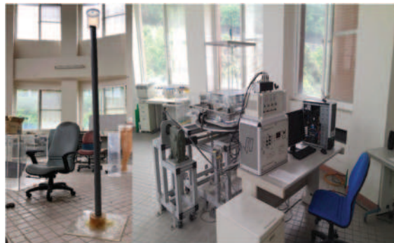
Figure 6. The simple experimental set up of OWT with a tuned liquid damper (TLD) on top.
