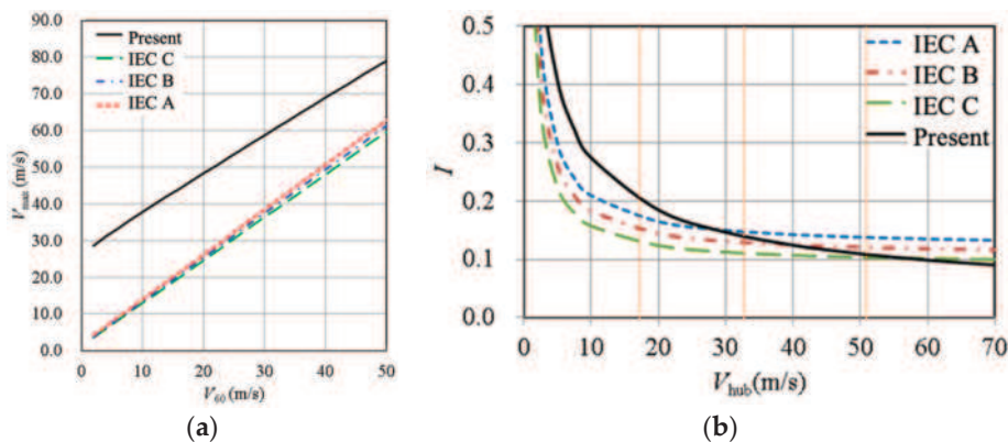
Figure 7. Wind condition comparison between local statistics and design standard. (a) Gust factor; (b) turbulence intensity.
