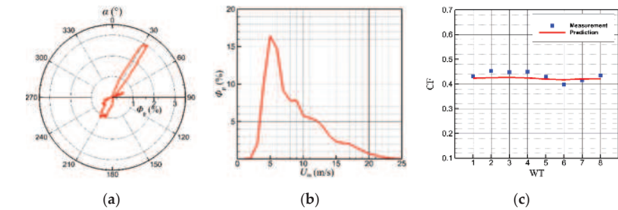
Figure 19. Wind farm A: (a) wind direction probability; (b) wind velocity probability; (c) yearly capacity factor.
