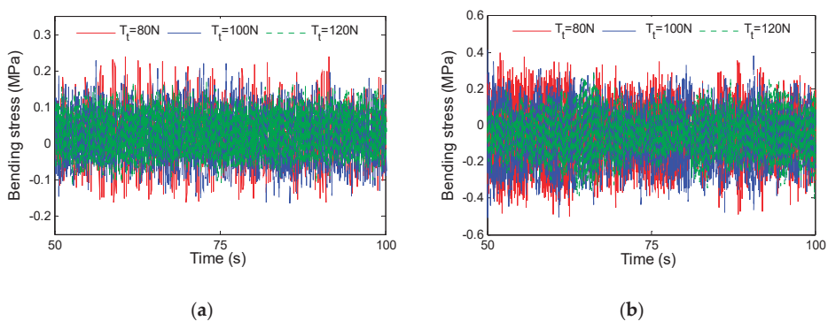
Figure 13. Bending stress time history of TTR at midpoint. (a) U = 0.3\text{ m/s} . (b) U = 0.5\text{ m/s} .
