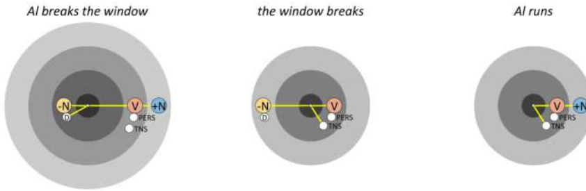
Figure 4.26: Orbital schemas for representing e and \phi -configurations.
