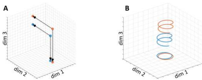
Figure 8.4: Projections of states/trajectories from higher-dimensional spaces to lower-dimensional spaces.
