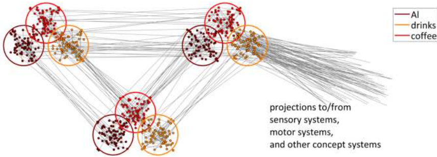
Figure 2.2: Conceptual systems as distributed populations of neurons. Conceptual systems differ in their projections to and from sensory systems, motor systems, and other systems.
