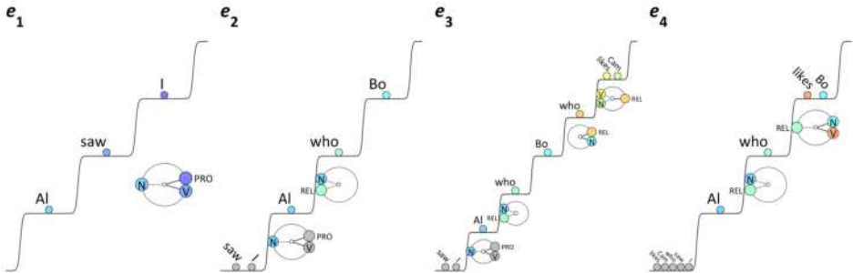
Figure 6.13: Interpretation trajectory for a center-embedded relative clause.
