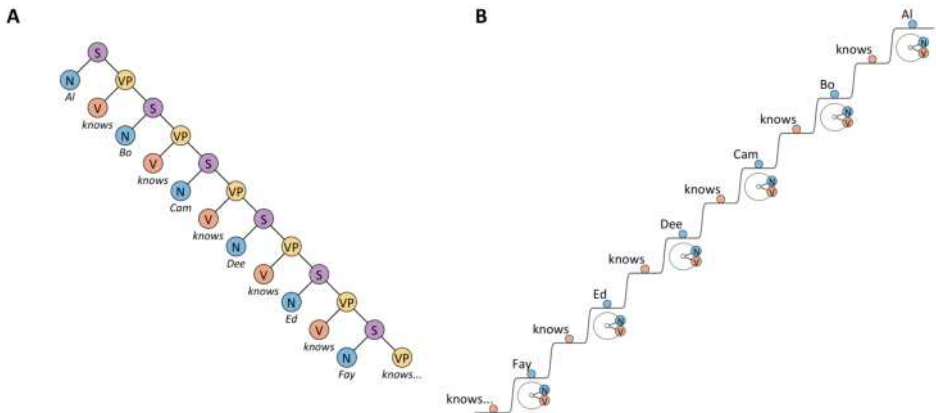
Figure 5.1: Simultaneous presence of syntactic objects.
