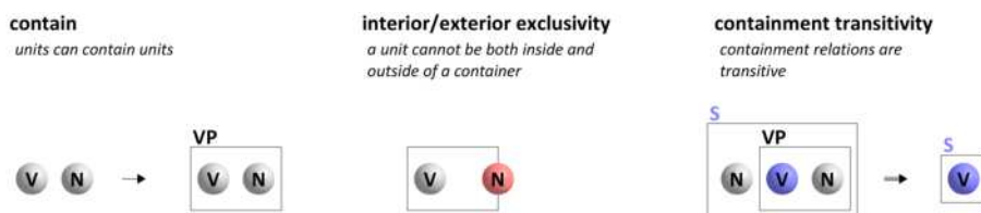
Figure 3.4: Mappings of container schemas: containers can be contained, interior/exterior exclusivity, and transitivity of containment.
