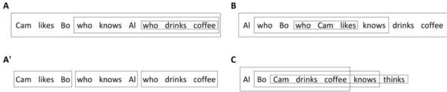
Figure 5.14: Containment schemas for recursive sentences.
