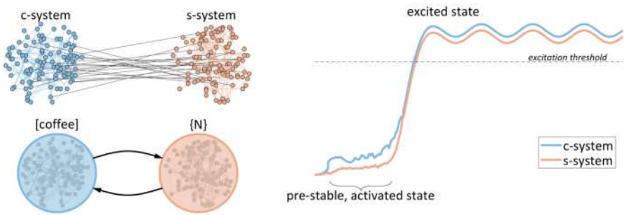
Figure 2.10: Resonance between an s-system and a c-system results in both systems transitioning to an excited state.
