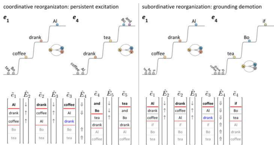
Figure 7.2: Coordinative reorganization vs. subordinative reorganization.
