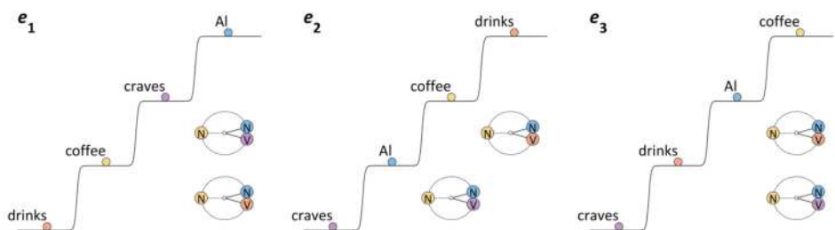
Figure 4.10: Noncanonical reorganization as a mechanism of disfluency.
