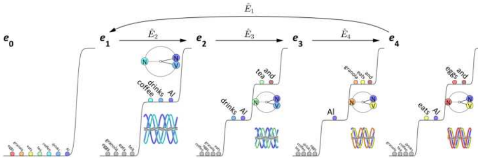
Figure 6.4: Reiterative trajectory involving four \phi -configurations.
