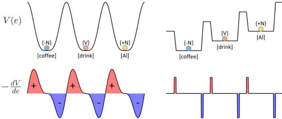
Figure 2.17: Alternative representations of the excitation potential.
