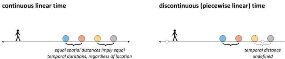
Figure 3.21: Comparison of continuous and discontinuous time schemas. Some temporal distances between events are undefined in discontinuous time.
