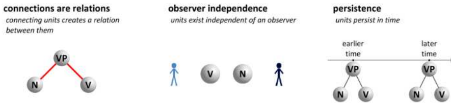
Figure 3.3: Mappings of the object metaphor: connections are relations, observer-independence, temporal persistence.
