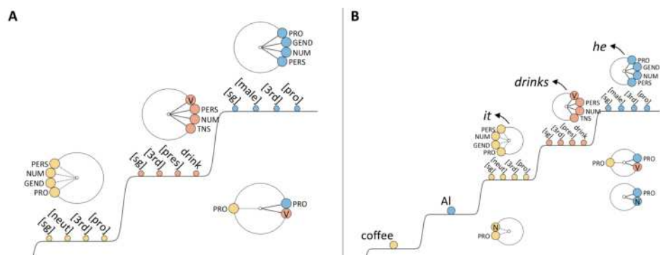
Figure 7.8: Pronominal systems are coupled to lexical systems.
