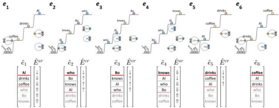
Figure 4.53: Selective reorganization for a subject relative clause.
