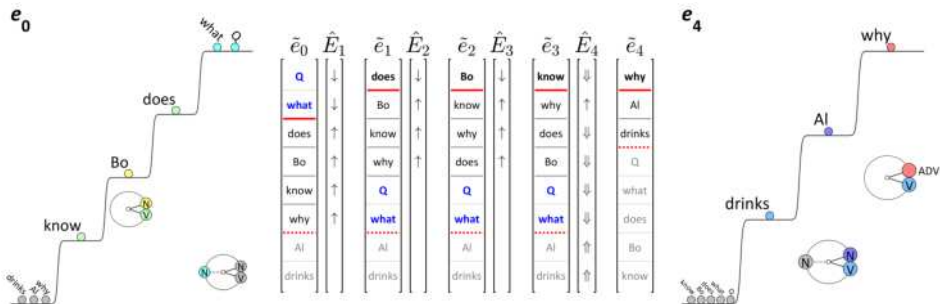
Figure 7.20: Adverbial and relative clauses are strongly grounding and give rise to island effects.
