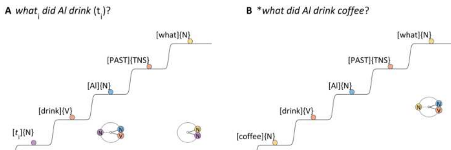
Figure 7.17: Movement/trace analyses of questions are problematic.
