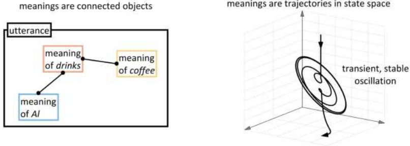
Figure 2.6: The conventional metaphor in which meanings are connected objects vs. an alternative metaphor in which meanings are trajectories in a state space.
