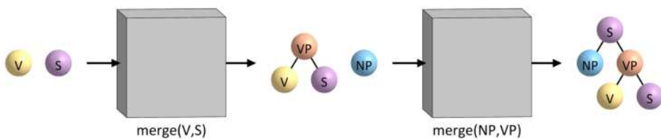
Figure 5.4: Merge and the object-transformation schema.
