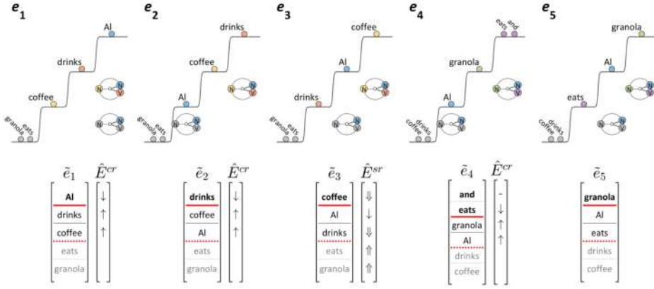
Figure 4.50: Selective reorganization of coordinated verb phrases.
