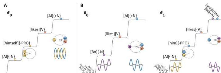
Figure 7.12: Reflexives are associated with destructive c-differentiation interference.
