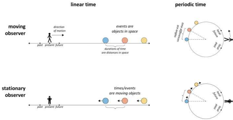
Figure 3.10: Linear and periodic schemas for conceptualizing time.
