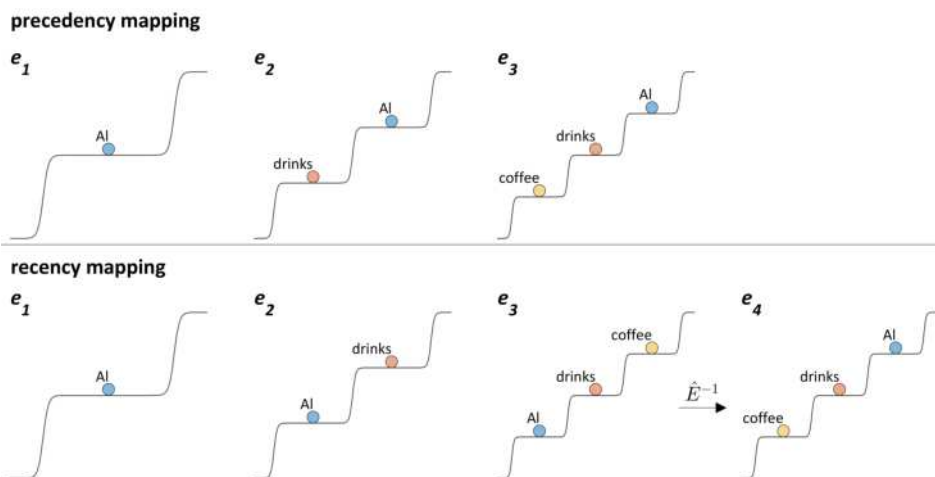
Figure 6.9: Comparison of recency and precedence mappings in the e-organization of perceptually activated systems.
