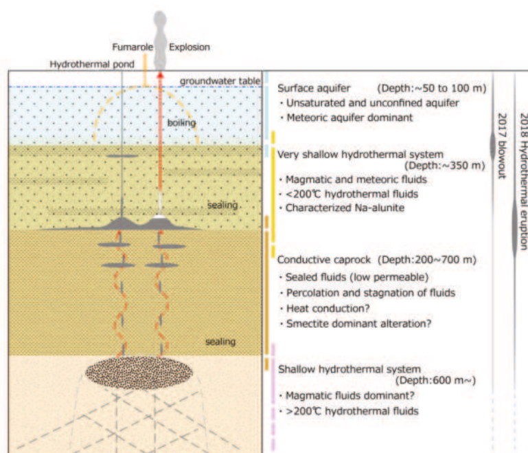
Figure 11. The schematic image of the shallow (ca. 600 m) and very shallow (ca. 350 m) systems beneath Ebino-Ioyama Volcano (See more details in Sections 6.1 and 6.2).
