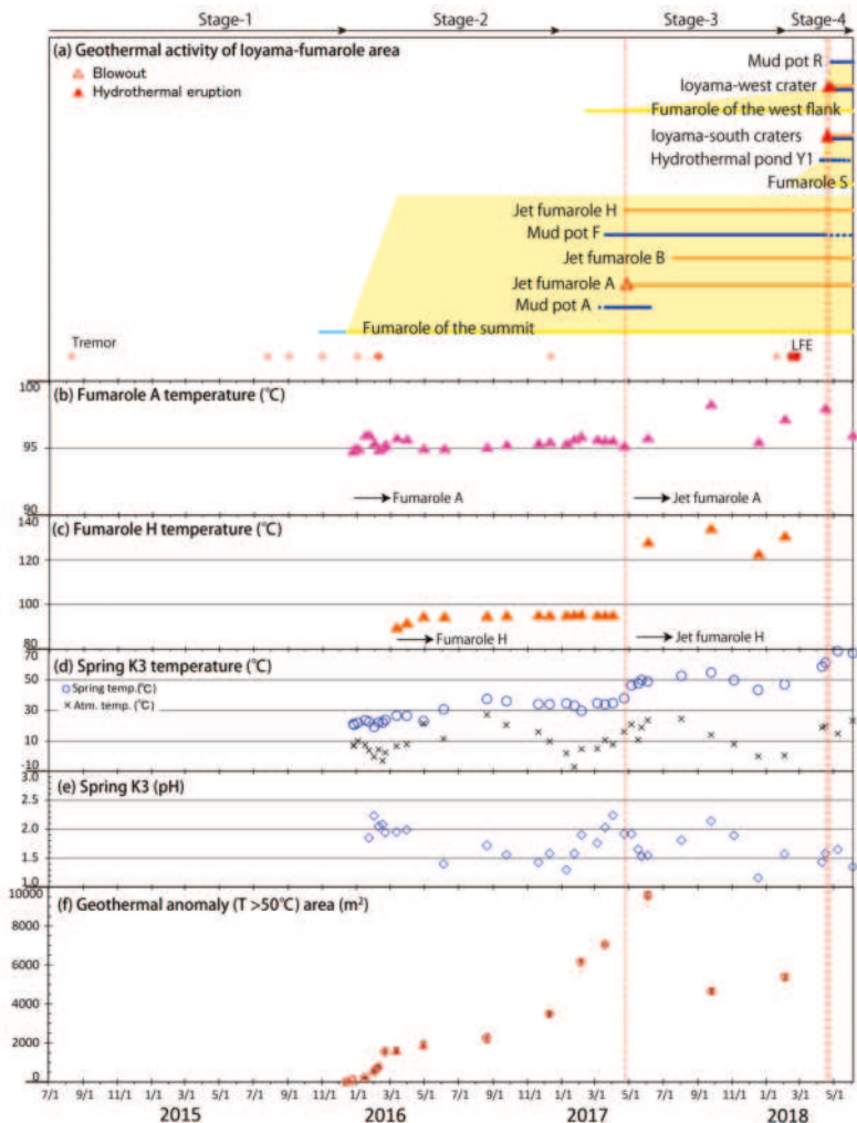
Figure 4. The sequence of geothermal activities at Ebinokogen Ioyama Volcano from July 2014 to June 2018. Geothermal locations are shown in Figure 3. (a) Yellow areas and bars denote the activity of Ioyama-fumarole area. Light blue line indicates a sulfur smell. Orange line denotes a jet fumarole. Blue line denotes a mud pot or hydrothermal pond. Tremor and low-frequency earthquake (LFE) based on the Japan Meteorological Agency (JMA) web site [50]; (b) Temperature observed at point A, before turning into a jet and the jet fumarole A; (c) Temperature observed at point H, before turning into a jet and the jet fumarole H; (d) Water temperature observed at the spring K3; (e) pH of water observed at the spring K3; (f) Geothermal anomaly (>50 °C) area in the summit of Ioyama. Triangles include larger error values.
