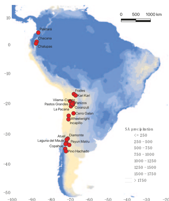
Figure 5. Locations of major late Cenozoic calderas (generally >10 km in diameter) in the Andes, from [51,52]. Map shows mean annual rainfall in mm from 190–2000, from worldclim.org. Calderas are dominantly found in the arid to hyperarid parts of the range.
