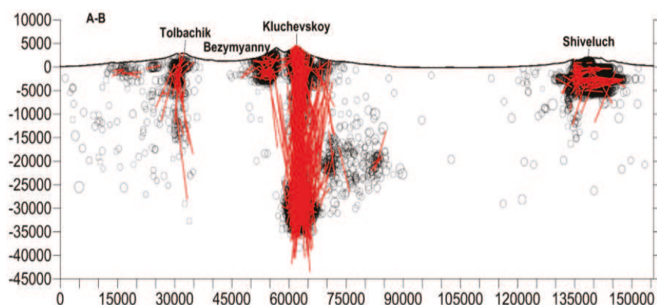
Figure 5. Magma fracturing system beneath the Northern group of volcanoes. The AB cross-section line was shown in Figure 1.
