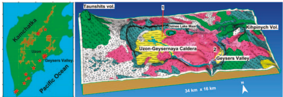
Figure 1. Kamchatka high temperature geothermal systems (left) and schematic 3D view of the Uzon–Geyser–naya caldera (right). The geological units are shown by the colors: alluvial and glacial deposits (light gray), caldera lake deposits ( Q_3^4 ) (yellow), rhyolite–dacite extrusions ( \xi Q_3^4 and \alpha \xi Q_3^4 ) (pink), pre-caldera tuffs and sedimentary deposits (gray), and basalt–andesite lavas (green) ( \alpha Q_3^{1-2} , \alpha Q_3^3 , and Q_3^3 ust). Geysers under monitoring: 1—Shaman geyser area, 2—Bolshoy, Velikan geysers area.
