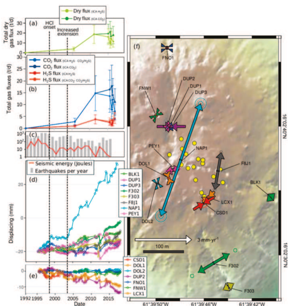
Figure 6. Compared temporal variations of fumarolic gas fluxes, seismicity and dome's fault extensometry at La Soufrière between 1992 and 2017. (a) Total dry gas flux and (b) \text{H}_2\text{S} and \text{CO}_2 fluxes calculated from both \text{H}_2\text{S} and \text{CO}_2 ICAs (for 2006 and 2012 we used only \text{H}_2\text{S} ICA-derived values). (c) Seismicity and (d,e) extent of opening or closing of fractures cross-cutting La soufrière summit dome revealed by extensometric survey. (f) Vectors and amplitudes of fracture width variations and location of active fumaroles (yellow circles) shown in Figure 1. BLK1: Gouffre Breislack, DOL1: Fracture Dolomieu Est, DOL2: Fracture Dolomieu Ouest, DUP1: Gouffre Dupuy Ouest, DUP2: Gouffre Dupuy Est, F302: Faille du Nord-Ouest, F303: Faille 30 Août Bas, F8J1: Faille 8 Juillet 1976, FNO1: Fente du Nord, FNW1: Faille du Nord-Ouest, LCX1: Fracture Lacroix, NAP1: Cratère Napoléon, PEY1: Gouffre Peyssonnel ([28,30], and this work).
