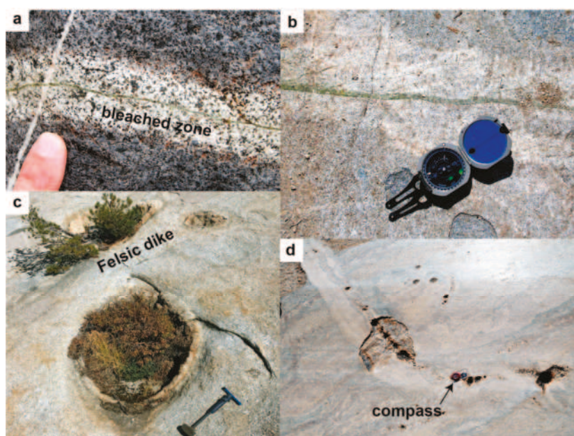
Figure 4. Field evidence of focused fluid transport in granitic plutons. (a) Fracture filled with hydrothermal epidote; diorite near Mack Lake, Sierra Nevada, California, USA. Note bleached zone around the vein. (b) Epidote-filled fracture network and surrounding bleached zone, Piute Creek, Sierra Nevada, California. (c) Pits weathered into large hydrothermal pipes, in and adjacent to felsic dike, Yosemite National Park, USA. (d) Line of pits weathered into hydrothermal pipes along contact of felsic dike, Yosemite National Park, USA (compass with 5 cm ring indicates scale).
