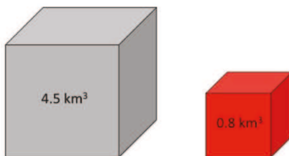
Figure 10. The volume of rock (gray) or magma (red) required to release 10^9 GJ of thermal energy during cooling of \Delta T = 100^\circ\text{C} . For the magma, the temperature drop is chosen to be liquidus to solidus, thereby releasing all the latent heat of crystallization. For the rock, where the energy content is entirely sensible heat, only the size of the temperature interval is important.
