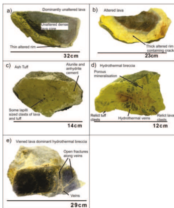
Figure 2. Photographs showing examples of collected ballistic samples from the 2016 eruption at Whakaari cut in two to reveal interior, (a) Unaltered lava, (b) altered lava, (c) Ash Tuff, (d) Hydrothermal breccia, (e) hydrothermal breccia of altered and unaltered lava.
