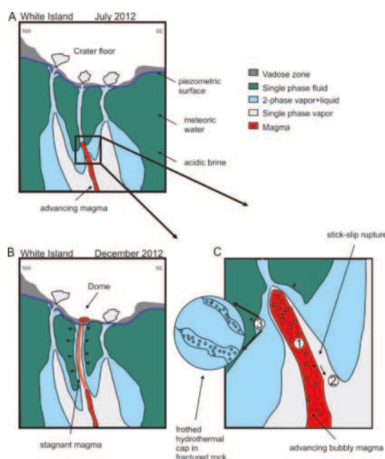
Figure 2. Schematic cross section depicting (A) the pre- and (B) post-extrusion scenarios for the dome. Acidic brine fluids underlie meteoric water/condensate lenses (both depicted green) and encapsulate the magmatic/fumarolic vent system (blue and grey). Magma ascends along the main conduit (designated by the red line in (B), preceded by increased heat and gas flow which evaporates the two-phase vapour-liquid region to single-phase vapor along its way (grey). Three possible resonant systems are portrayed in the inset diagram (C). The bubble filled cavity (1). A clockwork stick-slip rupture mechanism (2), or the frothed expanding boiling front (3 and its inset) may produce harmonic signals discussed. The arrows in B show the expanded two-phase system that results from the propagating magma injection. See text.
