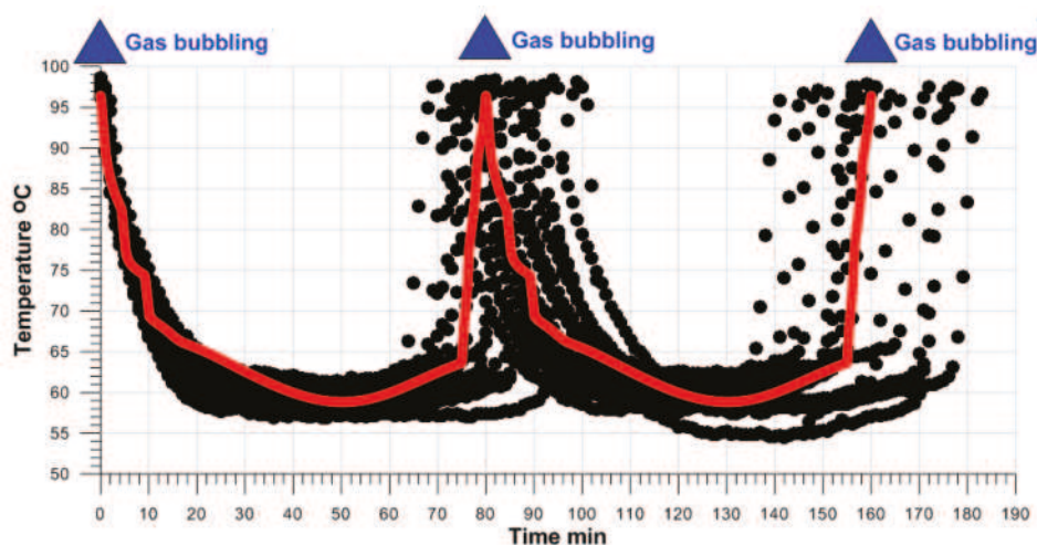
Figure 12. Modeling (run #9A2, unknown parameter estimations were: q = 0.15 \text{ kg/s} , h = 84 \text{ kJ/kg} (water 20^\circ\text{C} ), Q = 2 \text{ kg/s} ) of the transient bottom temperature in the Shaman geyser vs. the bottom temperature records obtained during the time period of observations from 27.06.2019 18:00 to 29.06.2019 18:00 (Figure 5).
