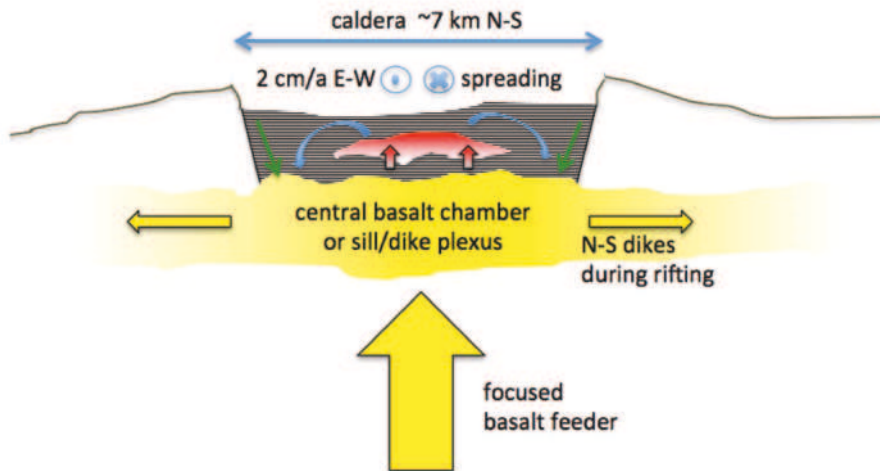
Figure 9. Suggested concept for Krafla shield and caldera. A basaltic magma plume beneath the rift is responsible for building the shield and maintaining a large and relatively shallow basaltic magma chamber. This chamber may be a plexus of dykes and sills rather than an oblate bladder. During rifting events, the magma accumulation feeds dikes that travel tens of kilometers to the north and south, deflating and contributing to caldera subsidence in the process. Central eruptions and intrusions of basalt and more silicic magmas comprise the caldera fill, which is hydrothermally altered in this crucible and gradually fed downward to the basaltic hearth. Partial melting ensues, probably continuously dribbling rhyolitic melt upward to its level of neutral buoyancy at about 2 km depth. If the input is insufficient, only felsite sills are produced, but if more vigorous, a homogeneous convecting rhyolite magma body is established. It is stable for long periods of time, but can be expelled if a massive influx of basaltic magma occurs below it during a major rifting event. Undisturbed, the shallow rhyolite contributes only a portion of the thermal output of the caldera, but it represents a massive concentration of latent heat of crystallization at shallow depth that can be accessed if the MHB above it is penetrated by drilling, allowing fluid to invade and fracture the magma and near-magma region.
