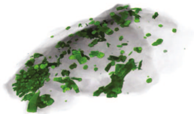
Figure 4. A 3-D perspective by X-ray tomography of a magma chip (2 mm long), from IDDP-1. False-color green crystals, mostly plagioclase, float in transparent gray melt. A clot of crystals at the lower left is partially melted felsite. The chip was quenched at about 2100 m depth and 900 °C. Credit: Sample provided by Landsvirkjun and A. Mortensen; image by F. Wadsworth, Munich U., Germany; E. Saubin, U. of Canterbury and C. I. Schipper, Victoria U., NZ.
