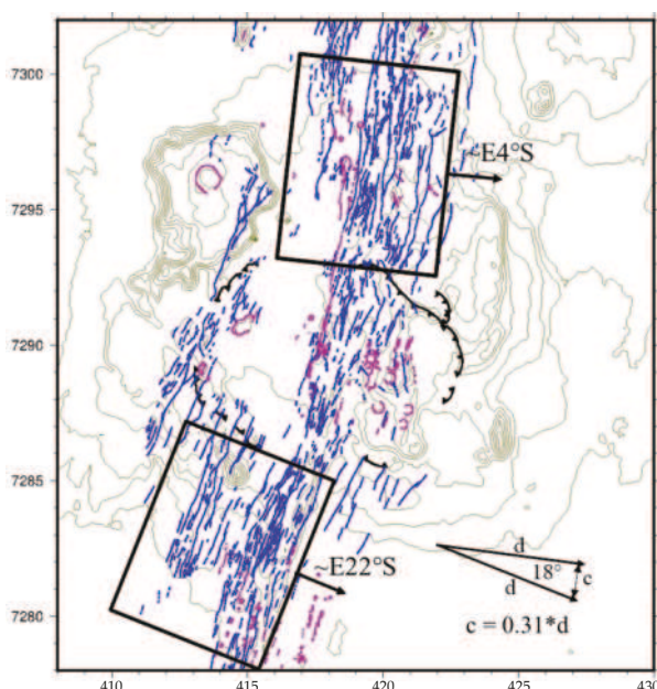
Figure 5. Different crustal spreading directions south and north of the Krafla caldera leading to an opening component in the eastern part. The inset bottom right shows how spreading by, d , leads to opening component, c , in the east. Blue lines represent faults and fissures and purple lines eruptive fissures and craters. Coordinates are UTM WGS84 zone 28 in km.
