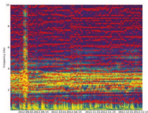
Figure 6. Same as Figure 5, but with potential dominant frequency and corresponding harmonics overlaid (red dots in 4-hr time windows).
