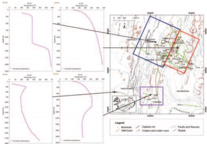
Figure 13. Drilled wells in Krafla (red dot on the little inlet map to the right) and the three main production fields (right) with different thermal character. The fields are: Vtismór and Leribotnar (blue frame), southern and western slopes of Mt. Krafla (red frame) and Hvíthólar (purple frame). To the left are shown characteristic temperature profiles in wells in each production area and a well drilled in the fissure swarm west of Hvíthólar. For well KS-01, east of Hvíthólar, see text.
