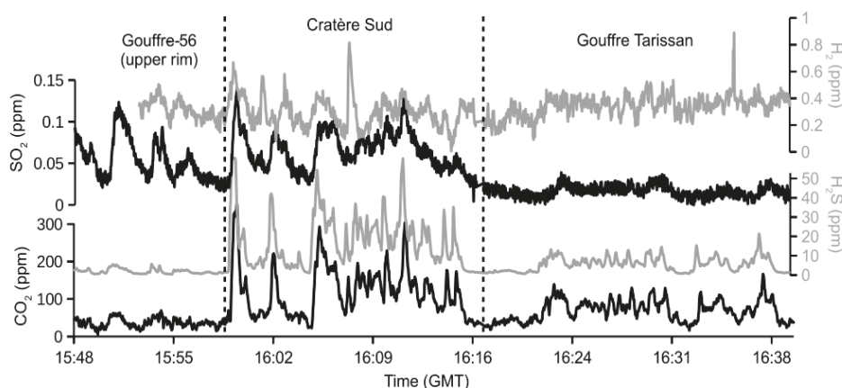
Figure 3. Example of MultiGAS recording of \text{CO}_2 , \text{SO}_2 , \text{H}_2\text{S} and \text{H}_2 co-variations in gas emissions from Gouffre-56 (G56), Cratère Sud (CS) and Gouffre Tarissan (TAS) fumaroles during walking profiles across the plumes in May 2016.
