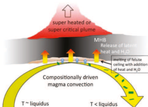
Figure 8. Thermally (density increase due to cooling) and compositionally (density increase due to crystal growth) driven circulation in magma could transfer heat and H 2 O at the lower face of the MHB without coating it with crystals and, in the case of Krafla, partially melting it. This would explain the sparse crystal content of all shallow silicic magmas thus far encountered (Table 1).
