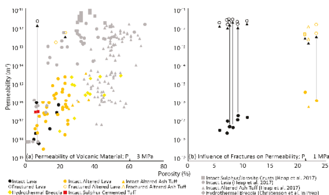
Figure 6. Permeability as a function of porosity at (a) confining pressure 3 MPa (this study) and 1 MPa, and (b) confining pressure 1 MPa showing the wide variability of matrix permeability (solid black points are unaltered intact lava from the edifice; yellow are altered intact ballistic samples collected at 3 MPa confining pressure) and low variability of fracture permeability (open points).
