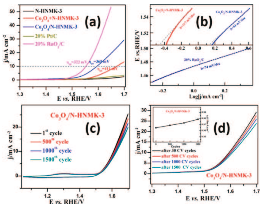
Figure 8. (a) LSV curves of N-HNMK-3, \text{Co}_3\text{O}_4 + \text{N-HNMK-3} (physical mixture), \text{Co}_3\text{O}_4/\text{N-HNMK-3} , 20 wt.% Pt/C, and 20 wt.% \text{RuO}_2/\text{C} towards the OER in \text{O}_2 -saturated 1.0 M KOH at 5 \text{ mV s}^{-1} and 1600 rpm; (b) Tafel plots of each samples derived from curves in (a); (c) CVs of \text{Co}_3\text{O}_4/\text{N-HNMK-3} from 1.05 V to 1.70 V at 200 \text{ mV s}^{-1} in \text{O}_2 -saturated 1.0 M KOH from 1st cycle to 1500th cycle; (d) LSV curves of \text{Co}_3\text{O}_4/\text{N-HNMK-3} from 1.30 V to 1.70 V at 5 \text{ mV s}^{-1} , the inset presents the variation of \eta_{10} at different CV cycles.
