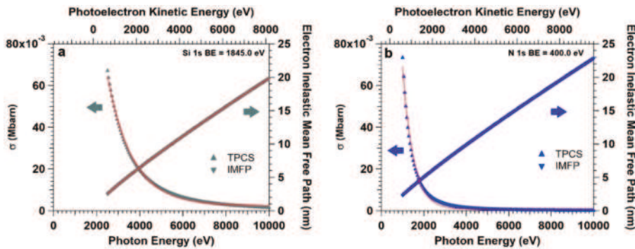
Figure 4. Electron inelastic mean free path (IMFP, right axes) and total photoionization cross section (TPCS, left axes) as a function of the photon energy, for Si 1s (a) and N 1s (b) core levels. The photoelectron kinetic energy scale has been generated from the photon energy values, using Einstein’s energy conservation law and a binding energy of 1845.0 eV and 400.0 eV for Si 1s and N 1s core levels, respectively. The IMFPs are determined for photoelectrons travelling through water. Red curves are fits according to Equations (3) and (4).
