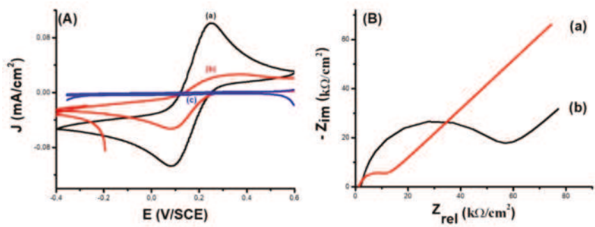
Figure 2. Electrochemical characterization of diazonium-modified ITO electrodes determined in aqueous solutions of 1 mM K 3 Fe(CN) 6 and 0.1 M KCl. (A) Typical cyclic voltammograms (a) bare ITO, (b) ITO-N(CH 3 ) 2 , and (c) ITO-SO 3 H. (B) Electrochemical impedance spectroscopy plots recorded with (a) ITO-N(CH 3 ) 2 , and (b) ITO-SO 3 H.
