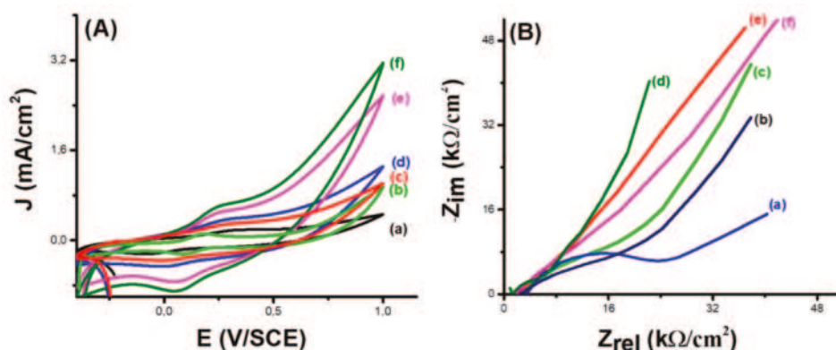
Figure 6. PPy-BSA film on (a) ITO-SO 3 H, (b) ITO-CN, (c) ITO-CO 2 H, (d) ITO-NH-Ph, (e) ITO-NH 2 , (f) ITO-N(CH 3 ) 2 . (A) Blocking effect of the PPy-ABS films on the ITO electrodes modified by the different diazonium cations. (B) Impedance measurements recorded for PPy-ABS coatings on modified ITO sheets.
