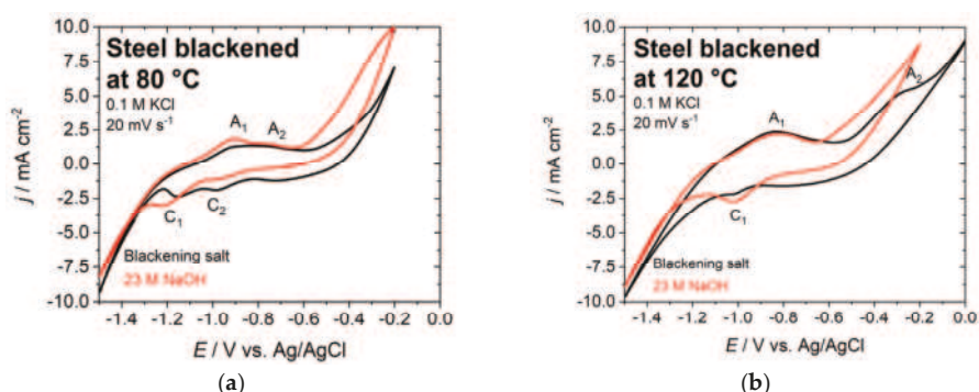
Figure 7. Cyclic voltammogram of blackened steel discs in 0.1 M KCl solution at (a) 80 °C and (b) 120 °C; black curve: blackening salt; red curve: NaOH; scan rate 20 mV s −1 .
