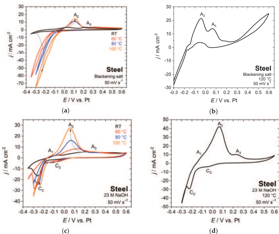
Figure 2. Cyclic voltammograms of steel in blackening salt solution (a) at various temperatures between room temperature and 100 °C, (b) at 120 °C and (c) in 23 M sodium hydroxide solution at various temperatures between room temperature and 100 °C, and (d) at 120 °C; scan rate 50 \text{ mV s}^{-1} .
