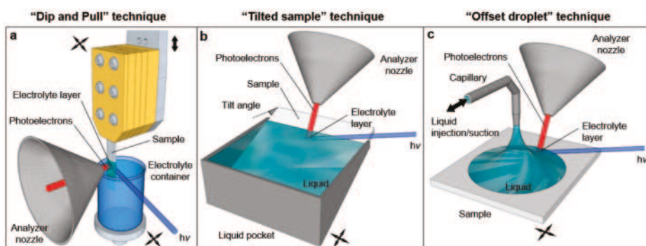
Figure 2. Schematization of the “dip and pull” (a), “tilted sample” (b) and “offset droplet” techniques (c) that are successfully used to prepare free-surface liquid layers thin enough to probe the solid/liquid interface using photoelectron spectroscopy.
