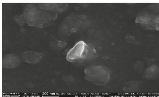
Figure 1. SEM image of nc-Si(1)/poly-3(hexylthiophene) (P3HT) samples.
