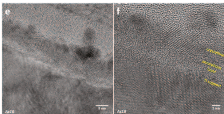
Figure 3. (a–d) Diffraction patterns evaluated from selected area electron diffraction (SAED) patterns (Figure S4) of Ox10 (a and c) and Ac10 films (b and d) before (_AP; a and b) and after electrochemical OER protocol (_OER; c and d). The patterns only show metallic Ir. (e,f) TEM cross-section of Ac10_AP film shows crystalline Ir particles on an amorphous interlayer.
