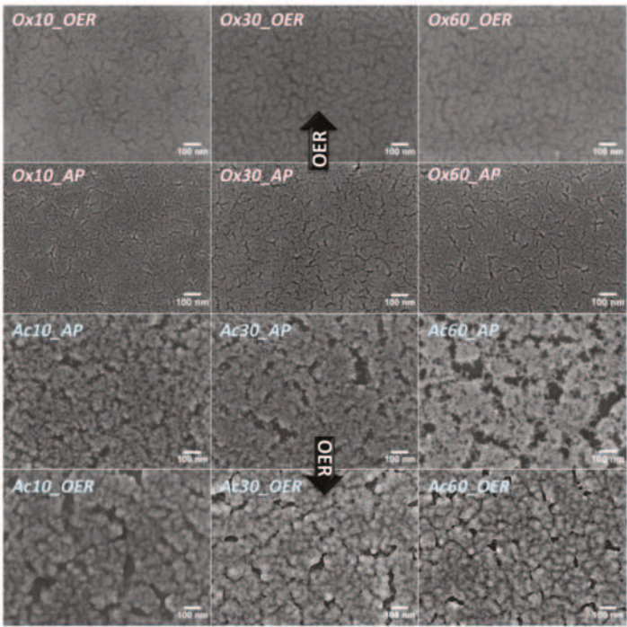
Figure 1. Scanning electron microscopy (SEM) images of Ox (top) and Ac (bottom) film series before (_AP, second and third row) and after oxygen evolution reaction (OER) (_OER, first and fourth row). The cracks in the Ac films enlarge with increasing heating time. The weakly cracked morphology of the Ox films does not show any change depending on the reductive heating time.
