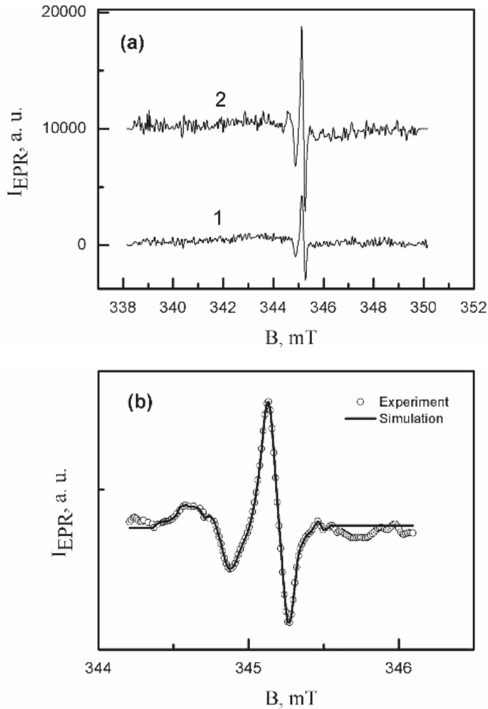
Figure 3. (a) EPR spectra of nc-Si(1)/P3HT samples in the dark (1) and under illumination (2). (b) Experimental and simulated EPR signals of nc-Si(1)/P3HT samples.
