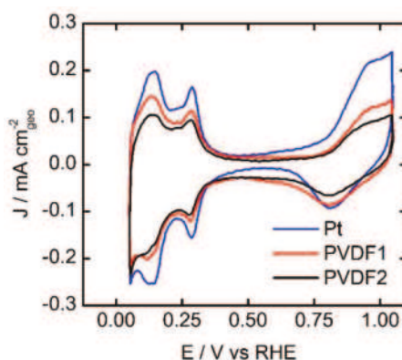
Figure 1. Cyclic voltammograms recorded in Ar saturated 0.05 M H_2SO_4 electrolyte solution for bare and polyvinylidene difluoride (PVDF) modified Pt. The scan rate was 100\text{ mVs}^{-1} and the measurements were recorded at room temperature. PVDF 1 stands for the film prepared by dip coating the Pt electrode into 0.1 mM PVDF solution, PVDF 2 for the film prepared by dip coating into 0.1 M PVDF solution. The roughness factors ( R_f ), calculated by H_{upd} for bare Pt, PVDF1, and PVDF2, are: 1.65, 1.20, 0.94. This corresponds to an ECSA loss with respect to the bare polycrystalline Pt electrode of 27 % and 43 % for PVDF 1 and PVDF 2, respectively.
