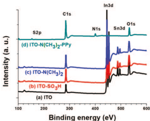
Figure 7. XPS survey regions of (a) ITO, (b) ITO-SO 3 H, (c) ITO-N(CH 3 ) 2 and (d) ITO-N(CH 3 ) 2 -PPy.
