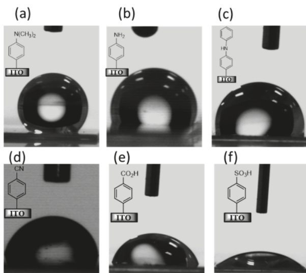
Figure 3. Contact angles of water drops gently deposited on diazonium-modified ITO: (a) ITO- \text{N}(\text{CH}_3)_2 , (b) ITO- \text{NH}_2 , (c) ITO- \text{NH-Ph} , (d) ITO- \text{CN} , (e) ITO- \text{CO}_2\text{H} , (f) ITO- \text{SO}_3\text{H} .
