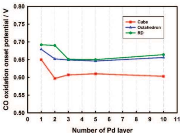
Figure 7. CO oxidation onset potential as a function of the Pd film thickness on different Au nanocrystals in 0.1 M \text{HClO}_4 .
