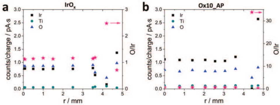
Figure 2. Counts per charge of the three main elements detected in energy-dispersive X-ray spectroscopy measurements (EDX) of (a) IrO x and (b) Ox10_AP. The different intensities are caused by different film thicknesses, mainly due to border effects during spin coating.
