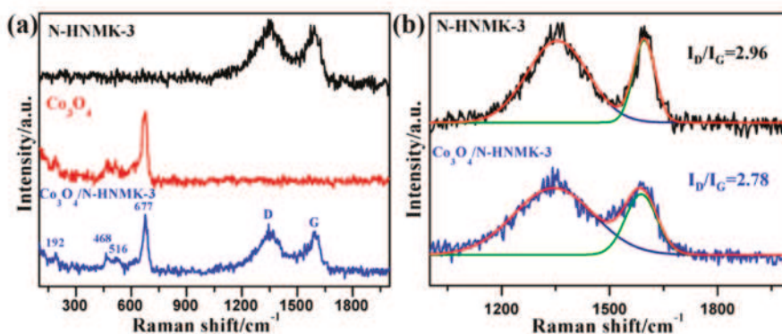
Figure 4. (a) Raman spectra of N-HNMK-3, \text{Co}_3\text{O}_4 and \text{Co}_3\text{O}_4/\text{N-HNMK-3} . (b) The corresponding Raman fitting profiles of N-HNMK-3 and \text{Co}_3\text{O}_4/\text{N-HNMK-3} .
