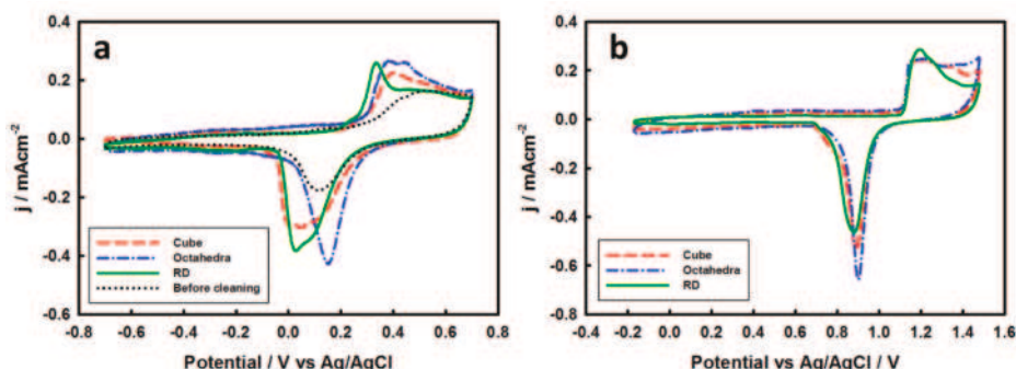
Figure 3. Cyclic voltammograms (CVs) of cubic, octahedral, and RD Au nanocrystals in (a) 0.1 M NaOH (b) 0.1 M \text{H}_2\text{SO}_4 . The dotted line in (a) is the CV of cubic Au nanocrystals before the potential cycling process. Scan rate: 0.100 \text{ V s}^{-1} .
