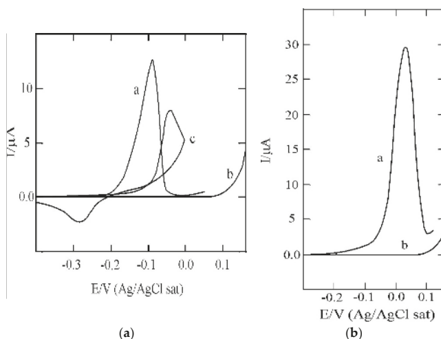
Figure 6. (a) Linear sweep voltammograms for the oxidative strippings of Cd from CdS deposited with 10 ECALE cycles on Ag(III) not covered by thiol (curve a); modified for about 18 h (curve b) and modified for short times (curve c); (b) linear sweep voltammograms for the oxidative strippings of Cd from CdS deposited with 30 ECALE cycles on Ag(III) not covered by thiol (curve a); modified for about 18 h (curve b). The scan rate was 10 mV/s.
