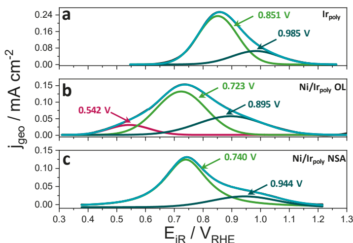
Figure 8. CO stripping curves for (a) the unmodified polycrystalline Ir electrode and the Ni-modified (b) Ir poly OL and (c) Ir poly NSA catalysts obtained at 50 mV s −1 in N 2 -saturated 0.1 M KOH (purified Fe free) at a rotation of 1000 rpm. A linear-background correction was performed through baseline subtraction for the anodic CO stripping voltammetry in Figure 7a between 0.4 and 1.2 V RHE . The peaks were fit by Gaussian functions and the individual contributions are shown in colors. The cumulative curve is given in turquoise.
