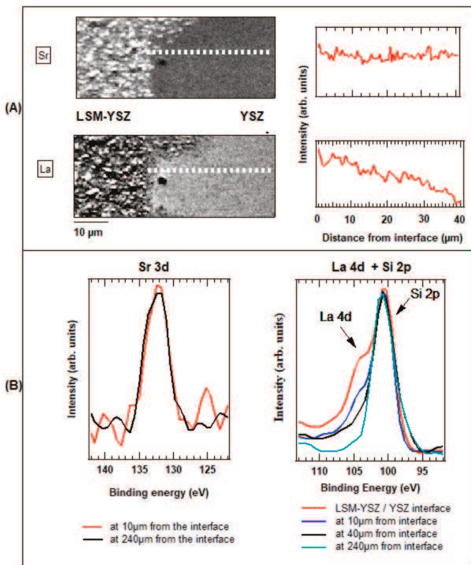
Figure 15. (A) SP-EDS maps at the Sr 3d and La 4d energies and elemental concentration profiles, recorded with a pristine cell in 0.05 mbar of O 2 at 924 K. The imaged region is the interface between the LSM-YSZ cathode (left) and the YSZ electrolyte (right). (B) Sr 3d and La 4d \mu XPS spectra measured at the indicated distances from the cathode/electrolyte interface along the dotted line shown in Panel (A).
