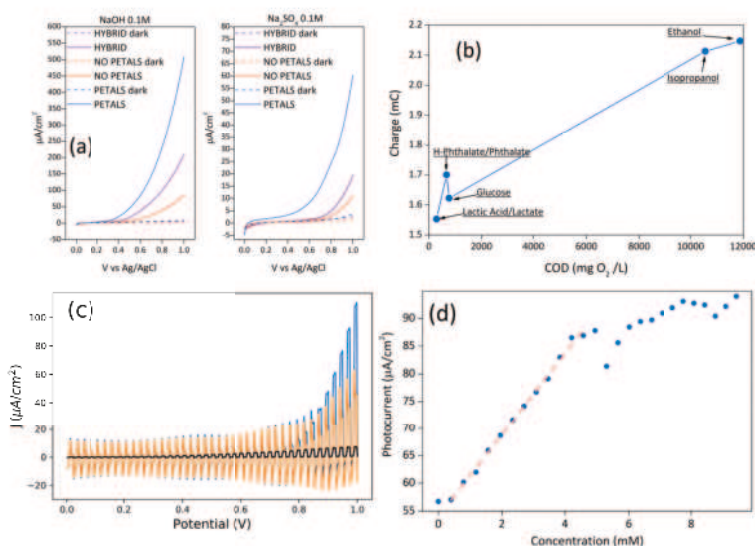
Figure 2. (a) LSV in 0.1 M Na 2 SO 4 and 0.1 M NaOH of the three samples in dark and illuminated conditions; (b) charge values at 1V vs. Ag/AgCl, from chronoamperometries (pH = 6), as a function of theoretical Chemical Oxygen Demand (COD) of the sample PETAL with different organic molecules in a 0.1 M sodium sulphate solution; (c) LSV with chopped illumination of the sample PETAL in sodium sulphate before (orange) and after (blue) the addition of glucose. The behavior of the bare silicon electrode is also shown for reference (black curve); (d) photocurrent dependence of sample PETAL at 1 V vs. Ag/AgCl on the concentration of glucose.
