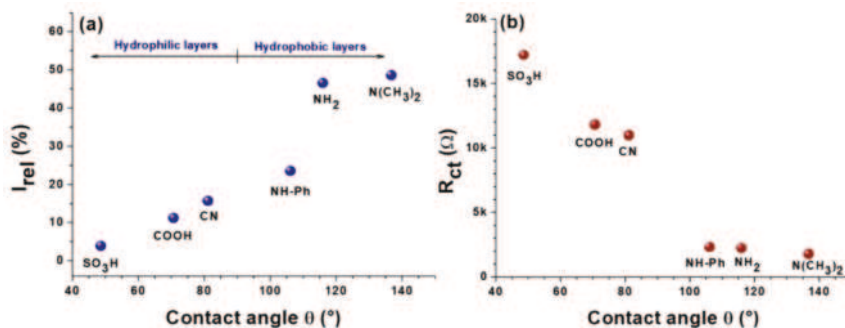
Figure 4. Correlations between the electrochemical and wetting properties of diazonium-modified flexible ITO electrodes: (a) I_{\text{rel}} -vs-water contact angle; and (b) R_{\text{ct}} -vs-water contact angle.
