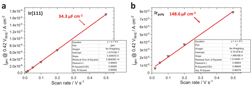
Figure 1. Double-layer capacitance measurements of (a) Ir(111) and (b) \text{Ir}_{\text{poly}} displaying the anodic charging current densities measured at 0.42 V_{\text{RHE}} .
