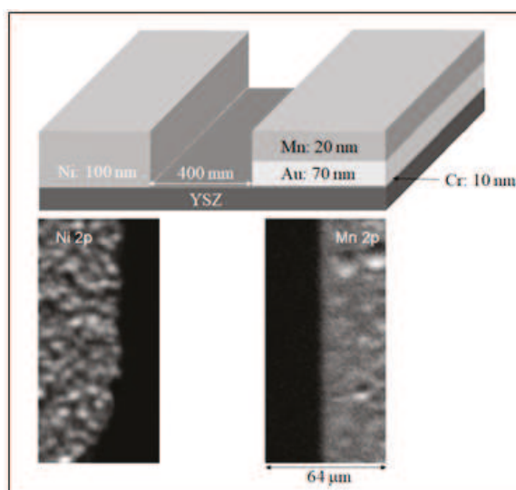
Figure 7. Scheme of the electrolyte (YSZ)–supported the planar cell with Ni and Mn electrodes for in situ electrochemical SPEM measurements. The images at the bottom are SPEM maps at the Ni 2p and Mn 2p energies of the electrode–electrolyte interfaces.
