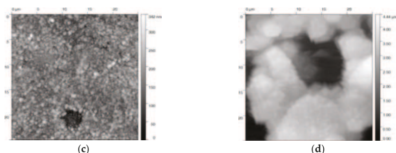
Figure 6. AFM images of steel samples electrochemically blackened in (a) blackening salt solution at 80 °C and (b) 130 °C, and (c) in NaOH at 80 °C, and (d) 120 °C. The images show a 25 × 25 μm 2 area of the individual samples.
