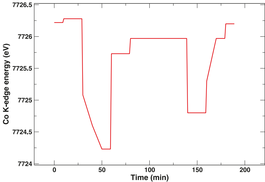
Figure 5. Energy of the Co K-edge, measured as the maximum of the first derivative of the XANES spectrum, as a function of time at 850 °C.
