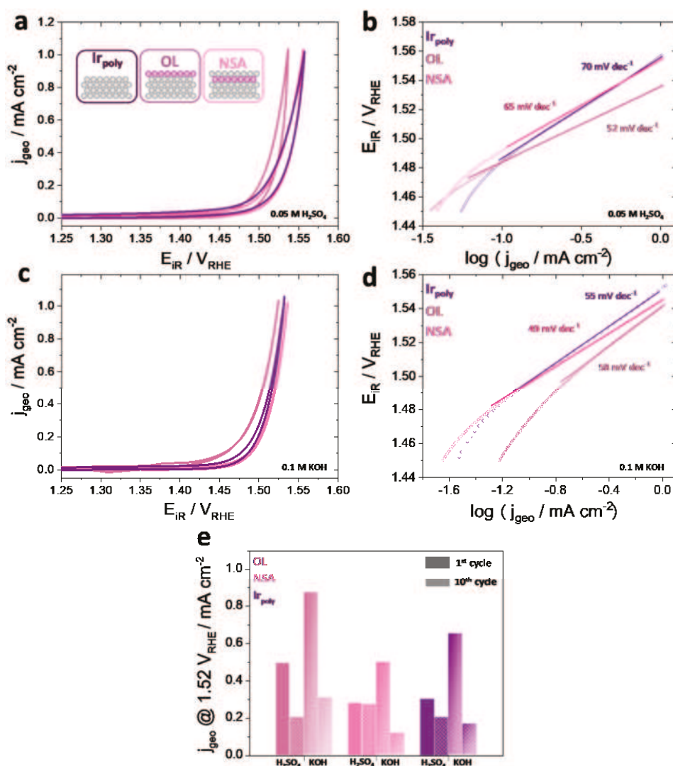
Figure 5. Electrocatalytic OER activities of Ni-modified Ir electrodes compared to pristine polycrystalline Ir at scan rates of 5 \text{ mV s}^{-1} . (a) 1st OER cycle in 0.05 M \text{H}_2\text{SO}_4 and (b) corresponding Tafel plots (with ohmic-drop correction) of Ir poly , Ni/Ir poly OL, and Ni/Ir poly NSA. (c) 1st OER cycle in 0.1 M KOH and (d) corresponding Tafel plots of all catalysts. (e) Current densities of electrodes measured at 1.53 V_{\text{RHE}} normalized to the electrode's geometric surface area of 0.785 \text{ cm}^{-2} for the 1st and 10th cycle. The 10th cycle is depicted in Figure S4 in the Supplementary Information.
