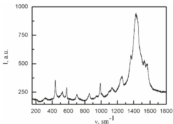
Figure 2. Raman spectrum of the nc-Si(2)/P3HT samples.
