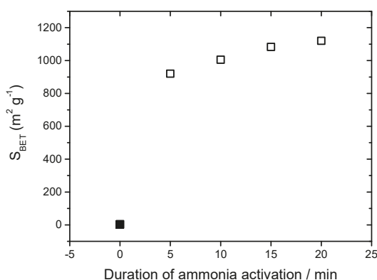
Figure 5. Effect of the duration of ammonia activation at 900^\circ\text{C} on the mass-specific surface area ( S_{\text{BET}} ) of \text{Zn}_7\text{-PAN}_{10}\text{-CNF} .
