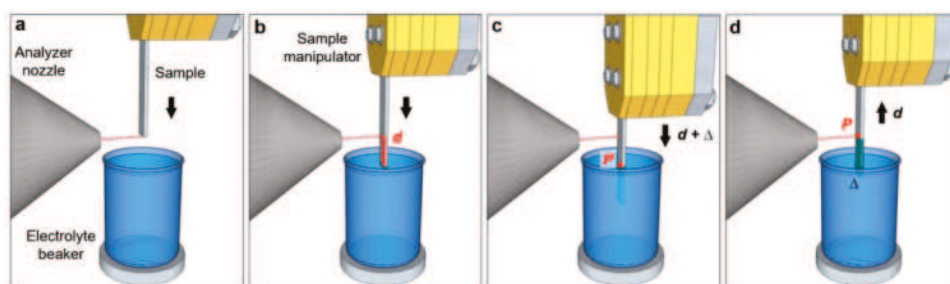
Figure 3. Schematization of the “dip and pull” method coupled with AP-HAXPES experiments. See text for the detailed explanation of the experimental procedure. The pressure inside the analysis chamber is generally close to the water vapor pressure at room temperature, thus enabling to work at about 100% relative humidity.
