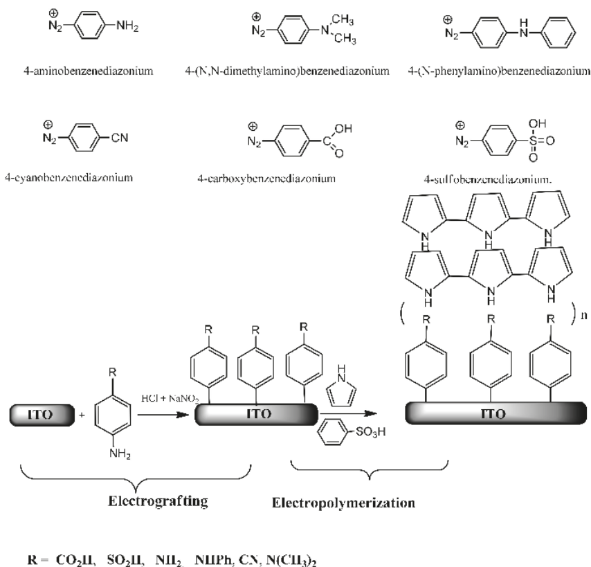
Figure 1. Upper panel: Chemical structures of the diazonium compounds under test. Lower panel: electrodeposition of benzene sulfonic acid-doped polypyrrole on diazonium-modified flexible ITO electrodes.
