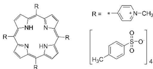
Figure 1. H_2TMPyP molecular structure.
