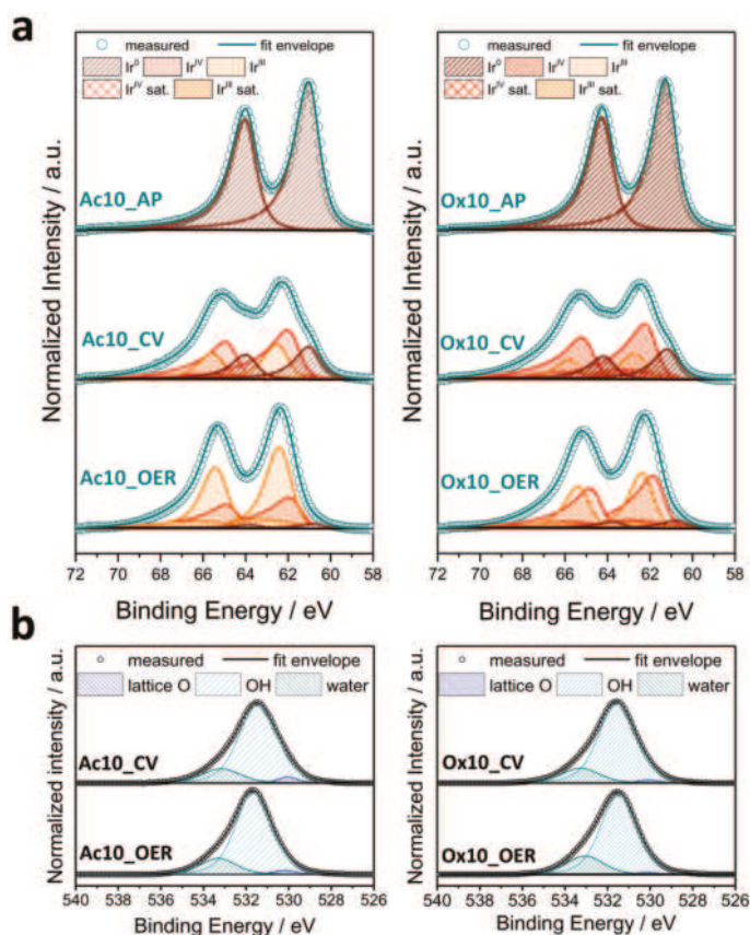
Figure 5. X-ray photoelectron spectroscopy of the Ac10 and Ox10 films at as-prepared states ( \text{AP} ), after cyclic voltammetry between 0.05–1.4 V_{\text{RHE}} ( \text{CV} ) and OER activity testing ( \text{OER} ) with fitted components of (a) Ir 4f and (b) O 1s species. The as-prepared samples only show metallic Ir ( \text{Ir}^0 ). Through potential cycling, the major part of metallic Ir was oxidized to \text{Ir}^{\text{III}} and \text{Ir}^{\text{IV}} . After stepped potential voltammetry with potentials up to 1.60 V_{\text{RHE}} , almost no \text{Ir}^0 is left and the ratio of \text{Ir}^{\text{III}} to \text{Ir}^{\text{IV}} is increased.
