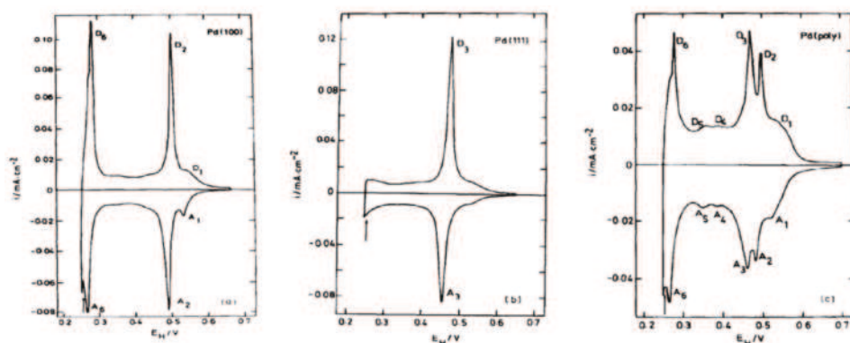
Figure 14. Cyclic voltammograms of Pd single-crystal electrodes in 0.5 mol L −1 NaClO 4 + 0.01 mol L −1 HClO 4 + 1 mmol L −1 Cu 2+ , at 10 mV s −1 : (a) Pd(1 0 0), (b) Pd(1 1 1), and (c) polycrystalline Pd. Reprinted from reference [100]. Copyright (1988) with permission from Elsevier.
