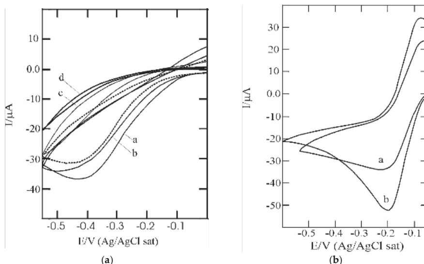
Figure 8. (a) Cyclic voltammograms obtained from 1 mM \text{Ru(NH}_3)_6^{3+} in 0.1 M KCl on \text{Ag(III)} covered by 30 ECALE cycles and modified with \text{C}_{16}\text{SH} for 20 min (curve a), 30 min (curve b), 90 min (curve c) and 4 h (curve d); the dashed curve was obtained after having further modified the substrate for 17 h; (b) cyclic voltammograms obtained from 1 mM \text{Ru(NH}_3)_6^{3+} in 0.1 M KCl on \text{Ag(III)} covered by 30 ECALE cycles and modified with \text{C}_{16}\text{SH} for 3 h (curve a), and more than 12 h (curve b). The scan rate was 50 mV/s.
