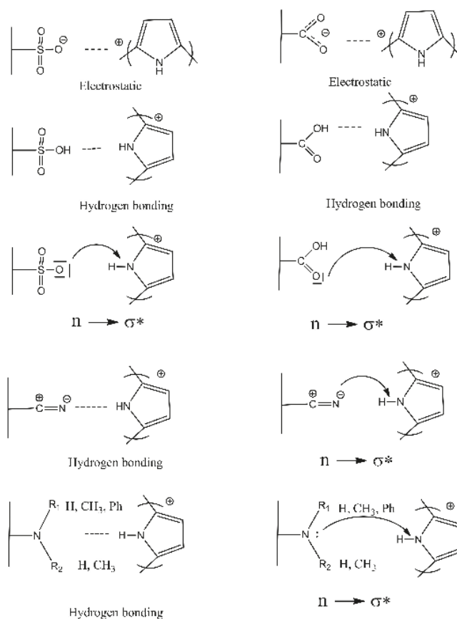
Figure 9. Possible molecular interactions at aryl-polypyrrole interfaces.
