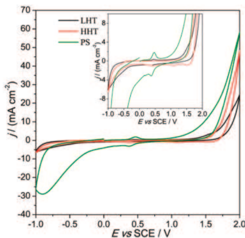
Figure 4. Cyclic voltammetry (CV) patterns of PS, LHT, and HHT nanofibers recorded in 0.1 M H 2 SO 4 at 100 mV s −1 . Zoom of the current density values in the inset.
