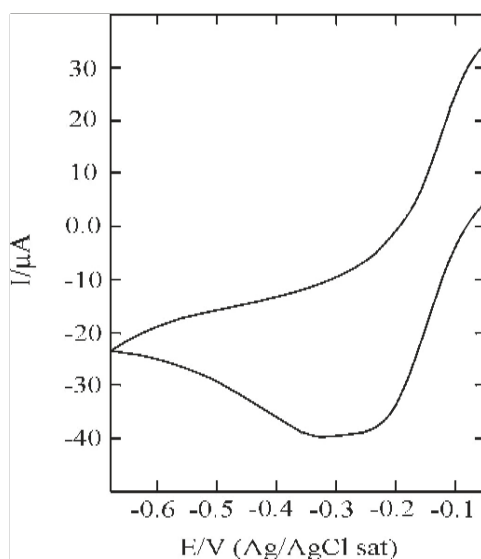
Figure 7. Cyclic voltammograms obtained from 1 mM \text{Ru}(\text{NH}_3)_6^{3+} in 0.1 M KCl on Ag(III) covered by 30 ECALE cycles in the absence of thiol. The scan rate was 50 mV/s.
