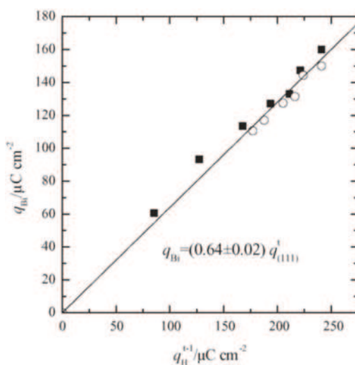
Figure 12. Charge density values of the bismuth redox peak vs. the charge associated with the (1 1 1) sites on the terraces, assuming that one electron is exchanged per site (■: Pt(n,n,n-2), ○: Pt(n+1,n-1,n-1) electrodes). Reprinted from reference [47]. Copyright (2005) with permission from Elsevier.
