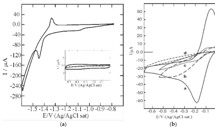
Figure 1. (a) Cyclic voltammograms of 0.1 mm C_{16}SH on Ag(III) electrodes using 0.1 M NaOH in 95% ethanol and 5% water as recorded from -0.8 V to -1.6 V/Ag/AgCl sat; inset: cyclic voltammogram of a bare Ag(III) (solid curve) and on Ag(III) modified for 15 min in C_{16}SH solution (dashed curve); (b) cyclic voltammograms obtained from 1 mm Ru(NH_3)_6^{3+} in 0.1 M KCl on the bare Ag(III) (curve a), and on Ag(III) covered by C_{16}SH deposited from a 0.03 mm solution for 10 min (curve b), 2 h (curve c) and 26 h (curve d). The scan rate was 50 mV/s.
