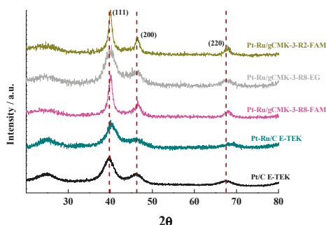
Figure 2. XRD patterns of the Pt–Ru catalysts supported on gCMK-3s and the commercial Pt/C and Pt–Ru/C from E-TEK.
