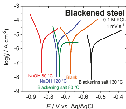
Figure 8. Potentiodynamic polarization curves for pristine and blackened steel surfaces in in 0.1 M KCl; scan rate 1 mV s −1 . Electrochemical blackening was performed both in 23 M NaOH and blackening salt solution.
