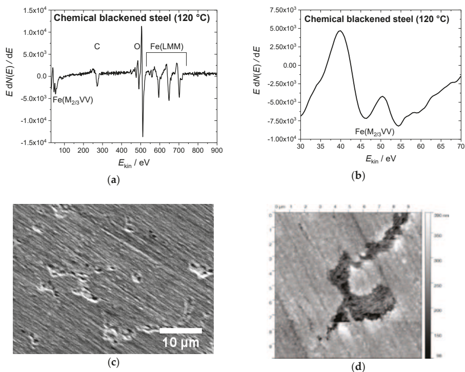
Figure 1. (a) Auger electron spectrum of a steel sample blackened at 120^\circ\text{C} in hot alkaline nitrite solution, showing (b) the \text{Fe}(\text{M}_{2/3}\text{VV}) signals at 46 and 54 eV with the intensity ratio of 7:10 for magnetite on the surface. (c) Scanning electron microscopy (SEM) image of the same sample (10 kV, 2000 magnification) with some defects in the blackened surface; (d) The atomic force microscopy (AFM) topography image shows a 10 \times 10 \mu\text{m}^2 area of the steel sample, scaling-up a surface defect similar seen in the SEM image.
