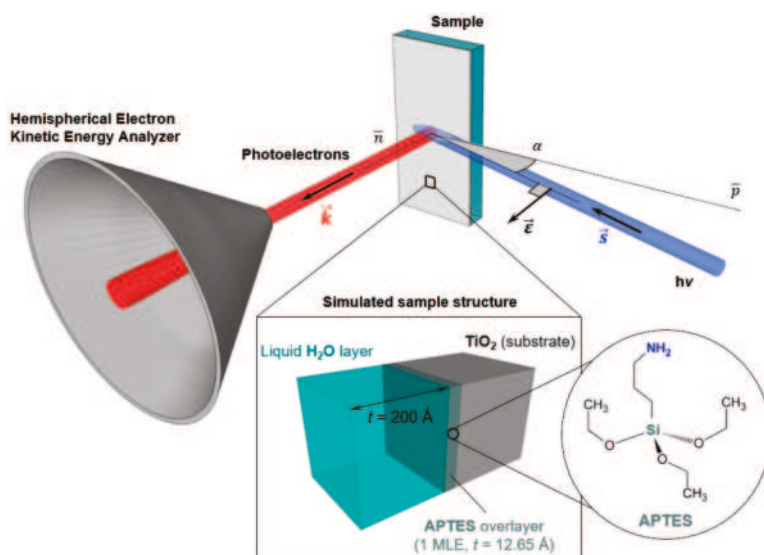
Figure 1. Schematization of the ambient pressure hard X-ray photoelectron spectroscopy (AP-HAXPES) experimental geometry (implemented in Simulation of Electron Spectra for Surface Analysis (SESSA) calculations) and 3-aminopropyl triethoxysilane (APTES)-functionalized TiO_2 model system used in this work.
