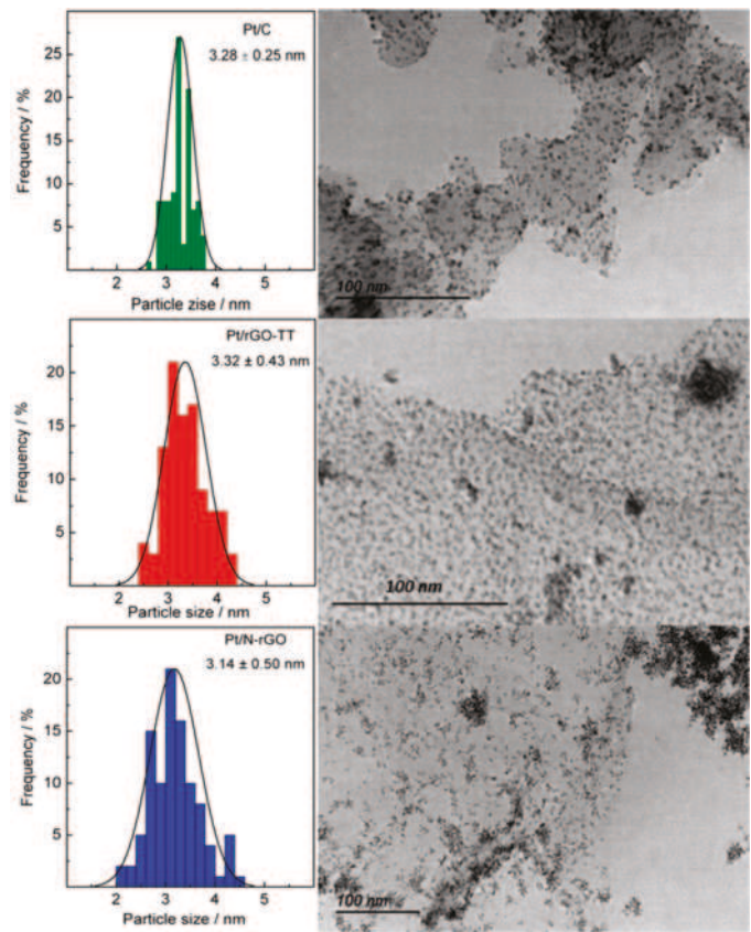
Figure 3. Transmission electron micrographs and particle size distribution histograms of the catalysts.
