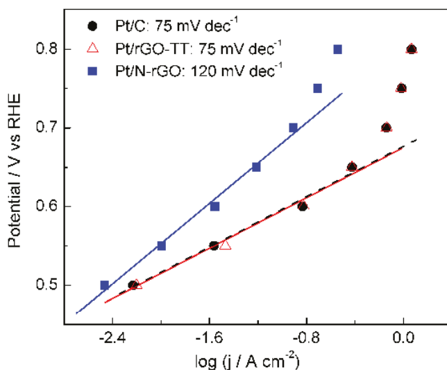
Figure 9. Tafel plots obtained at 300 s from Figure 8.
