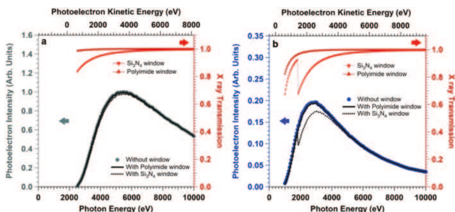
Figure 5. Si 1s (a) and N 1s (b) photoelectron intensity evolution as a function of the photon energy, with and without the X-ray window placed between the X-ray source and the sample. The two elements belong to the APTES overlayer buried by 20 nm of water. For a better comparison, the reported photoelectron intensities with no simulated absorber are normalized by the maximum value obtained at 5390 eV for the Si 1s core level. The right axes of Figure a,b report the X-ray transmission through a \text{Si}_3\text{N}_4 and polyimide (Kapton) window. For both materials, the simulated window thickness is 500 nm, which is a common value for X-ray windows used during AP-HAXPES experiments. To simulate the effect of the X-ray window on the photoelectron response, the X-ray transmission curves have been convoluted with the photoelectron intensity trends obtained in absence of an X-ray absorber.
