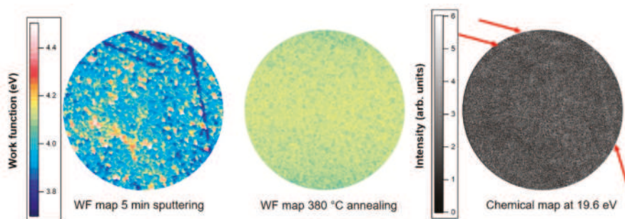
Figure 4. WF maps of the Pb on Au after the 5 min sputtering (left) and 380 °C annealing (center) steps. On the (right), a normalized EF-PEEM image at 19.6 eV BE for Pb after 5 min of sputtering. The arrows are a guide to the eye highlighting some features in the image. The images were taken in the same area, with a field of view of 17.2 μm.
