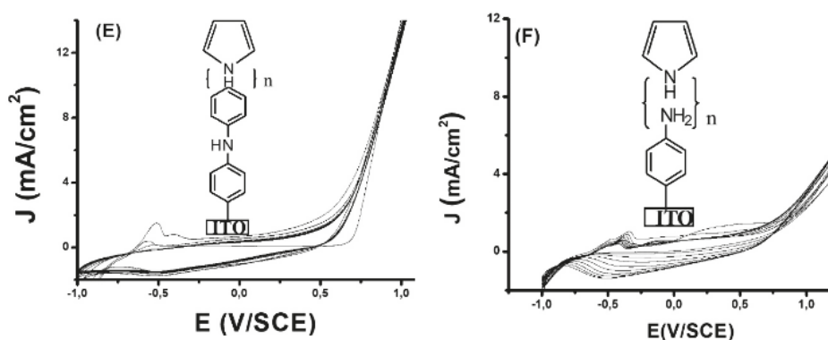
Figure 5. Electrosynthesis of PPy-BSA films by cyclic voltammetry on (A) ITO-SO 3 H; (B) ITO-CO 2 H; (C) ITO-CN; (D) ITO-N(CH 3 ) 2 ; (E) ITO-NH-Ph; and (F) ITO-NH 2 .
