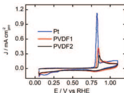
Figure 2. CO stripping curves recorded for polycrystalline Pt and the two PVDF modified surfaces at room temperature in Ar saturated 0.05 M H 2 SO 4 electrolyte solution. The scan rate was 50 mVs −1 . PVDF 1 stands for the film prepared by dip coating the Pt electrode into 0.1 mM PVDF solution, PVDF 2 for the film prepared by dip coating into 0.1 M PVDF solution. The roughness factors (Rf) calculated by CO stripping for the bare Pt surface, PVDF1 and PVDF2 are: 1.40, 1.17, 0.51. This corresponds to an ECSA loss with respect to the bare polycrystalline Pt electrode of 17 % and 64 % for PVDF 1 and PVDF 2, respectively.
