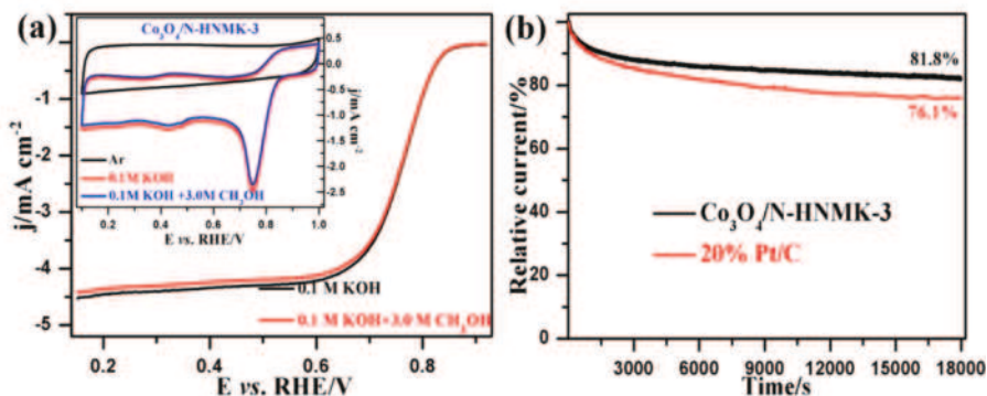
Figure 7. (a) CV and LSV curves of Co_3O_4/N\text{-HNMK-3} in O_2 -saturated with or without 3.0 M methanol in 0.1 M KOH; (b) The durability test of Co_3O_4/N\text{-HNMK-3} and 20 wt.% Pt/C at 0.70 V in O_2 -saturated 0.1 M KOH at 1600 rpm.
