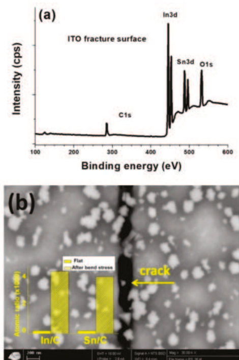
Figure 8. Adhesion testing of polypyrrole thin films on (a) bare ITO using XPS; and (b) ITO-NH 2 using SEM and XPS. Inset of 8b shows the bar graph of In/C atomic.
