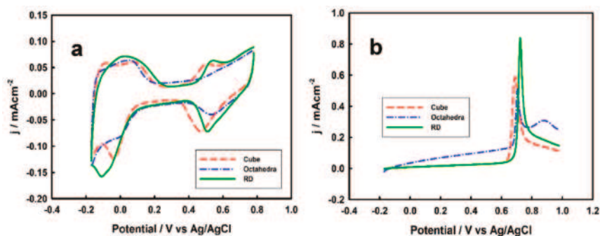
Figure 4. (a) CVs; (b) CO stripping voltammograms of cubic, octahedral, and RD Au nanocrystals coated with one monolayer of Pd recorded in 0.1 M \text{HClO}_4 . Scan rate: 0.100 \text{ V s}^{-1} .
