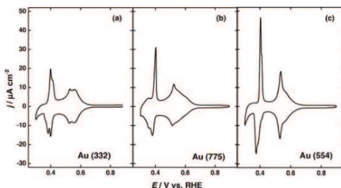
Figure 4. Cyclic voltammograms of (a) Au(3 3 2); (b) Au(7 7 5); and (c) Au(5 5 4) in 0.05 \text{ mol L}^{-1} \text{H}_2\text{SO}_4 + 1 \text{ mmol L}^{-1} \text{CuSO}_4 at 5 \text{ mVs}^{-1} . Reprinted from reference [19]. Copyright (2004) with permission from Elsevier.
