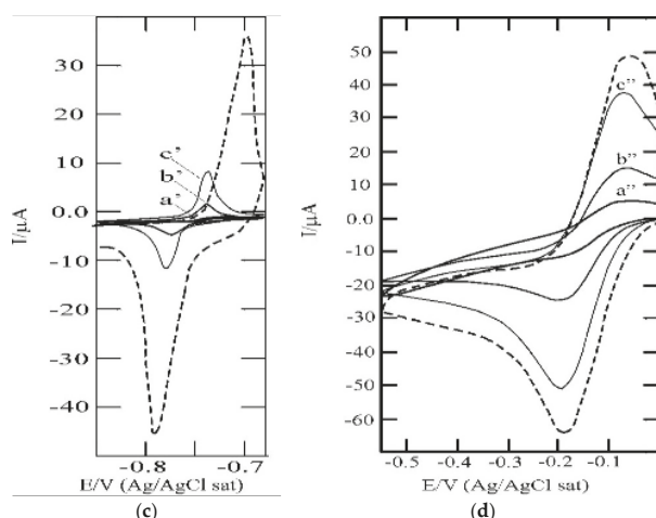
Figure 3. (a) Oxidative UPD of S on Ag(III) from 1 mM Na 2 S, as recorded from -1.1 to -0.68 V; (b) oxidative UPD of S on Ag(III) modified with C 16 SH for 16 h and successively treated at E = -1.8 for 1 min (curve a), 3 min (curve b) and 4 min (curve c) up to a total time of 8'; (c) oxidative UPD of S on Ag(III) modified with C 16 SH for 2 h (curve a') and successively treated at E = -1.6 V for 3 min (curve b') and further 2 min (curve c') up to a total time of 5 min; as comparison, the dashed curve is the curve on the bare Ag(III); (d) cyclic voltammograms obtained from 1 mM Ru(NH 3 ) 6 3+ in 0.1 M KCl on Ag(III) modified with C 16 SH for 2 h (curve a'') and successively treated at E = -1.6 V for 3 min (curve b'') and further 2 min (curve c'') up to a total time of 5 min; as comparison, the dashed curve is the curve on the bare Ag(III). All curves were recorded in pH 9.2 ammonia buffer solutions. The scan rate was 50 mV/s.
