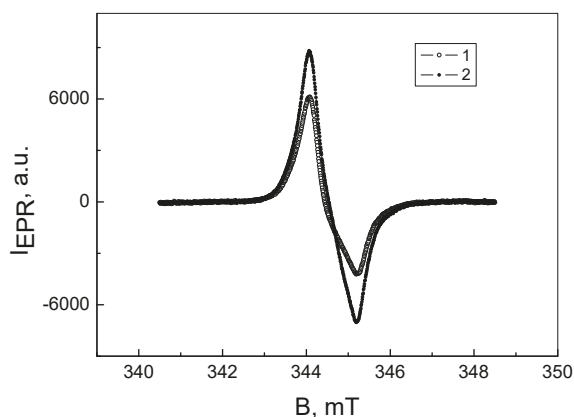
Figure 5. EPR spectra of nc-Si(1) in the dark (1) and under illumination (2).
