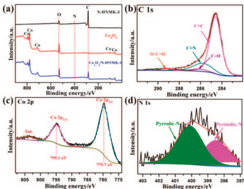
Figure 5. (a) XPS survey scan of samples: N-HNMK-3, \text{Co}_3\text{O}_4 and \text{Co}_3\text{O}_4/\text{N-HNMK-3} ; XPS spectra of (b) C 1s; (c) Co 2p; (d) N 1s of \text{Co}_3\text{O}_4/\text{N-HNMK-3} .
