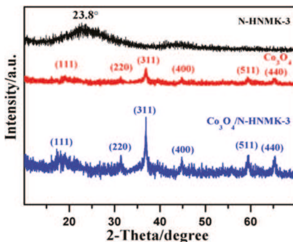
Figure 2. Powder XRD patterns of N-HNMK-3, \text{Co}_3\text{O}_4 , and \text{Co}_3\text{O}_4/\text{N-HNMK-3} composite.
