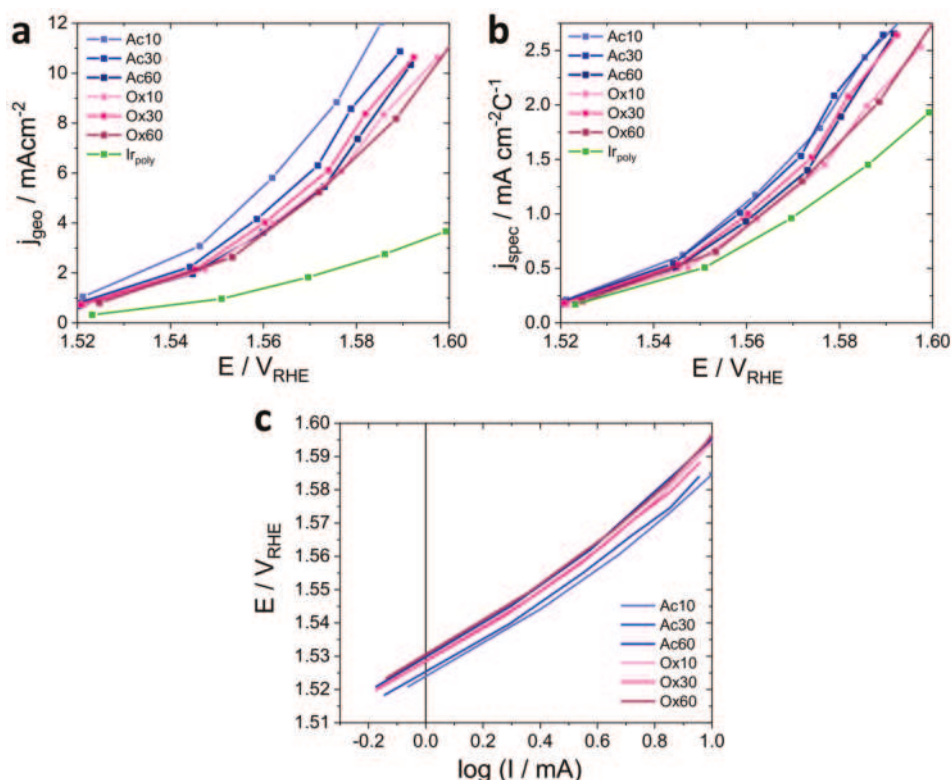
Figure 4. Electrochemical OER activity curves of Ac and Ox films obtained by stepped potential voltammetry. (a) Geometrical current densities in 0.05 M \text{H}_2\text{SO}_4 . The shorter heated Ac films exhibit a slightly higher activity compared with the Ox films and longer heated Ac films. (b) Specific current density in 0.05 M \text{H}_2\text{SO}_4 based on the anodic charge obtained from the last scan (between 0.4 and 1.4 V_{\text{RHE}} ) before SPV. Because of charge normalization, the activities of the Ac films no longer differ significantly from each other. The relation of the Ox films' activities to each other is not affected. (c) Tafel plot of the _OER films extrapolated from the stepped potential voltammetry (SPV) measurements.
