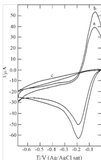
Figure 4. Cyclic voltammograms obtained from 1 mM \text{Ru}(\text{NH}_3)_6^{3+} in 0.1 M KCl on Ag(III) covered by 10 ECALE cycles and modified with \text{C}_{16}\text{SH} for 26 h (curve a), on bare Ag(III) (curve b), and on Ag(III) modified with \text{C}_{16}\text{SH} in the absence of CdS (curve c). The scan rate was 50 mV/s.
