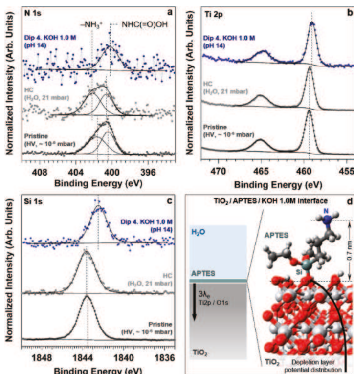
Figure 7. N 1s (a), Ti 2p (b) and Si 1s (c) core level spectra acquired at the pristine conditions, hydrated conditions (HC) and after dipping the sample in the KOH 1.0 M solution (pH 14). (d) Relaxed structure obtained from the molecular dynamics simulation of the adsorption of one APTES molecule on a rutile TiO 2 (110) surface through the formation of one Ti–O–Si bond (white: titanium; light grey: hydrogen; dark grey: carbon; light green: silicon; red: oxygen; blue: nitrogen).
