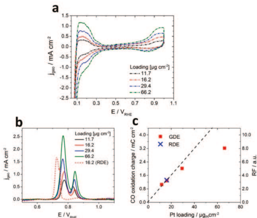
Figure 3. (a) Loading dependent electrochemical behaviour of Pt TF in GDE setup (298 K, 4 M \text{HClO}_4 , 0% RH), cyclic voltammograms recorded with 50 \text{ mV s}^{-1} and Ar saturated flow field. (b) CO stripping curves recorded with 50 \text{ mV s}^{-1} . (c) Plot of CO oxidation charge as function of the Pt loading on the GDE and RDE. The linear slope indicates the ideal correlation between oxidation charge and Pt loading.
