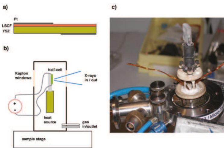
Figure 1. (a) LSCF/YSZ half-cell. (b) Schematic of the X-ray absorption spectroscopy setup. (c) Inner view of the cell.
