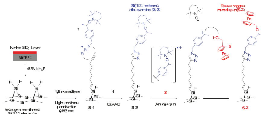
Scheme 2. Light-assisted (365 nm) hydrosilylation of 1,8-nonadiyne to passivate an hydrogen-terminated Si(100) surface (S-1) and covalent attachment of alkoxyamine 1 via CuAAC “click” reactions to yield an alkoxyamine monolayer (S-2). Anodization of S-2 in the presence of the alcohol nucleophile 2 leads to release of TEMPO in the electrolyte with formation of a redox-active monolayer (S-3) by reaction of 2 with the putative surface-tethered carbocation intermediate.
