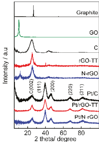
Figure 1. XRD patterns of graphite, graphene oxide (GO), Vulcan carbon (C), reduced graphene oxide by thermal treatment (rGO-TT), nitrogen-modified reduced graphene oxide (N-rGO), Pt/C, Pt/rGO-TT, and Pt/N-rGO.
