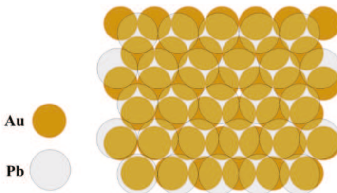
Figure 6. Representation of the hexagonal monolayer of lead on \text{Au}(1\ 1\ 1) .
