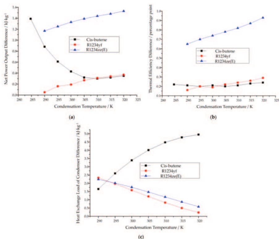
Figure 8. Variation in the difference in thermodynamic performance with increasing condensation temperature in the subcritical cycle model when the condensation temperature is known: (a) net power output, (b) thermal efficiency, (c) heat exchange load of the condenser.
