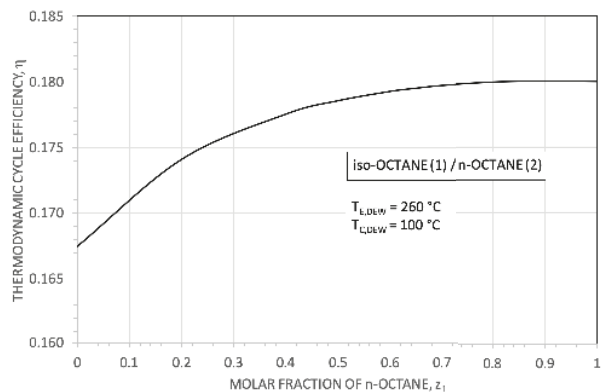
Figure 12. Thermodynamic cycle efficiency for the mixture iso-octane/n-octane as a function of the molar fraction of n-octane. The considered cycles are all subcritical with saturated vapour.
