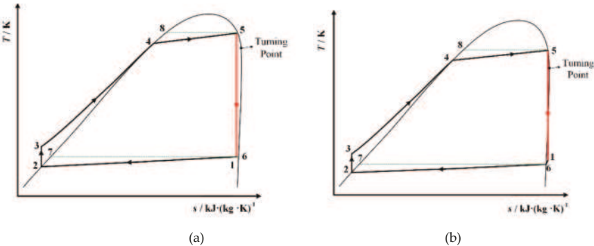
Figure 5. Subcritical ORC using single screw expander with isentropic zeotropic mixture as working fluid: (a)expander outlet at vapor-liquid two-phase region for R436A; (b)expander outlet at superheated region. for R436B.
