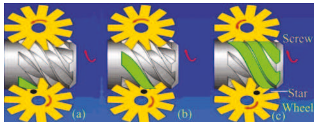
Figure 3. Working processes of CP type single screw expander (a) suction, (b) expansion, and (c) discharge.
