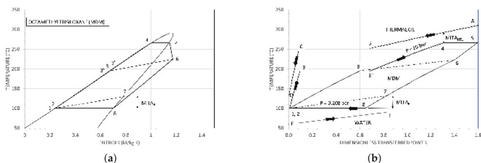
Figure 3. (a) Reference thermodynamic cycle with MDM as working fluid in a T-S plane. (b) The heat sources (thermal oil in HT_1 and in HT_2 loops and the cooling water) and the thermodynamic cycle in a temperature—dimensionless power plane.
