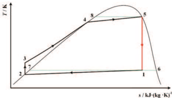
Figure 4. Subcritical ORC using single screw expander with wet zeotropic mixture as working fluid.
