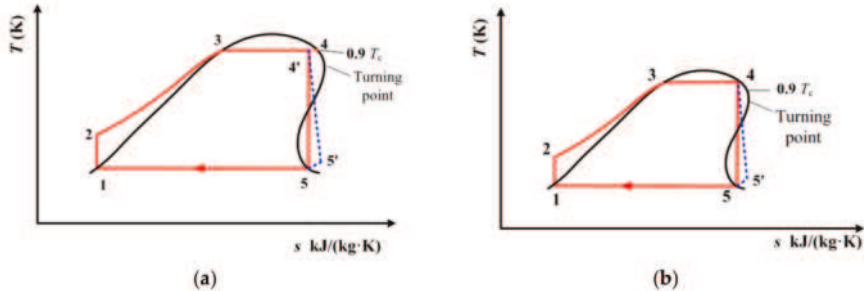
Figure 13. (a) Subcritical and (b) transcritical cycles of cis-butene when considering the isentropic efficiency of the expander.
