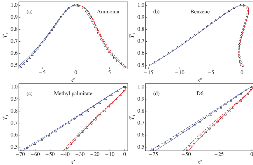
Figure 3. Liquid–vapor saturation boundary in a T_r – s^* diagram for: (a) ammonia; (b) benzene; (c) methyl palmitate; and (d) D6. The solid lines correspond to the results of approximation A3 for the entropies of the saturated vapor s_{g,A3}^* (solid red line) and the saturated liquid s_{l,A3}^* (solid blue line). The dashed lines correspond to the results of approximation A1 for the entropies of the saturated vapor s_{g,A1}^* (dashed red line) and the saturated liquid s_{l,A1}^* (dashed blue line). The symbols are RefProp 9.1 results for s_g^* (circles) and s_l^* (triangles).
