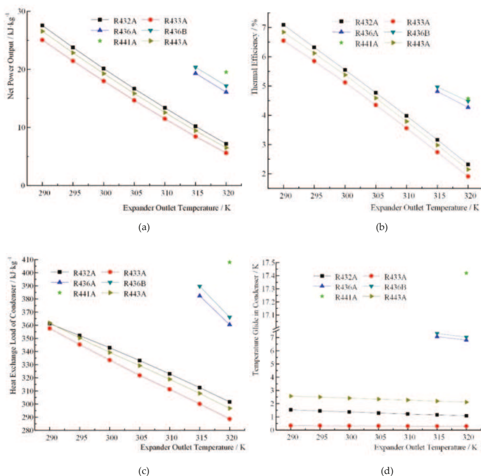
Figure 10. Variation trend of four indicators with the increase of expander outlet temperature when considering isentropic efficiency of expander: (a) net work; (b) thermal efficiency; (c) heat exchange load of condenser; (d) temperature glide in condenser.
