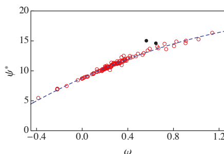
Figure 2. \psi^* vs. \omega for the 121 fluids of RefProp 9.1 [17] at a reduced temperature \bar{T}_{Mr} = 0.81 . The dashed blue line is the result of a quadratic fit to the data (red circles) excluding ethanol and methanol (solid black circles).
