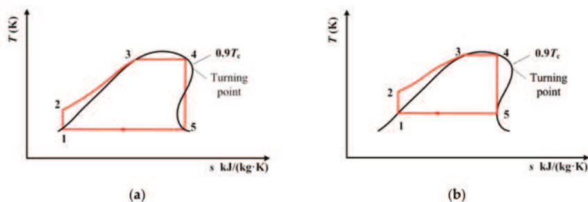
Figure 9. Transcritical ORC for cis-butene with single-screw expander when the condensation temperature is known: (a) 290 K, (b) 320 K.
