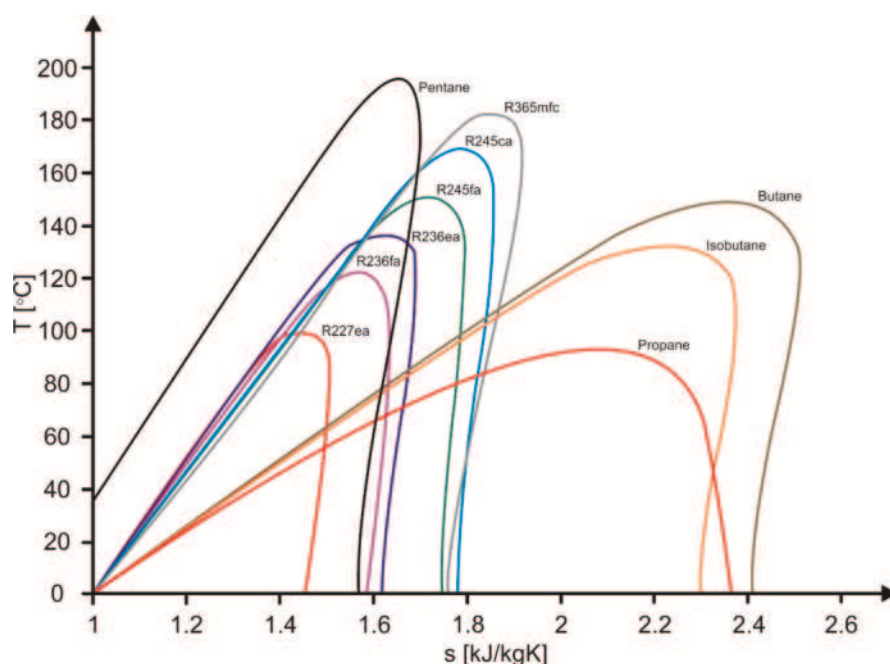
Figure 2. Saturation curves of different low-boiling working fluids.
