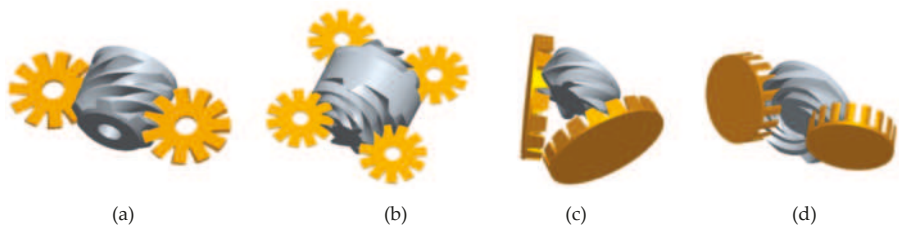
Figure 1. Four forms of single screw structure: (a) CP type; (b) CC type; (c) PP type; (d) PC type.
