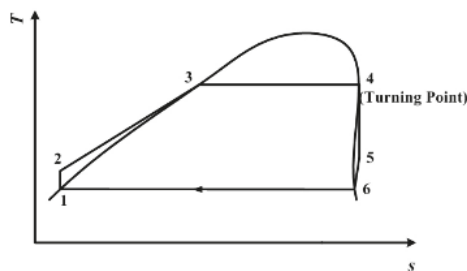
Figure 4. Traditional subcritical ORC with dry/isentropic working fluid.
