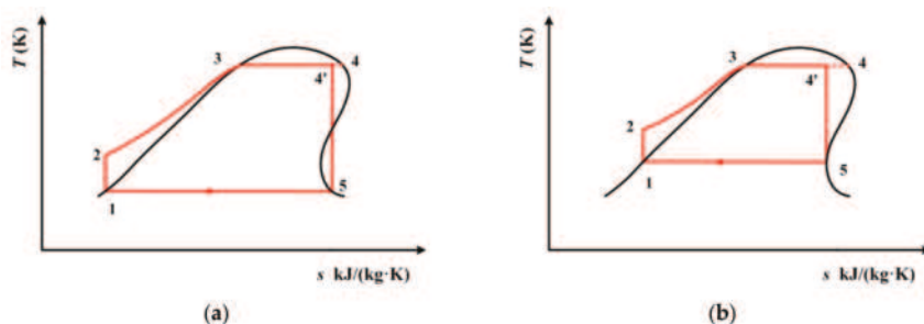
Figure 6. Subcritical ORC for cis-butene with a single-screw expander when the condensation temperature is known: (a) 290 K, (b) 320 K.
