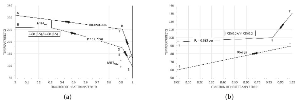
Figure 9. Temperature-thermal power exchanged for the cycle operating with the mixture i-C8 (0.5)/n-C8 (0.5) in the (a) High Temperature heat exchangers. (b) Condenser.
