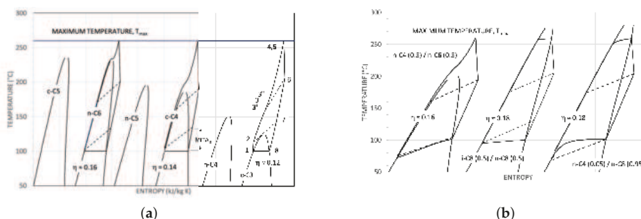
Figure 7. (a) Configuration of some (supercritical) thermodynamic cycles in the T-S plane (pure fluids); (b) Configuration of some thermodynamic cycles in the T-S plane for hydrocarbon mixtures.
