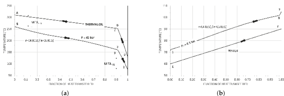
Figure 8. Temperature - Thermal power exchanged ( T - \dot{Q} diagrams) for the the equimolar mixture n-C4/n-C6. (a) in the hot oil heat exchangers. (b) in the condenser.
