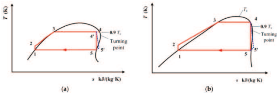
Figure 14. (a) Subcritical and (b) transcritical cycles of R1234yf and R1234ze(E) when considering the isentropic efficiency of the expander.
