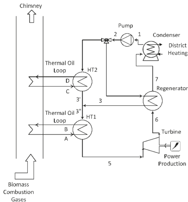
Figure 1. The reference plant scheme assumed as a reference case. Adapted from [17].
