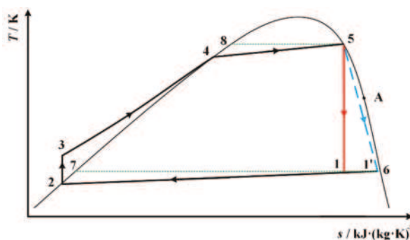
Figure 12. Point A with the longest distance between the outlet of the single screw expander and the saturated vapor curve.
