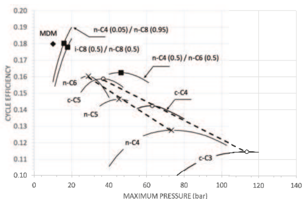
Figure 6. Thermodynamic cycle efficiency as a function of the maximum pressure.
