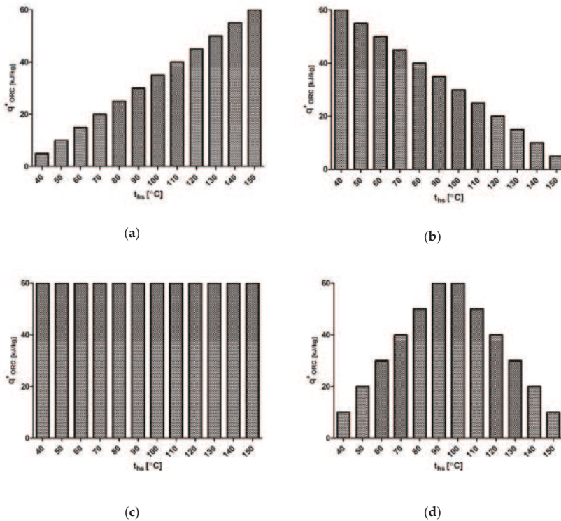
Figure 5. Histograms of different heat sources: (a) ascending; (b) descending; (c) constant; (d) parabolic.
