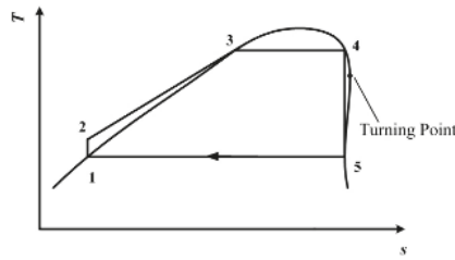
Figure 3. Subcritical ORC with a single-screw expander when the working conditions of the expander inlet are known.
