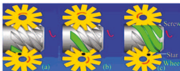
Figure 2. Working processes of single-screw expanders: (a) suction, (b) expansion, and (c) discharge.
