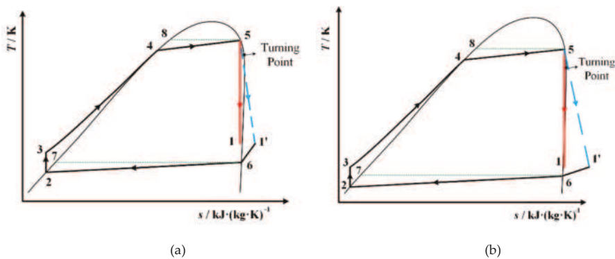
Figure 9. Subcritical ORC using single screw expander with isentropic zeotropic mixture as working fluid when considering isentropic efficiency of expander: (a) expander outlet at superheated region for R436A; (b) expander outlet at superheated region for R436B.
