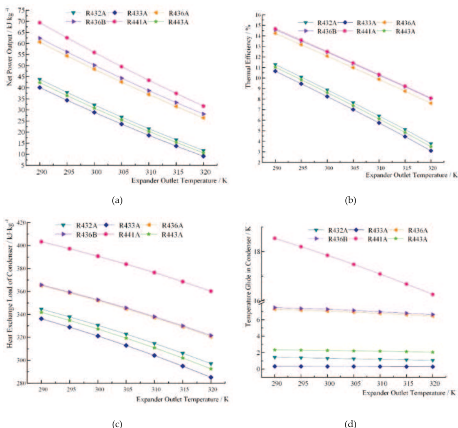
Figure 6. Variation trend of four indexes with the increase of expander outlet temperature: (a) net work; (b) thermal efficiency; (c) heat exchange load of condenser; (d) temperature glide in condenser.
