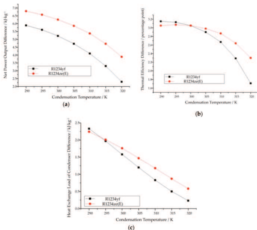
Figure 11. Variation in the difference in thermodynamic performance with increasing condensation temperature in the transcritical cycle model when the condensation temperature is known: (a) net power output, (b) thermal efficiency, (c) heat exchange load of the condenser.
