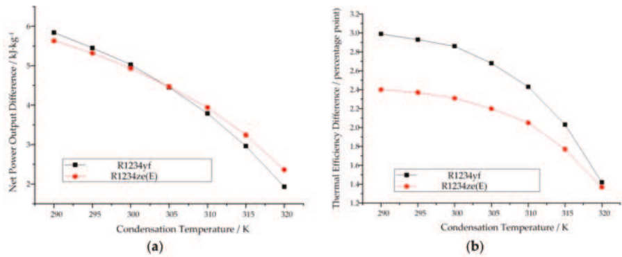
Figure 12. Thermodynamic performance difference variation between subcritical and transcritical cycle with increase of condensation temperature: (a) Net power output, (b) Thermal efficiency.
