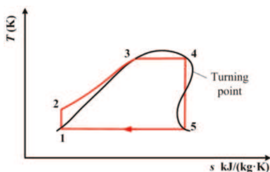
Figure 5. Shape of the saturated vapor curve of R1234yf, resulting in two intersections with the isentropic line.
