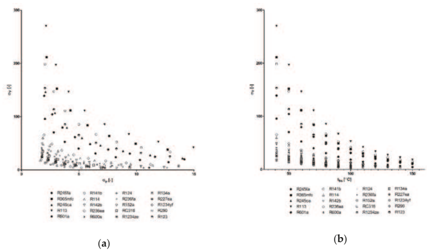
Figure 16. The variation of the \sigma_V parameter vs. the pressure expansion ratio and heat source temperature: (a) \sigma_V = f(\sigma_P) ; (b) \sigma_V = f(t_{hs}) .
