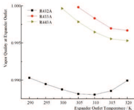
Figure 11. Relation between vapor quality at the expander outlet and the expander outlet temperature.
