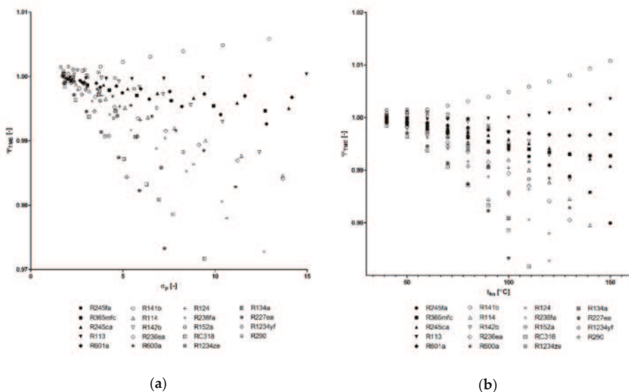
Figure 13. The variation of \psi_{TME} parameter vs. pressure expansion ratio and heat source temperature: (a) \psi_{TME} = f(\sigma_p) ; (b) \psi_{TME} = f(t_{hs}) .
