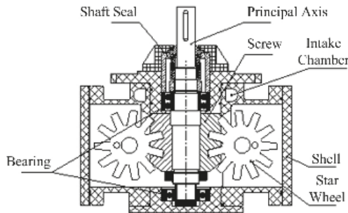
Figure 2. Configuration of CP type single screw expander.
