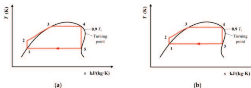
Figure 10. Transcritical ORC for R1234yf and R1234ze(E) with single-screw expander when the condensation temperature is known: (a) 290 K, (b) 320 K.
