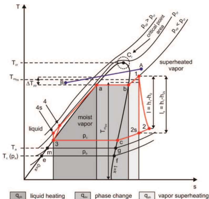
Figure 1. T-s diagram of a low-boiling working fluid.
