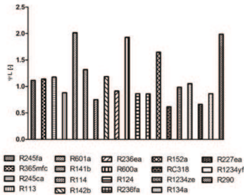
Figure 18. The variation of the \psi_L rating parameter (graph is valid for the heat sink temperature of t_c = 20\text{ }^\circ\text{C} ).
