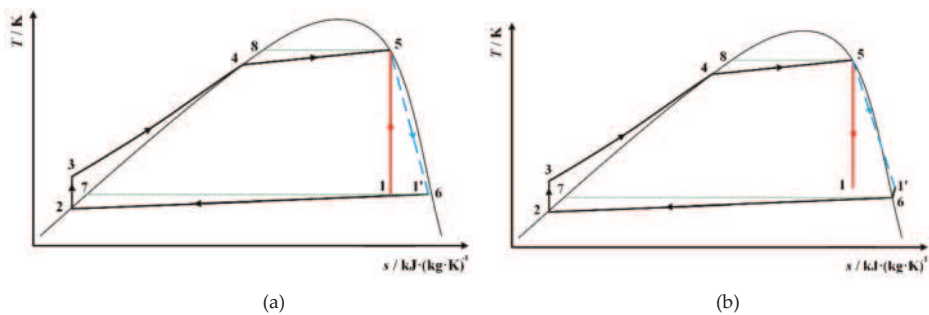
Figure 8. Subcritical ORC using single screw expander with wet zeotropic mixture as working fluid when considering isentropic efficiency of expander: (a) expander outlet at vapor-liquid two-phase region; (b) expander outlet at superheated region.
