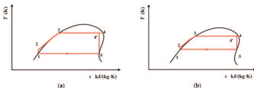
Figure 7. Subcritical ORC for R1234yf and R1234ze(E) with a single-screw expander when the condensation temperature is known: (a) 290 K, (b) 320 K.
