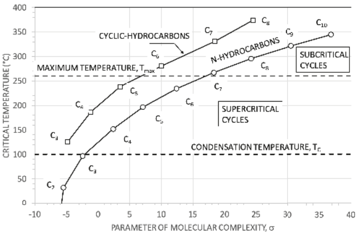
Figure 2. Critical temperature as a function of the molecular complexity parameter for linear (normal) hydrocarbons and cyclic hydrocarbons.
