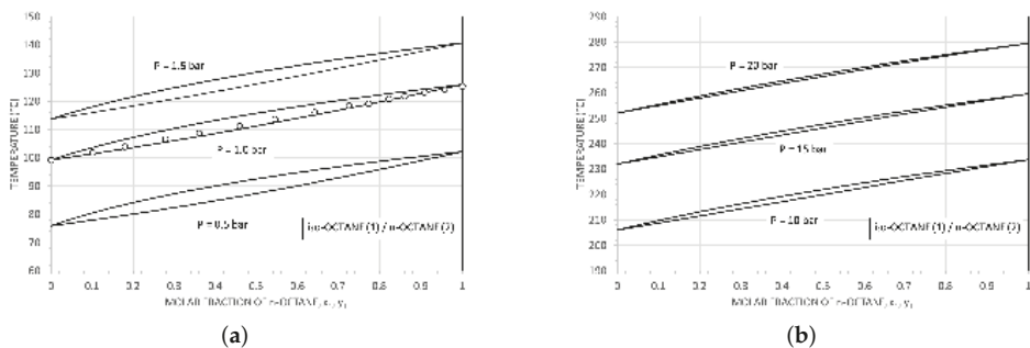
Figure 11. T – xy diagrams for the mixture i-C8 (0.5)/n-C8 (0.5) at different pressures. The white circles are from experimental literature data [44], and are reported as a comparison with the calculated values.
