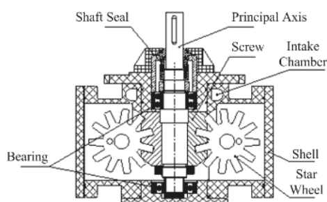
Figure 1. Configuration of a single-screw expander.
