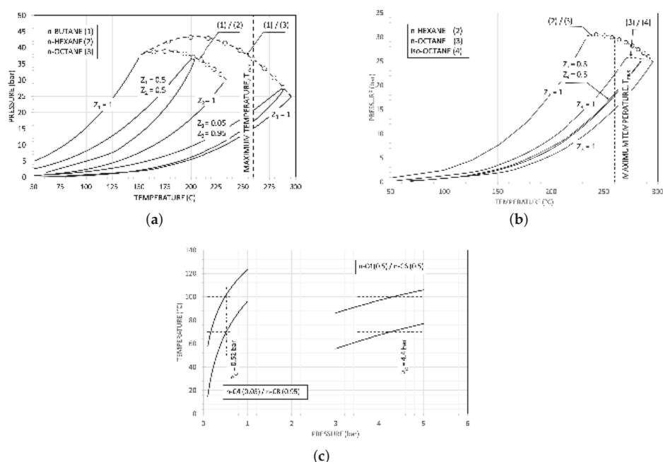
Figure 5. Critical loci for some mixtures (dotted lines). The white circle are from experimental literature data [35]. (a) Critical loci and some P - T envelopes for mixtures of n-C4/n-C6 and n-C4/n-C8. (b) Critical loci and P - T envelopes for mixtures of n-C6/n-C8 and n-C8/i-C8. (c) P - T envelopes for two mixtures around a dew temperature of 100 °C.
