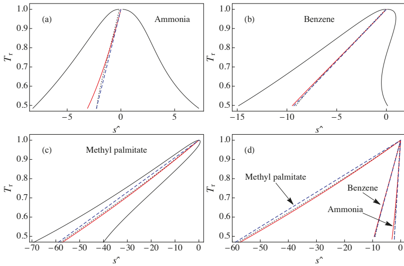
Figure 1. T_r - s^* diagram for: (a) ammonia; (b) benzene; and (c) methyl palmitate. The solid red line corresponds to the ideal gas contribution to the entropy s^{ig0*} defined in Equation (17), the dotted black line is the constant quality entropy s_{q,A1}^* obtained from Equation (4) with \bar{q} = 0.385 , and the dashed blue line shows s_{q,A1}^* = b(1 - T_r) with b obtained from Equation (11) (approximation A1). The solid black line represents the liquid–vapor saturation boundary. (d) A comparison of the results for s^{ig0*} , s_{q,A1}^* , and s_{q,A1}^* presented in (a–c). All data were obtained using RefProp 9.1 [17].
