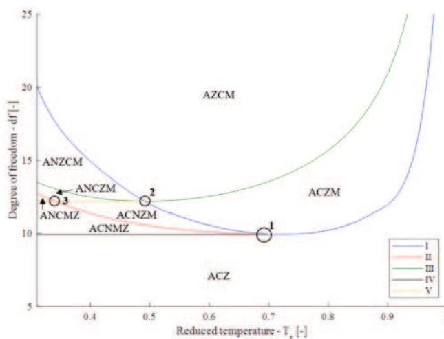
Figure A2. Correlation curves ( df vs. T_r ) for the different borders of the maps shown in Figure 4.
