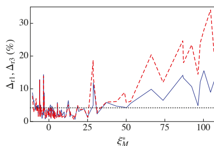
Figure 5. The percent relative deviations \Delta_{r1} and \Delta_{r3} vs. \zeta_M^* . For clarity, the deviations are plotted with lines: the dashed red line corresponds to \Delta_{r1} and the solid blue line represents \Delta_{r3} . The dotted line indicates a deviation level of 5%. The data for \Delta_{r1} , \Delta_{r3} , and \zeta_M^* are listed in Table A1.
