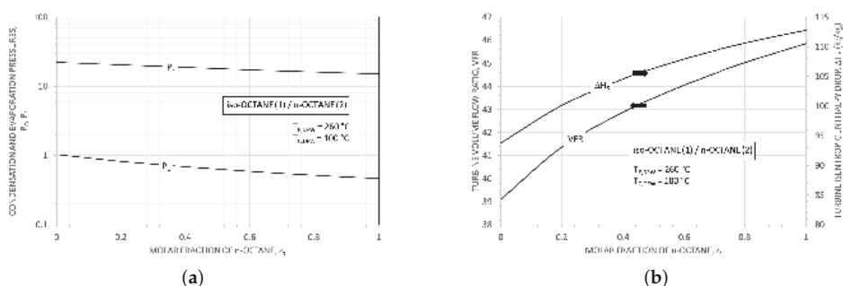
Figure 13. For a mixture of iso-octane/n-octane: (a) The trend of the evaporation and of the condensation pressures with the molar fraction of n-octane. (b) The variation of the isentropic enthalpy drop in turbine and of the isentropic volume flow ratio with the molar fraction of n-octane.
