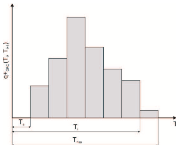
Figure 4. Example of the heat source histogram.
