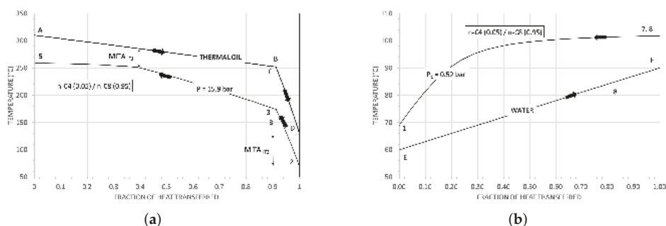
Figure 10. Temperature-thermal power exchanged for the cycle operating with the mixture n-C4 (0.05)/n-C8 (0.95) in the (a) High Temperature heat exchangers. (b) Condenser.
