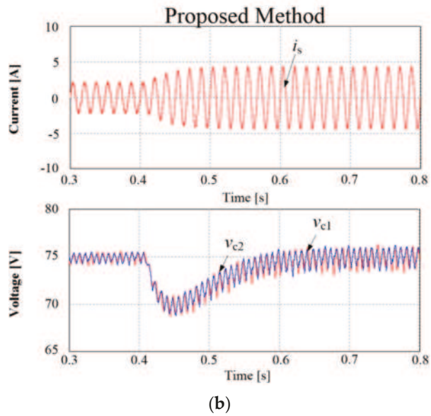
Figure 11. Simulation results of capacitor voltages ( v_{c1} , v_{c2} ) and source current with step change of load resistor from 200\ \Omega to 100\ \Omega obtained by (a) conventional method and (b) proposed method.
