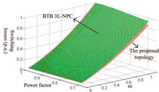
Figure 2. Switching losses comparison.
