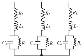
Figure 7. Three-phase load circuit.
