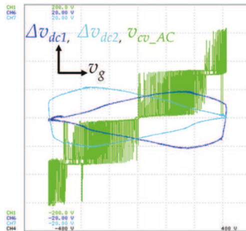
Figure 17. Experimental results in x-y mode showing the DC-link voltage ripple ( \Delta v_{dc1} : 5 V/div, \Delta v_{dc2} : 5 V/div) (y-axis) and the voltage levels produced by the grid-side converter ( v_{cv\_AC} : 50 V/div) (y-axis), both in function of the power grid voltage ( v_g : 100 V/div) (x-axis).
