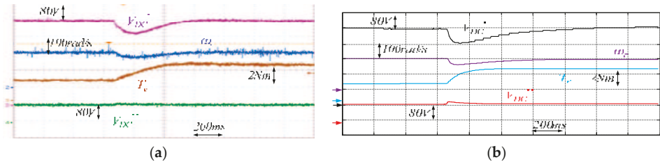
Figure 25. Load transient from T_L = 2 Nm to T_L = 4 Nm at \omega_r = 200 rad/s and V_{DC}' = 400 V, V_{DC}'' = 100 V. Output voltage V_{DC}' , TLI DC bus voltage V_{DC}'' , rotor speed \omega_r , electromagnetic torque T_e . (a) Experimental results. (b) Simulation results.
