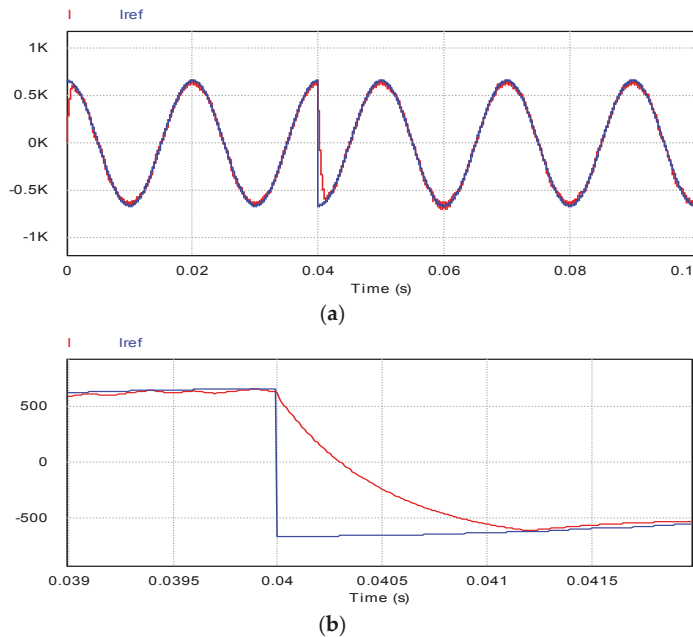
Figure 10. Load current for a sudden change: (a) reference current and actual load current; (b) Detail of the reference current and actual load current at the instant.
