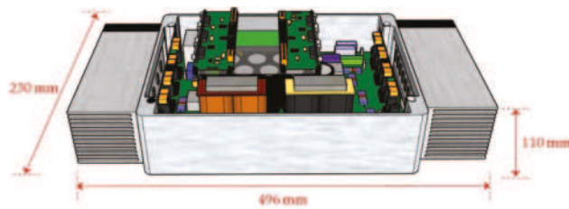
Figure 8. Three-dimensional modeling of the proposed on-board EVBC.
