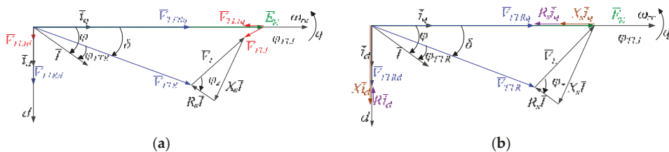
Figure 4. Vector diagram of AC variables: (a) considering V_{TLI} , (b) neglecting V_{TLI} .
