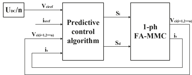
Figure 3. Schematic diagram of the control system.
