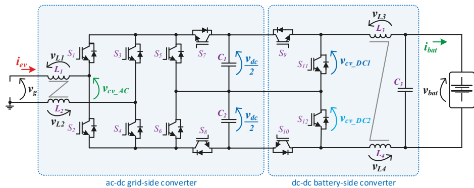
Figure 2. Topology of the proposed on-board electric vehicle battery charger (EVBC).
