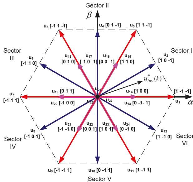
Figure 2. Voltage vectors distribution of T-type inverter.
