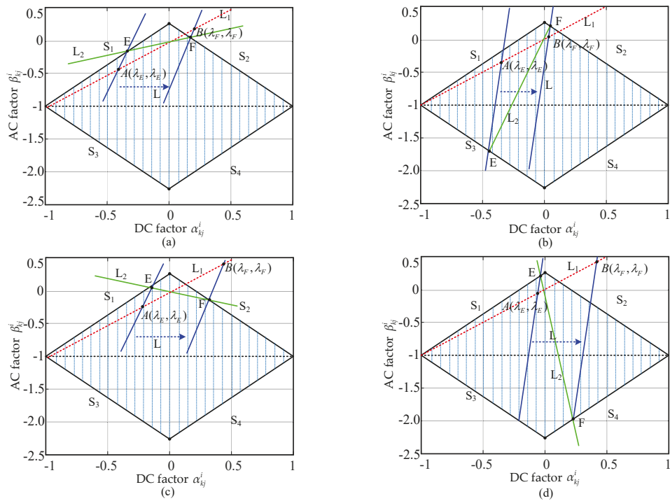
Figure 4. Choosing appropriate DC and AC factor for maximum tolerance in different conditions: (a) when 0 < \eta_{kj} \leq 1 ; (b) when \eta_{kj} > 1 ; (c) when -1 < \eta_{kj} \leq 0 ; (d) when \eta_{kj} \leq -1 .
