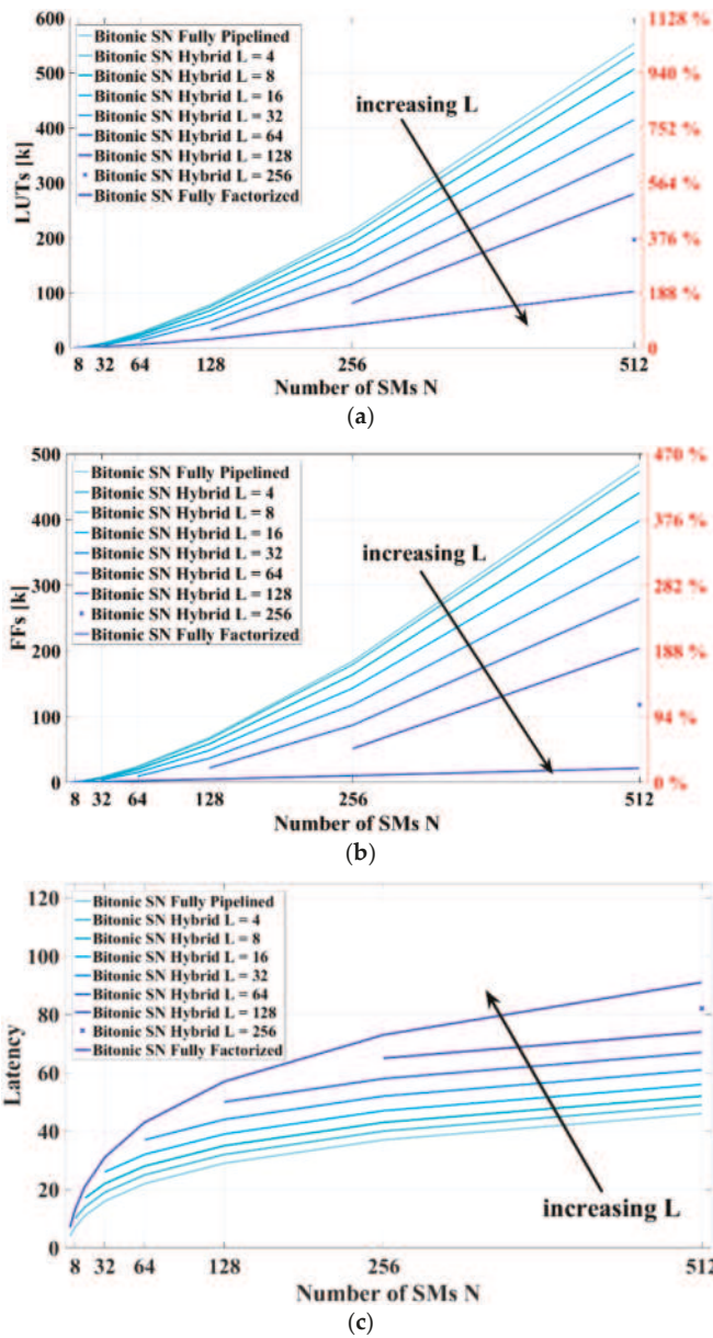
Figure 12. Evaluation of resources and timing performance of the fully pipelined Bitonic SN, the hybrid structure with different factorization level and the fully factorized SN with different input lengths (equal to the number of SMs N ): (a) LUTs; (b) FFs; and (c) latency number.
