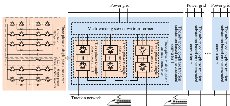
Figure 2. The structure of the advanced co-phase traction power supply system (ACTPSS).
