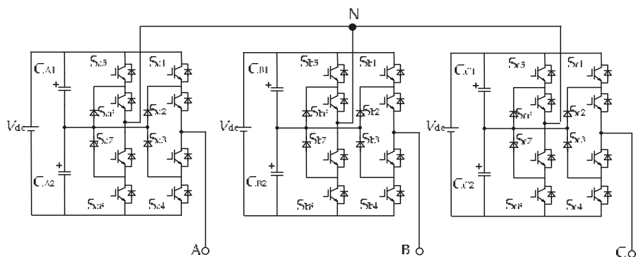
Figure 1. Three-phase NPC/H bridge five-level inverter topology.
