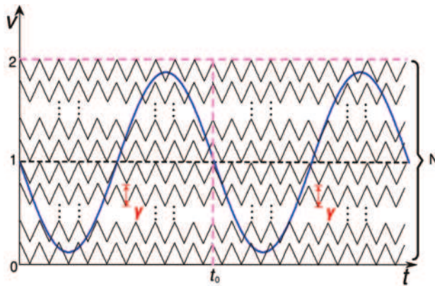
Figure 5. Modulation diagram of one phase under the normal operation.
