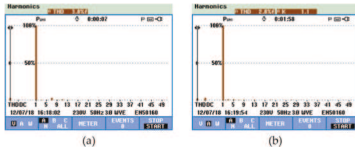
Figure 18. Experimental results in G2V mode of the total harmonic distortion and spectral analysis: (a) power grid voltage ( v_g ); and (b) EVBC current ( i_{ev} ).
