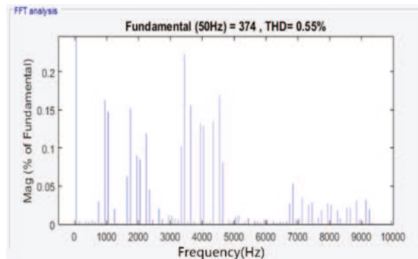
Figure 20. Three-phase four H-bridge CHB current THD for PS PWM and best switching of non-equal sources.
