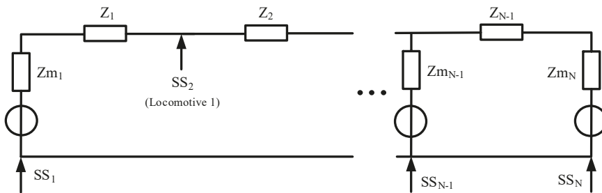
Figure 8. The equivalent mathematic model of ACTPSS.
