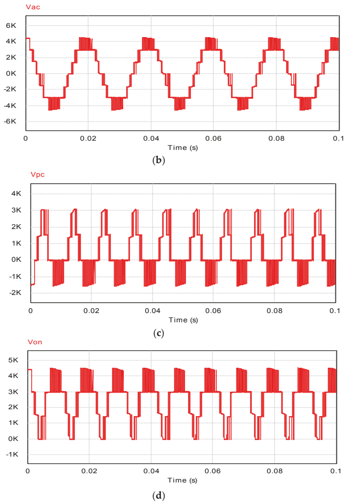
Figure 5. Simulation waveform of the single-phase FA-MMC in steady state operation: (a) Load current and reference current; (b) output AC voltage; (c) voltage of the stack of H-bridges; (d) voltage across the director switches S_1 – S_4 .
