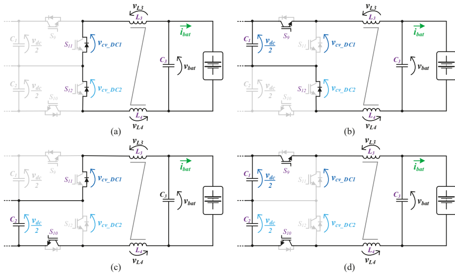
Figure 6. Operation stages for the battery-side converter during the operation as a buck-type converter: (a) The stored energy in L_3 , L_4 is released to the batteries; (b) L_3 , L_4 and the batteries store energy from C_1 ; (c) L_3 , L_4 and the batteries store energy from C_2 ; (d) L_3 , L_4 and the batteries store energy from C_1 , C_2 .
