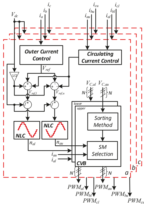
Figure 2. Block Diagram of the MMC FPGA-based controller.
