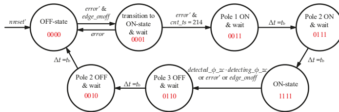
Figure 5. ON-OFF finite state machine.
