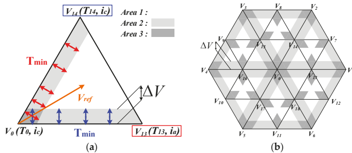
Figure 7. Current-unmeasurable areas (CUAs). (a) Sector 1; (b) reference-voltage vector hexagon.
