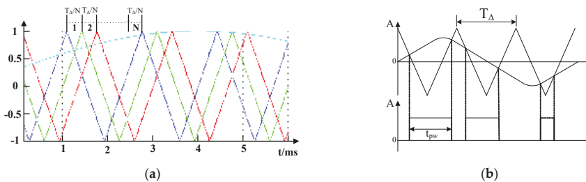
Figure 4. Modulation: (a) Carrier phase-shifted modulation (Different colors represent different carriers); (b) sine pulse width modulation.
