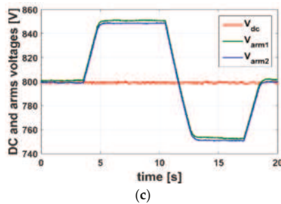
Figure 13. Energy control tests results, (a) DC voltage, upper and lower arms total voltages without an energy control; (b) DC voltage, upper and lower arms total voltages with an energy control and step change in the DC voltage; (c) DC voltage, upper and lower arms total voltages with an energy control and step change of total arm voltages.
