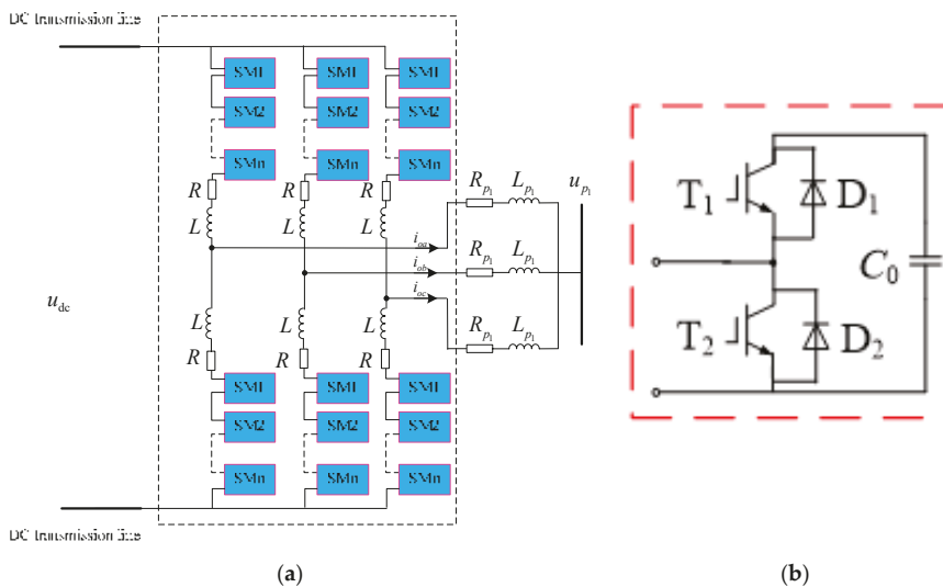
Figure 2. Circuit diagram of MMC: (a) Circuit diagram of the inverter side of a three-phase MMC; (b) Circuit diagram of Sub-Module (SM).
