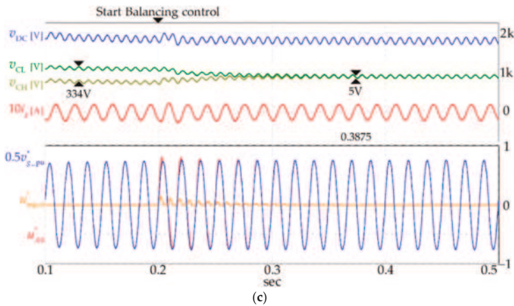
Figure 9. Simulation results for the single-phase NPC inverter with V_{DC} , V_{CH} , V_{CL} and i_g : (a) using distribution factor \mu ; (b) using second-order harmonic component; and (c) using half-wave of second-order harmonic component.
