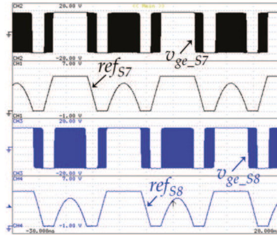
Figure 20. Experimental results showing the modulation technique applied to the IGBTs S_7 and S_8 , namely, the reference signals adopted for the modulation ( ref_{S7} : 1 V/div, ref_{S8} : 1 V/div) and the voltage gate-emitter of the respective IGBT ( v_{ge\_S7} : 5 V/div and v_{ge\_S8} : 5 V/div).
