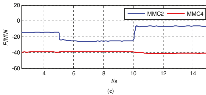
Figure 8. Simulation waveforms of load fluctuation: (a) The active power of the receiving end controlled by double closed-loop control (DCLC); (b) The active power of receiving end controlled by an MPC method based on a finite control set (FCS-MPC); (c) The active power of the receiving end controlled by the hybrid modulated model predictive control (HM 2 PC).
