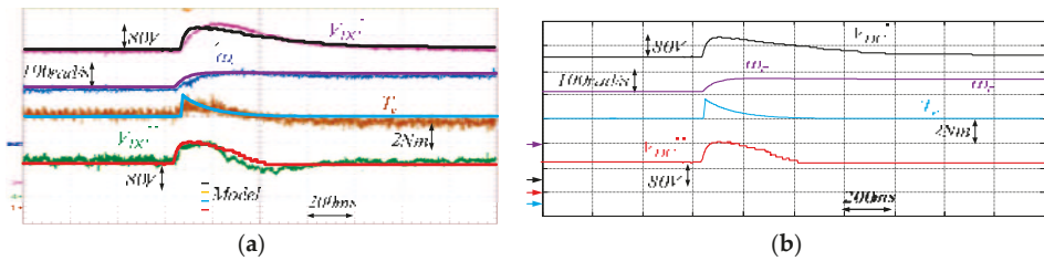
Figure 24. Speed transient from \omega_r = 200 rad/s to \omega_r = 260 rad/s under a constant resistor value R_L = 80 \Omega and V_{DC}' = 400 V, V_{DC}'' = 100 V. Output voltage V_{DC}' , TLI DC bus voltage V_{DC}'' , rotor speed \omega_r , electromagnetic torque T_e . (a) Experimental results. (b) Simulation results.
