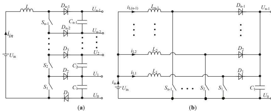
Figure 1. Two interleaved structures: (a) SI; (b) PI.
