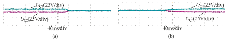
Figure 22. Voltage balance process of C_1 , C_2 when U_{in} is 48 V: (a) from no voltage-balance control to voltage-balance control; (b) from voltage-balance control to no voltage-balance control.
