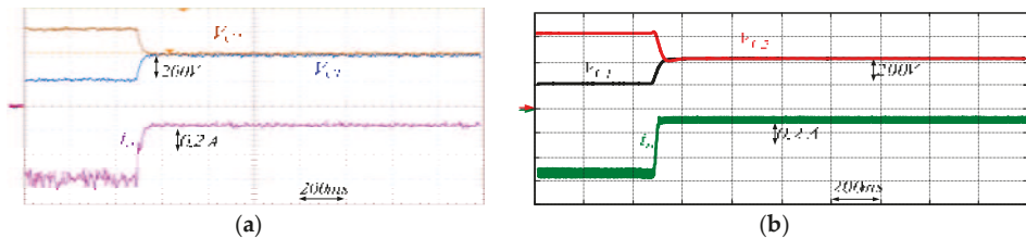
Figure 26. DC bus voltage balancing: T_L = 4 Nm, \omega_r = 200 rad/s and V_{DC}' = 400 V, V_{DC}'' = 100 V. V_{c1} , V_{c2} and i_n . (a) Experimental results. (b) Simulation results.
