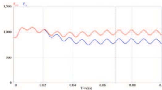
Figure 8. Unbalanced voltage waveforms of upper capacitor V_{CH} and V_{CL} .
