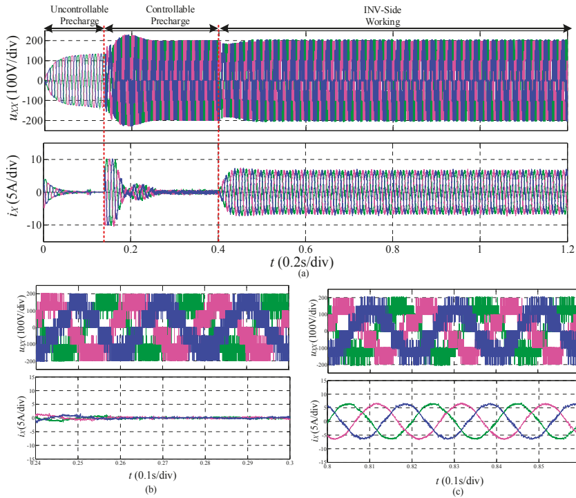
Figure 16. Simulation results of the whole working process; (a) Output voltage–current waveforms, u_{xx} and i_x ; (b) Output voltage–current waveforms, u_{xx} and i_x ; time from 0.24s to 0.3s; (c) Output voltage–current waveforms, u_{xx} and i_x ; time from 0.8 s to 0.86 s.
