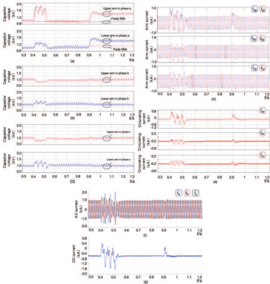
Figure 9. Simulation results of fault condition 1: (a) Capacitor voltage of phase a; (b) Capacitor voltage of phase b; (c) Capacitor voltage of phase c; (d) Arm current of phase j ( j = a, b, c ); (e) Circulating current of phase j ( j = a, b, c ); (f) AC current; (g) DC-link current.
