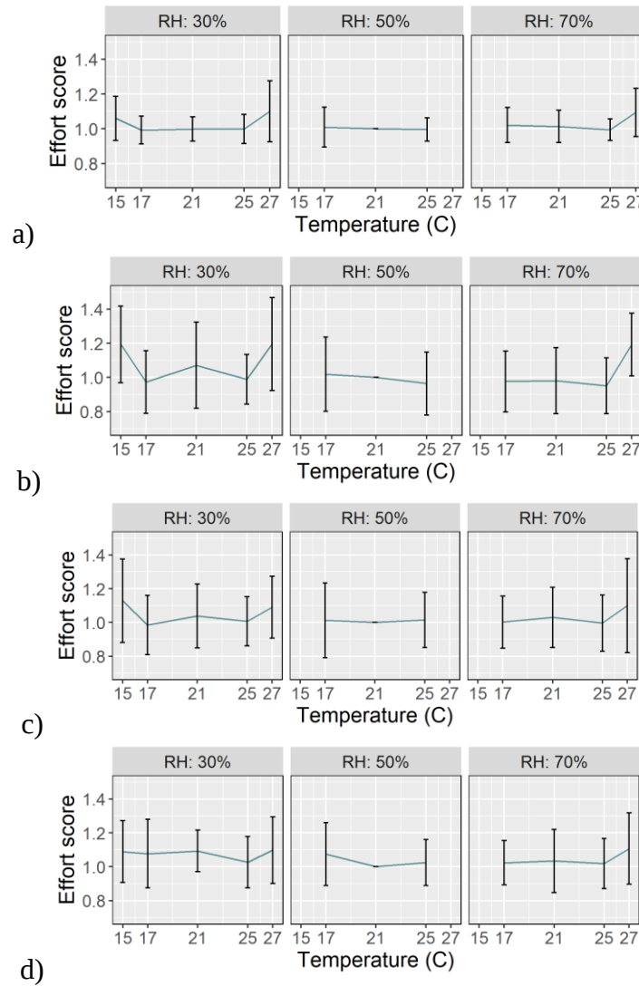
Figure 1. Normalised Effort score changes in tested temperatures and RH levels in each cognitive function. a) Executive function, b) Memory, c) Attention, d) Office simulated tasks. Error bars show the mean \pm SD.
