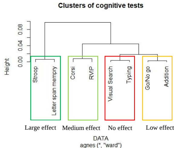
Figure 2. Cluster dendrograms for cognitive tests, Method used: Hierarchical agglomerative clustering analysis (AGNES), Ward method. The high on vertical axis shows the similarity between objects, the higher the fusion, the less the similarity.
