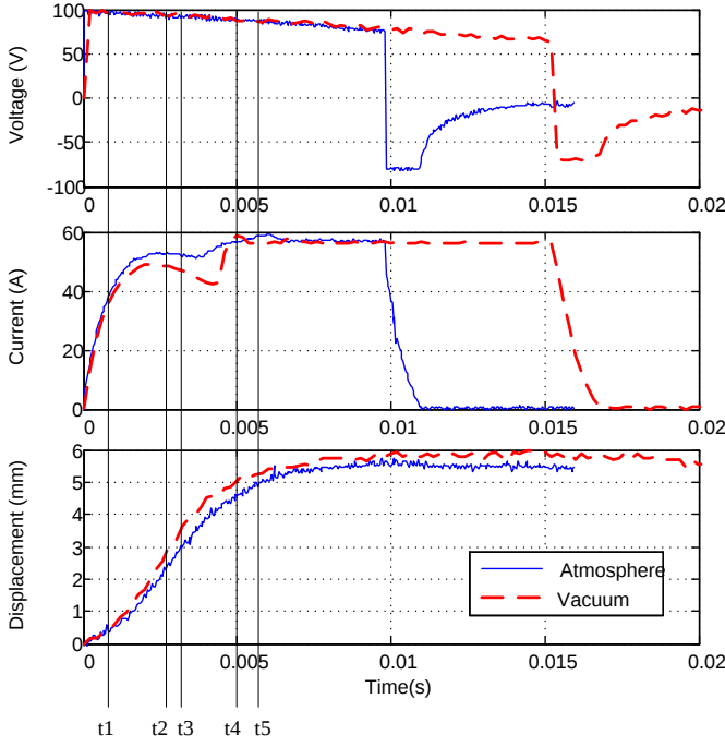
Fig. 15. Opening operation of the vacuum circuit breaker at atmospheric pressure and in the vacuum.
