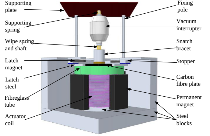
Fig. 9. 3-D structure of the operating actuator
