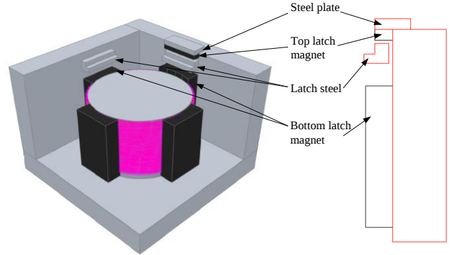
Fig. 8. Geometry of the actuator with magnetic latch (left) and cross-sectional view (right)
