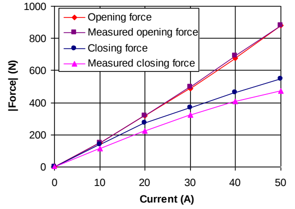
Fig. 13. Actuator opening and closing force versus current.
