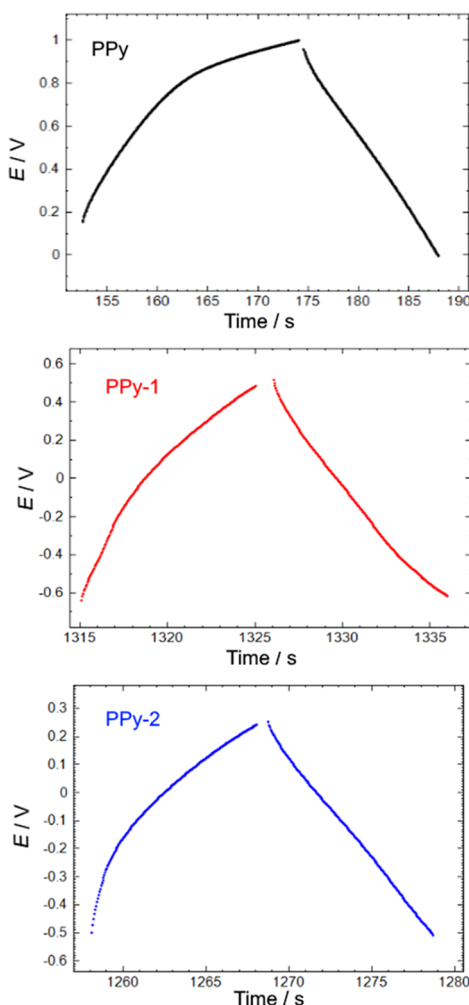
Figure 11. Galvanostatic charge–discharge curves for 10-cycle PPY, PPY-1, and PPY-2 films on GC electrodes. Electrolyte: 0.1 M NBu 4 BF 4 /MeCN at 25 °C vs the Ag wire reference.
