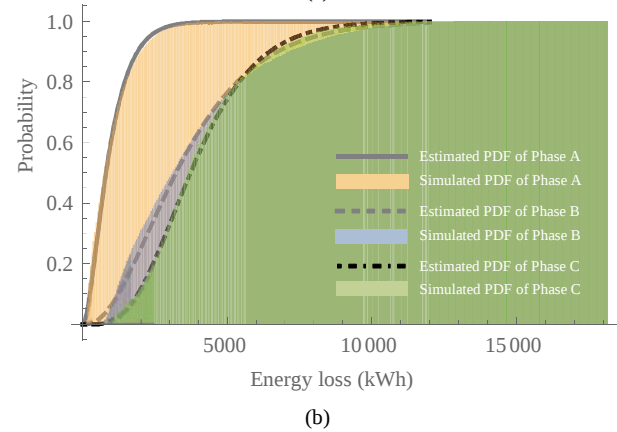
Fig. 4. PDF and CDF of estimated three-phase energy loss. (a) PDF, (b) CDF.
