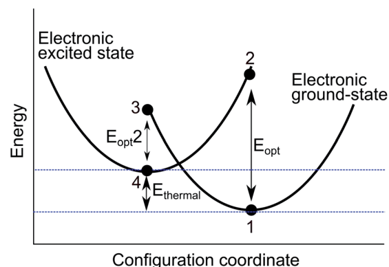
Fig. 2 Configuration coordinate diagram used to illustrate the charge transfer process between two neighbouring cations in the \text{Al}_2\text{O}_3 structure. It contains both an adiabatic charge transfer energy ( E_{\text{thermal}} ), which corresponds to the barrier to thermal activation, and two vertical processes ( E_{\text{opt}} and E_{\text{opt}2} ). The shape of the curves is schematic.
