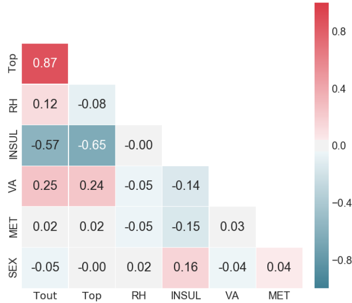
Figure 5. Correlation matrix for the selected variables. Each cell shows the Pearson coefficient, colour coded according to the strength of positive (red) and negative (blue) correlation.
