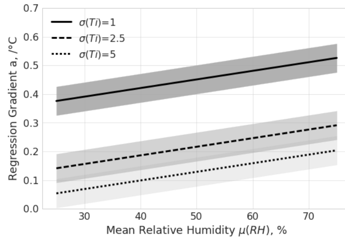
Figure 4. Regression gradient a as a function of the mean relative humidity \mu(RH) for three different values of \sigma(Ti) ; fitted model with 95% confidence bands.
