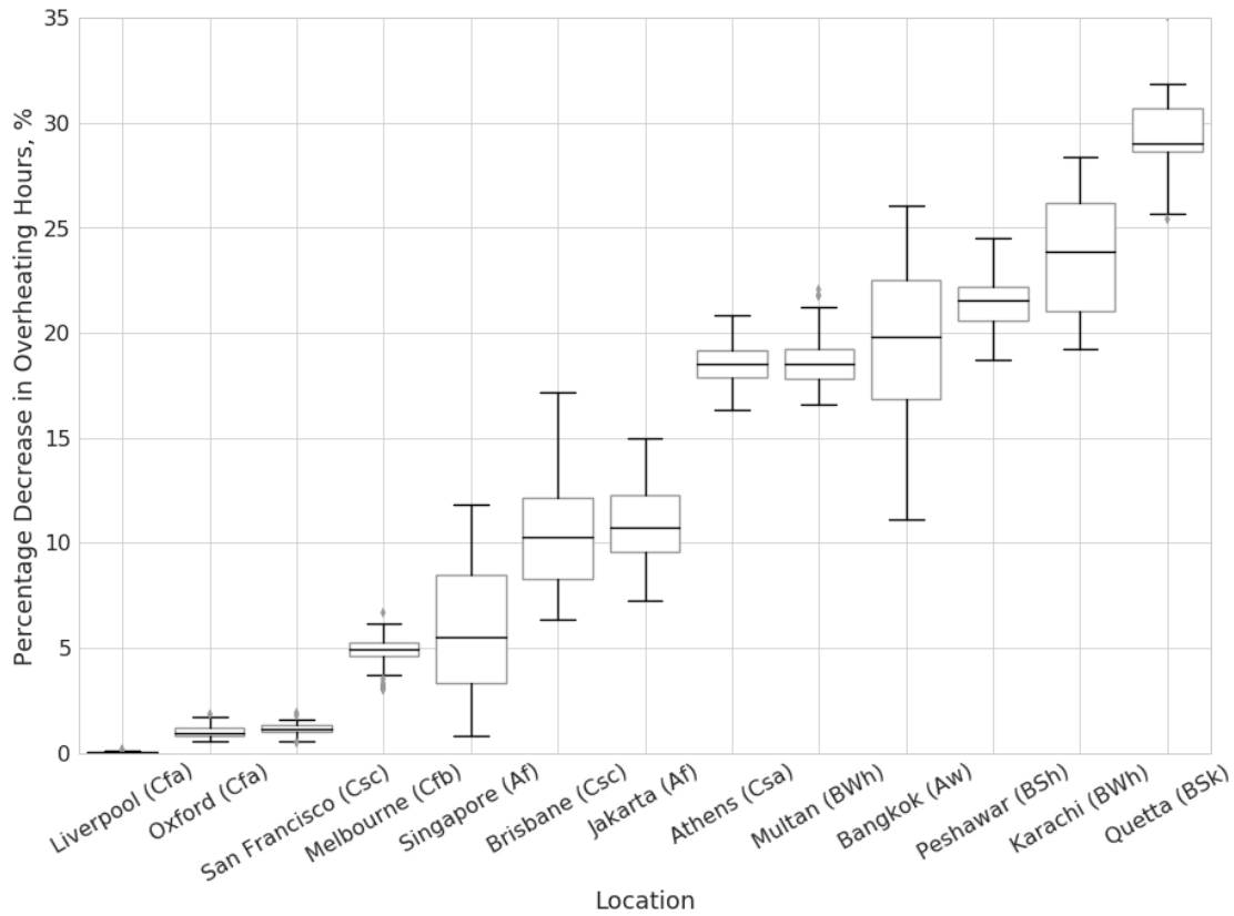
Figure 10. Rank-ordered percentage decrease in overheating hours when using the new adaptive model proposed in this paper in place of the current ASHRAE model. Letters within brackets show the Köppen Geiger climate classification [80] for each location. The box-and-whisker plots represents data from a total of 3,744 simulations.
