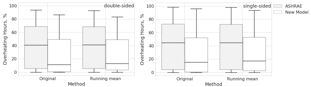
Figure 9. A comparison of overheating hours between the current ASHRAE model and the new model proposed in this paper for double-sided (left) and single-sided (right) offices. Each box-and-whisker plot represents data from 468 variants based on differing location, orientation, shading and window openable areas.
