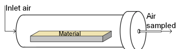
Figure 2: Two-litre chamber schematic.
