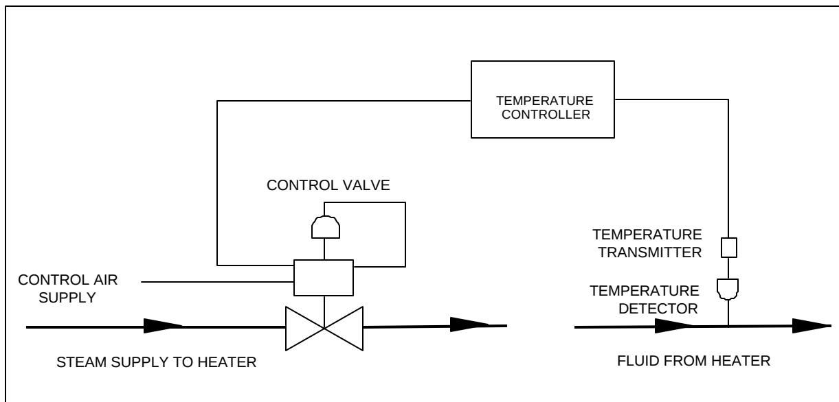
Figure 7-3. Typical Temperature Control Loop
