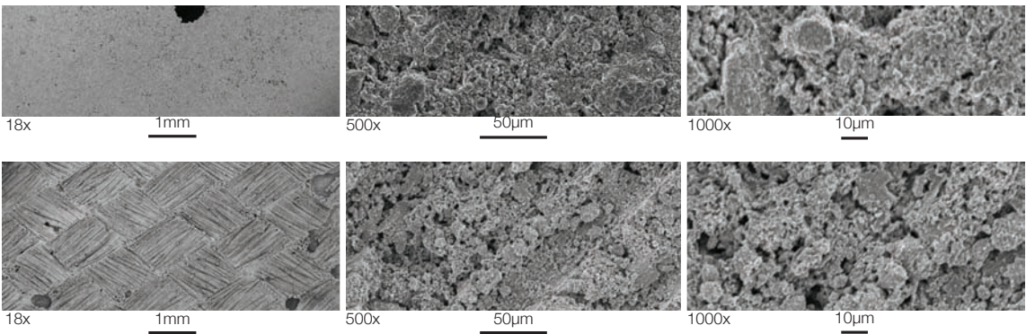
Figure 13: Sample of SEM data at increasing magnification for timber (top) and fabric (bottom) faces.
