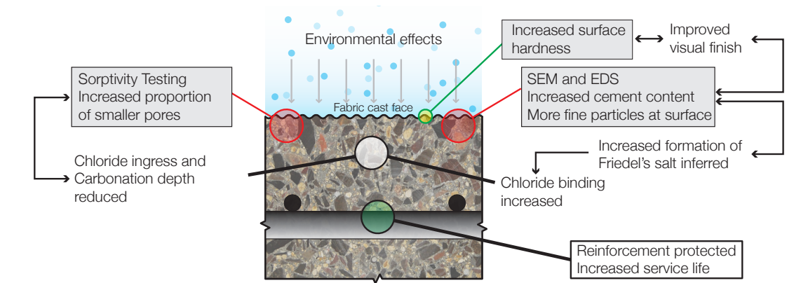
Figure 15: Summary of durability advantages
