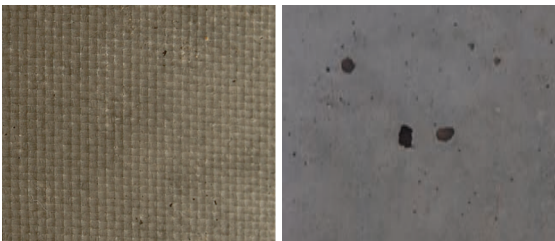
Figure 6: Fabric cast (left) and Timber cast surface (right), from the same concrete mix.
