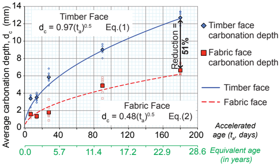
Figure 7: Summary of carbonation measurements.
