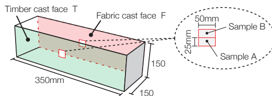
Figure 12: SEM Sample Locations and referencing
