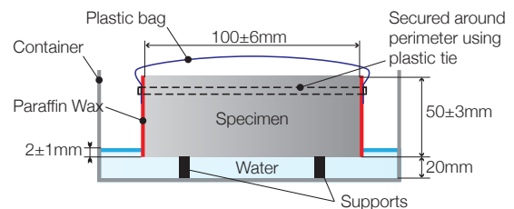
Figure 9: Setup for sorptivity testing.
