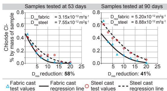
Figure 8: Chloride ingress profile summary.
