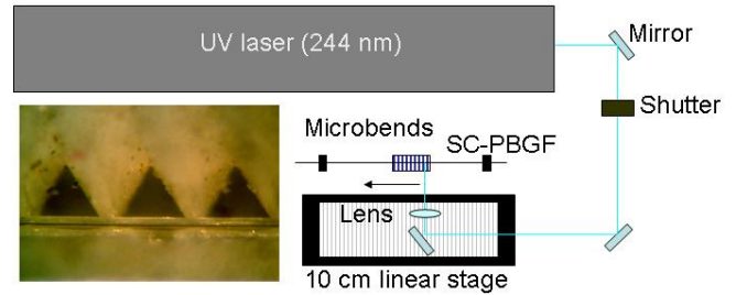
Fig. 3: Schematic of the experimental setup. Bottom left, detail of the threaded rod applied to the SC-PBGF to generate the microbend LPG.
