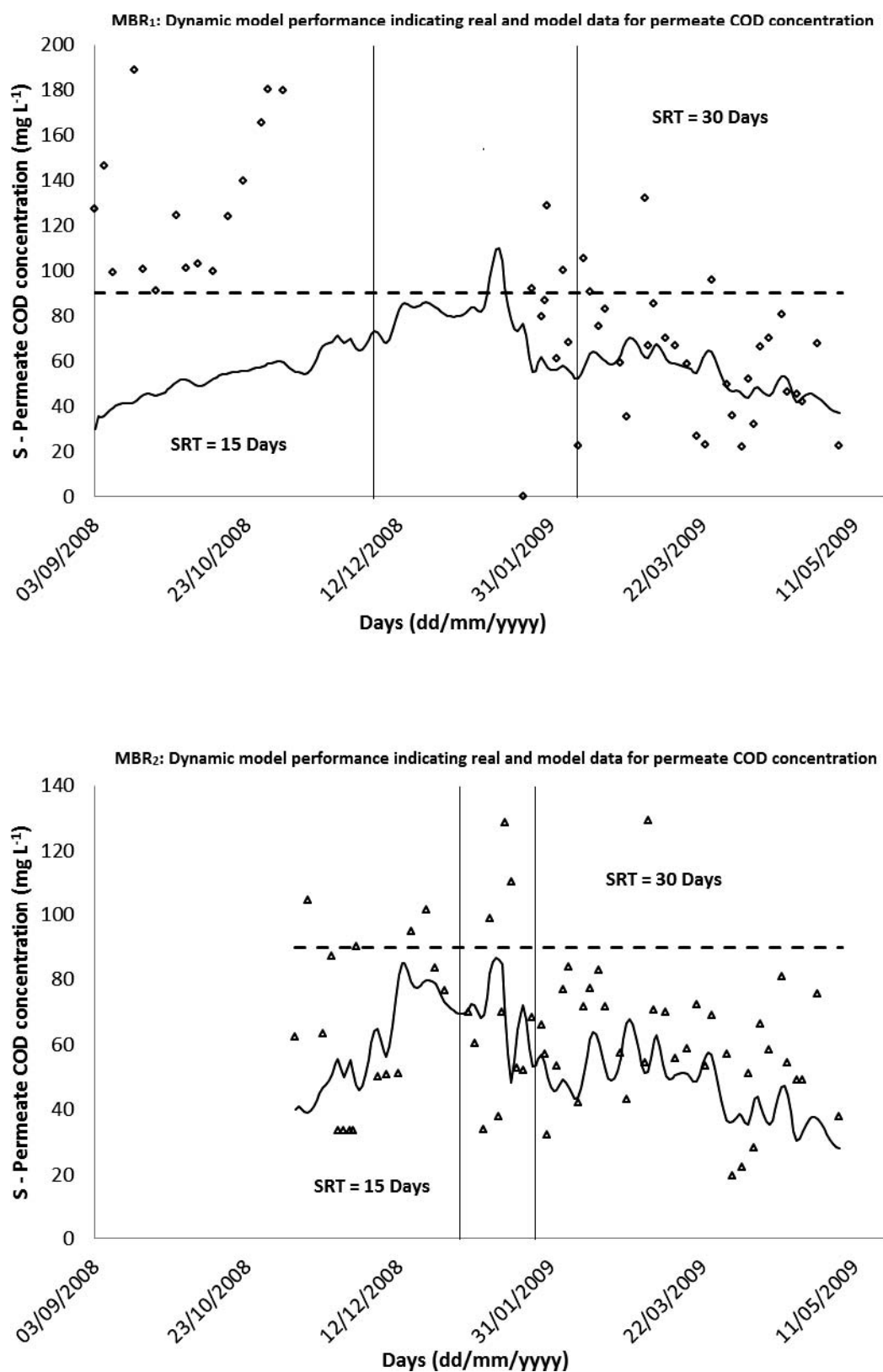
Figure 4—Dynamic model performance for MBR 1 (4a - top) and MBR 2 (4b - bottom) indicating real and model data for permeate COD concentration ( S -value). Note: The horizontal dashed line represents the maximum COD concentration that can be used for unrestricted irrigation in Tunisia, 90 mg L -1 .
