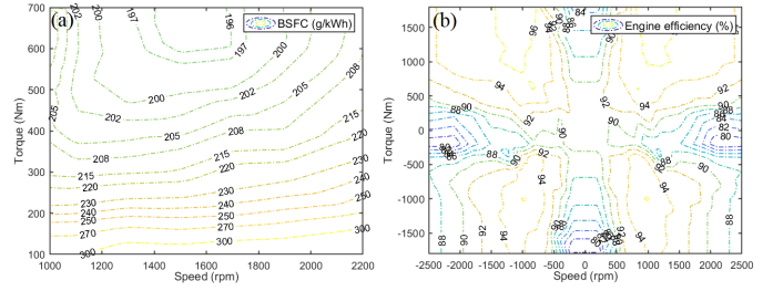
Fig. 4. The (a) fuel consumption map of the engine and (b) working efficiency map of the driving motor.
