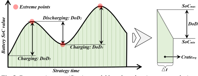
Fig. 3. Battery aging quantification model based on charging event analysis.
