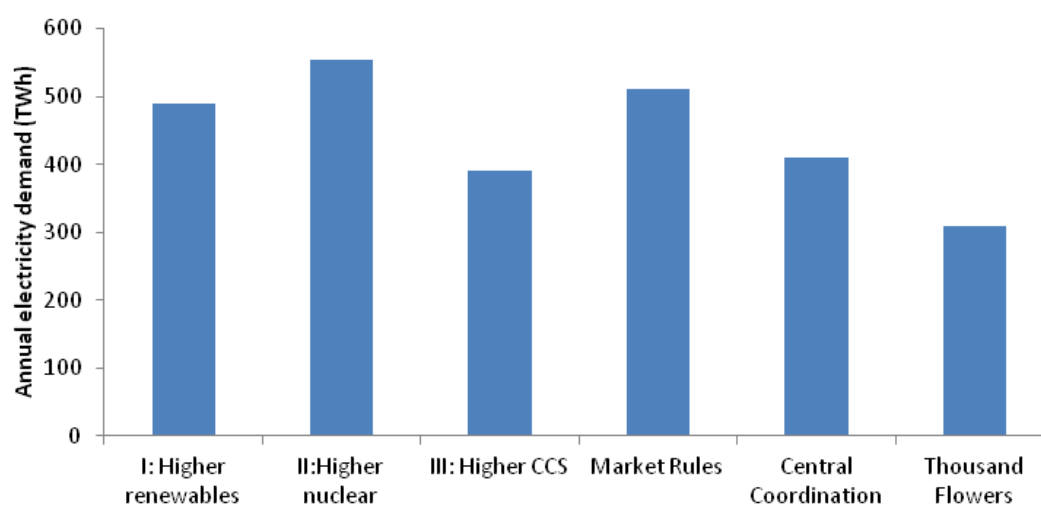
Figure 3. Annual UK electricity demand in 2050 under three DECC scenarios and three Transition Pathways (source: Davies et al. 2013)
