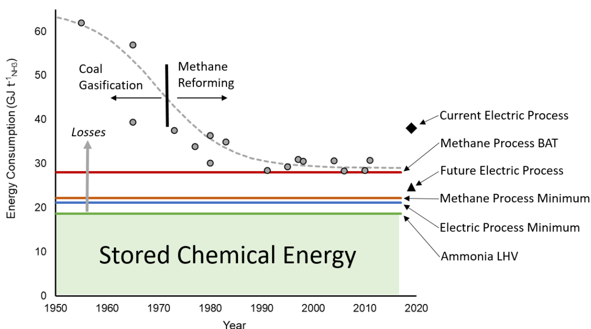
Figure 3: Improvement in the efficiency of ammonia production over the last decades showing actual plant data compared to Best Available Technique (BAT), the minimum energy requirement for a methane-fed plant, the minimum energy for electrolysis ( \text{H}_2 LHV), and current and future electrically driven processes. The amount of energy stored in ammonia is the lower heating value (LHV) and everything above that is losses. Data points acquired from 33, 34 .
