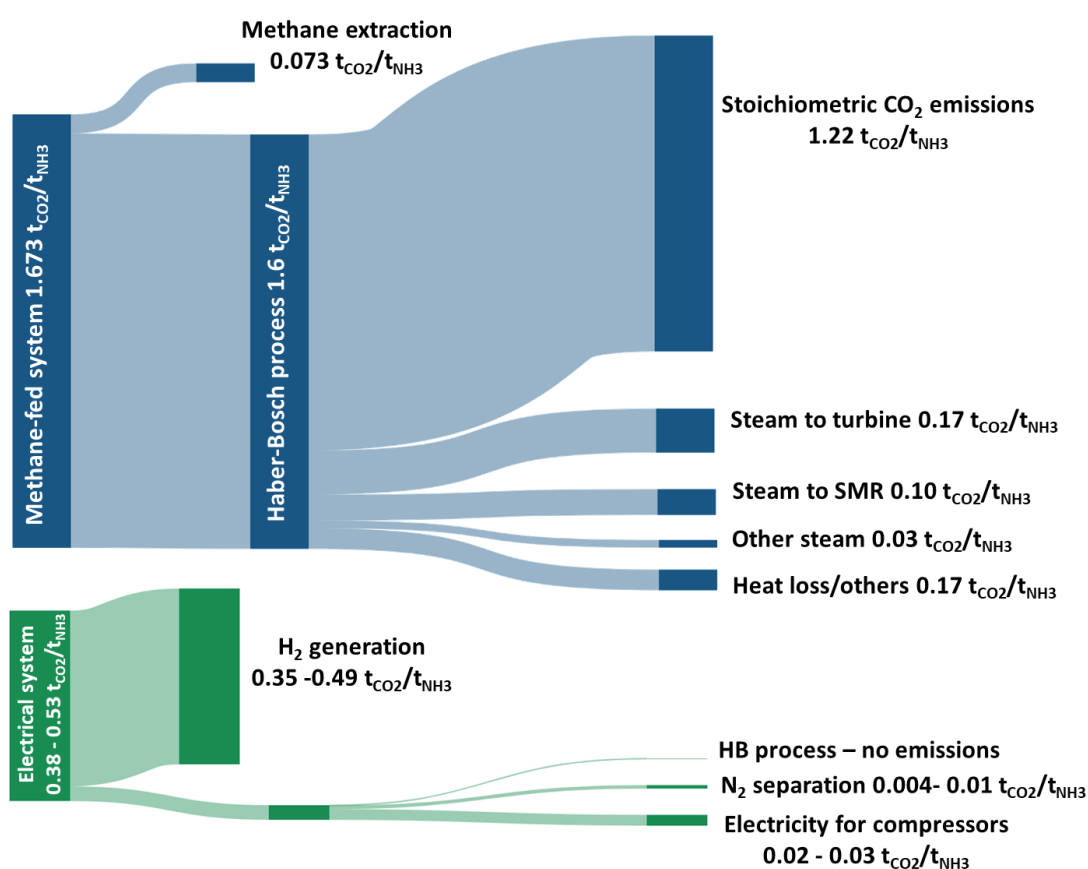
Figure 2: Sankey drawing comparing the attributions of direct CO 2 -eq emissions arising from the methane-fed and the electrically driven Haber-Bosch processes (range of values depend on size of wind turbines). The stoichiometric CO 2 emissions are shown to highlight the minimum level of direct CO 2 emissions that can be achieved by the methane-fed system without carbon capture. The additional CO 2 emissions are allocated proportionally to the significant energy consumers. The figure presents an analysis of data from 25, 29, 30 .
