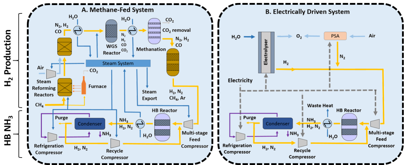
Figure 1: Schematic diagram of A. a typical conventional methane-fed Haber Bosch process and B. an electrically powered alternative. Hydrogen and ammonia production stages are separated for illustration purposes to identify similarities and differences between both technologies. Yellow lines are process gas, dark blue lines are water/steam, light blue lines are air, purple lines are ammonia, and dashed lines are electricity.
