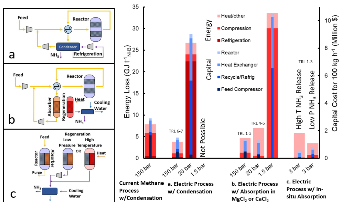
Figure 5: Comparison of energy losses and capital requirements of different HB synthesis loop configurations taking 100 kg NH 3 h -1 as a basis production. In every case the reactor is at 400 °C. The high pressure processes have an operating pressure of 150 bar and either a condenser at -25 °C or an absorber at 300 °C, and approx. 140 bar after a 10 bar pressure drop. The medium pressure processes are at 20 bar, with a condenser at -33 °C or an absorber at 200 °C and 19 bar. The low pressure process is at 1.5 bar with an absorber temperature of 200 °C. The pressure of in-situ absorption is 3 bar with a low temperature (250-300 °C) reactor. In-situ absorbent can be regenerated by either high temperatures (350 – 400 °C) at > 10 bar to subsequently condense ammonia or by release at atmospheric pressure and compressing ammonia before condensation (> 10 bar). Calculations can be found in section S.2 and are meant as estimates for comparison.
