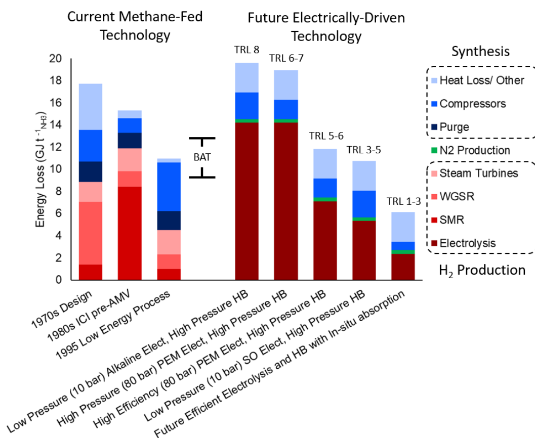
Figure 4: Comparison of methane-fed and electrified Haber-Bosch process energy losses. The data for methane fed processes includes a 1970s 37 , a 1980s 36 , and a 1995 process data 29 . The data for electrically driven process is extrapolated from the methane-fed process using more efficient compressors and typical efficiencies for current alkaline and PEM electrolyzers (60%) 38 , in addition to efficient PEM electrolyzers projected available in the medium term (75%) 39 and SO (80%) 38 electrolyzers. The data for the efficient electrolysis and HB with in-situ absorption includes a hypothetical 90 % efficient electrolyser and a low pressure (3 bar) HB process with in-situ ammonia absorption. Calculations for future technologies can be found in section S.1 and are estimates meant for comparison.
