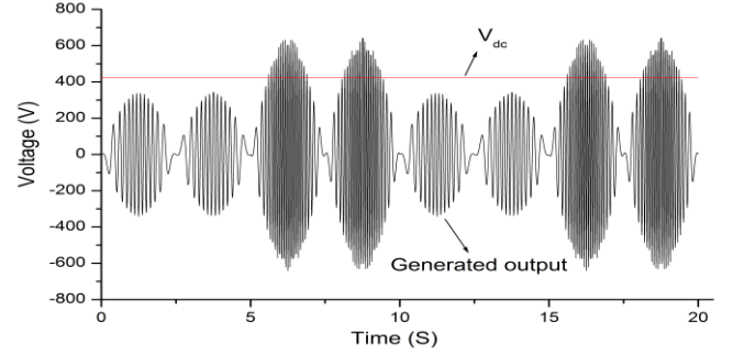
Figure 7: Generated EMFs of DDLWEC and the maintained DC link voltage by SMES-battery system
