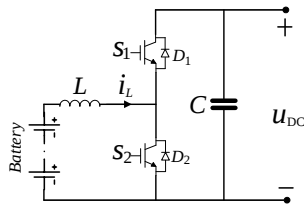
Figure 5: Interface circuit for battery
