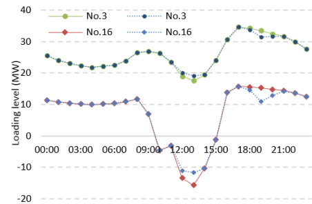
Fig.9: Power flow on the overloading branches
