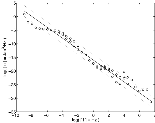
Figure 1. The energy density of electromagnetic fields measured at the surface of the Earth (circles) follows a scaling law which extends over \sim 16 orders of magnitude from \sim 10^{-9} \text{ Hz} to \sim 10^7 \text{ Hz} (solid line). The energy density can be approximated by the scaling law u(f) = u_0(f_0/f)^2 where u_0 \approx 10^{-16} \text{ Jm}^{-3}\text{Hz}^{-1} , f_0 = 1 \text{ Hz} is a scaling constant, and f is the frequency of the electromagnetic field. The measured energy density exhibits deviations from the scaling law by \sim \pm 2 orders of magnitude across the entire frequency range (dotted lines).
