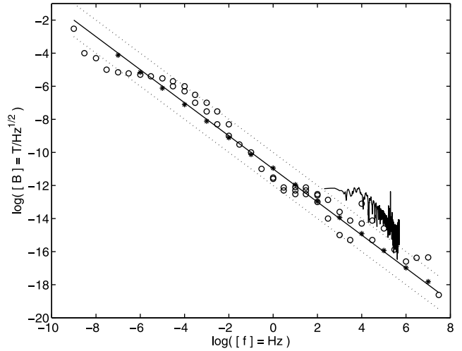
Figure 2. The magnetic field spectrum from \sim 10^{-9} \text{ Hz} to \sim 10^7 \text{ Hz} (circles) can be approximated by the scaling law B = B_0(f_0/f) where B_0 \approx 10^{-11} \text{ T/Hz}^{1/2} , f_0 = 1 \text{ Hz} is a scaling constant, and f is the frequency of the magnetic field (solid line). The measured magnetic field exhibits deviations from the scaling law by \sim \pm 1 order of magnitude across the entire frequency range (dotted lines). The spectrum of an average lightning discharge, which is recorded with a radio receiver at a distance of \sim 510 \text{ km} , exceeds the scaling law by \sim 2 orders of magnitude at frequencies from \sim 0.2 – 400 \text{ kHz} . The spectrum of the lightning discharge is exceeded at 198 \text{ kHz} by the narrow maximum from man made long wave radio transmissions, i.e., BBC radio 4 in the UK. The scaling law is simulated in the frequency range from 10^{-7} \text{ Hz} to 10^7 \text{ Hz} with a persistent normal distributed random noise process (stars) and exhibits an excellent agreement with the scaling law.
