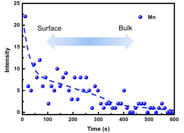
Figure 5. Depth intensity (counts) profile of Mn in the Mn-doped hematite measured with Secondary Ion Mass Spectroscopy (SIMS). Shorter time corresponds to the surface of the sample, while the bulk of the sample is probed at longer time.
