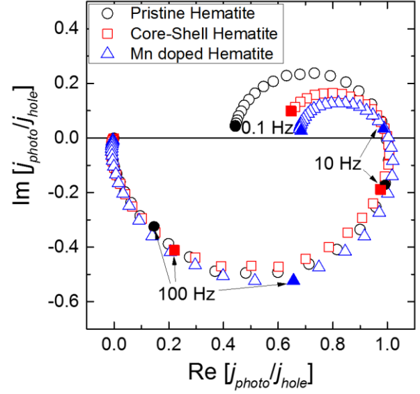
Figure 3. IMPS spectra of pristine, Mn-doped and core-shell hematite samples measured at 1.0 V vs. RHE under blue LED ( \lambda = 455 nm) illumination in 1M NaOH electrolyte solution.
