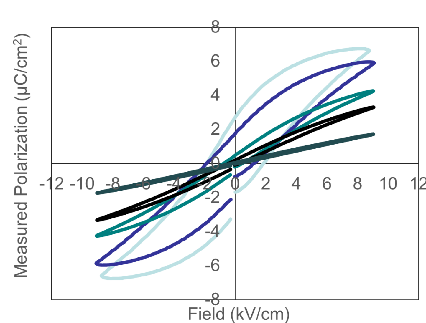
Figure 2: P-E hysteresis loops for BST dense pressed tablet at a range of temperatures from 0^\circ\text{C} to 70^\circ\text{C} .
