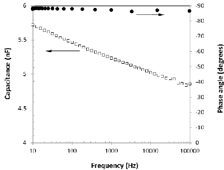
Figure 3. Capacitance and phase angle of piezoelectric device with frequency
