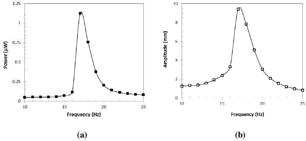
Figure 5. (a) Power and (b) amplitude during vibration. Load resistance is 70.1k \Omega .
