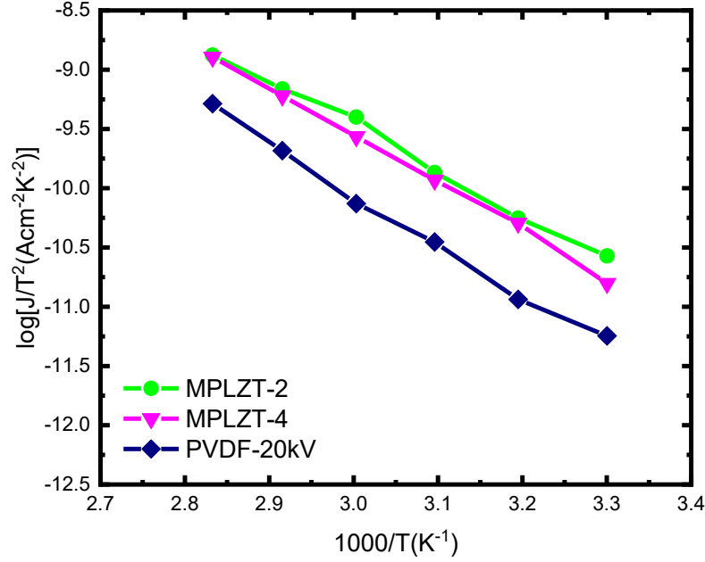
Figure 9. Richardson plots of MPLZT-2 and MPLZT-4 and PVDF-20kV at the applied voltage of 10V.
