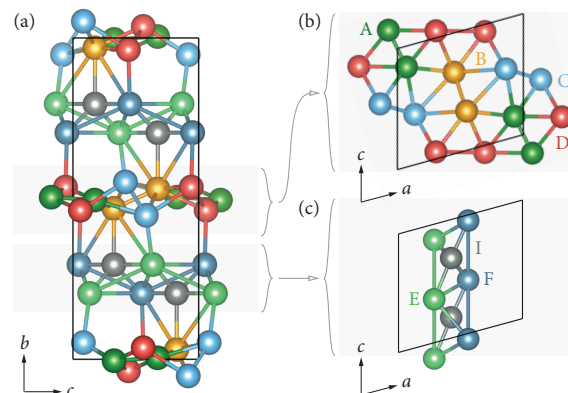
Fig. 5 Illustration of the Li sites with respect to each other.
