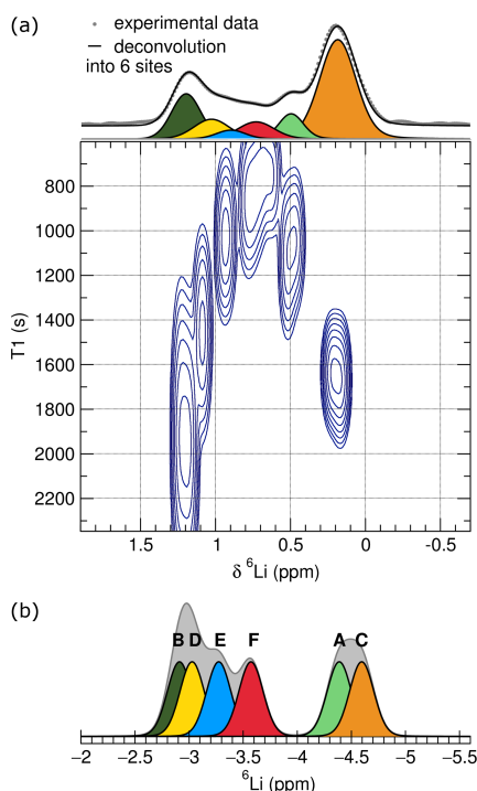
Fig. 4 Experimental and simulated NMR patterns. (a) ^6\text{Li} NMR results for \text{Li}_6\text{Y}(\text{BO}_3)_3 . The contour plot shows the results of the inversion-recovery experiments indicating at least six different Li species. The projection on top represents the added traces of the longest relaxation delay spectra and a fit as a deconvolution into six spectral components. (b) Simulated ^6\text{Li} spectrum of \text{Li}_6\text{Y}(\text{BO}_3)_3 using the DFT chemical shift values for the six crystallographic Li sites and arbitrary gaussian line shapes.
