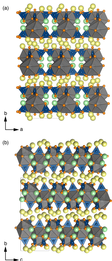
Fig. 1 Crystal structure of \text{Li}_6\text{Y}(\text{BO}_3)_3 . Illustration of the crystal structure of monoclinic \text{Li}_6\text{Y}(\text{BO}_3)_3 viewed along the (a) c - and (b) a -axes. B is shown in blue, Y in gray, O in orange, and Li in yellow or green. Edge-sharing \text{YO}_8 dodecahedra form chains that zig-zag along the c -axis. Trigonal bipyramidal chains of \text{LiO}_5 form along the c -direction and connect the chains of \text{YO}_8 along the a -direction.
