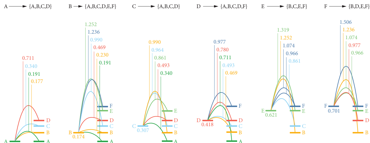
Fig. 6 Calculated energy barriers for vacancy diffusion between each site. Schematic of the calculated minimum energy barriers for all Li–Li site vacancy hops with site separations \leq 4\text{\AA} . All energies are in eV, and give the maximum energy along each minimum-energy path relative to the energy of a vacancy at site Li A . Relative energies of vacancies at sites Li {B,C,D,E,F} are also given.
