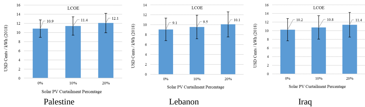
Figure 7. LCOE for solar PV system in the 3 select countries (USD cents/kWh – 2018)
