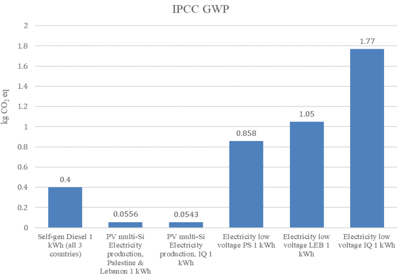
Figure 3. IPCC 2013 GWP 100a V1.03 / Characterization for the three select countries
