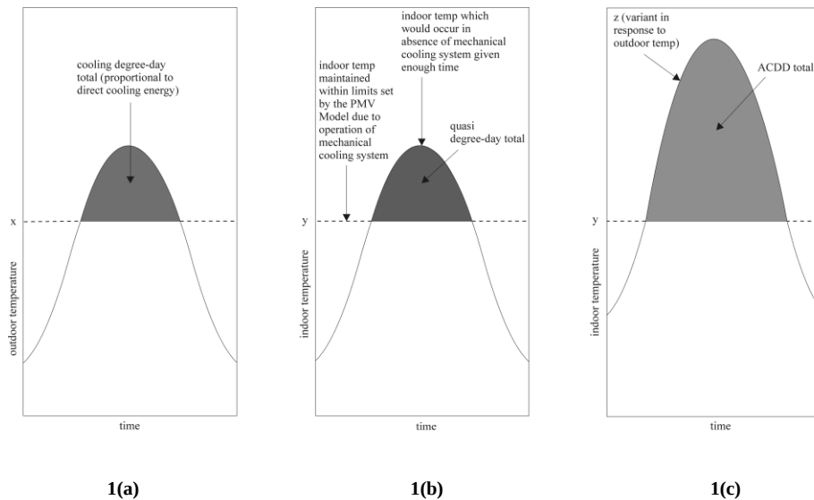
Figure 1 Adaptive Comfort Degree-Day concept explained by analogy with the traditional cooling degree-day – (a) Cooling degree-day total as a function of outdoor temperature and time, (b) Quasi cooling degree-day total as a function of indoor temperature and time, (c) ACDD total as a function of indoor temperature and time
