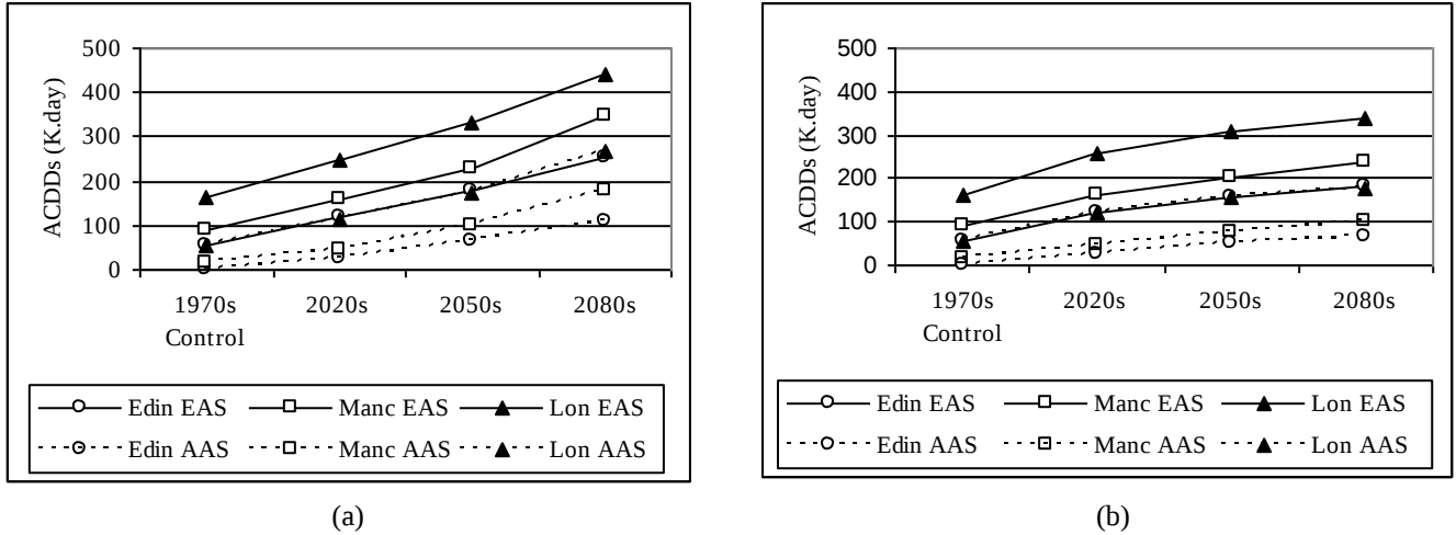
Figure 6 Annual number of cooling ACDDs following implementation of the AAS and the EAS using TRY data for (a) high and (b) low emissions scenarios for Edinburgh (Turnhouse), Manchester (Ringway) and London (Heathrow) for the 2020s, 2050s and 2080s
