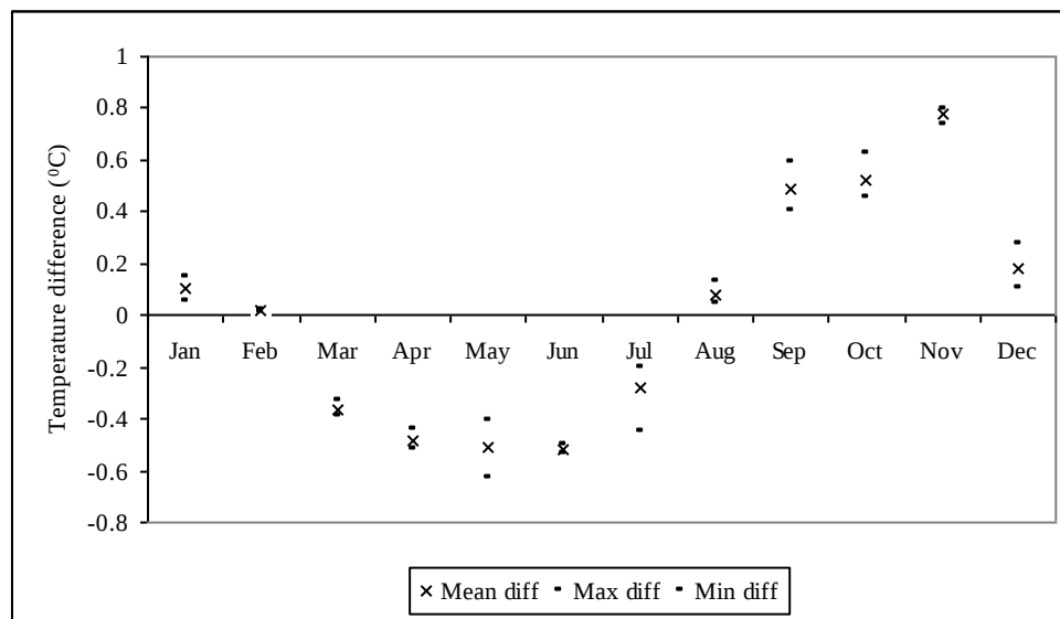
Fig 8 Difference between monthly mean drmm temperatures and monthly mean temperatures for 29700 years of future weather data for Climates I, II and III
