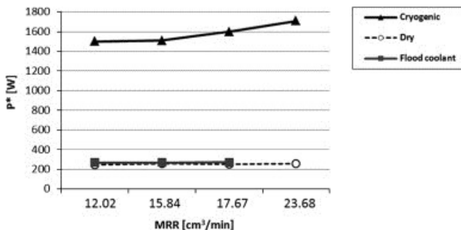
Figure 15, Influence of the material removal rate on the power consumption when machining in different cutting environments.
