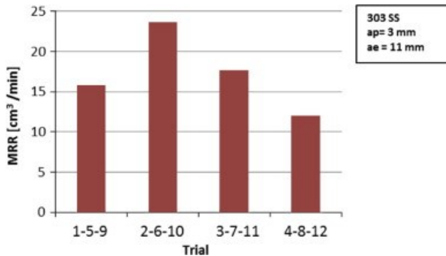
Figure 14. Material Removal Rate for AISI303 stainless steel under different cutting conditions.
