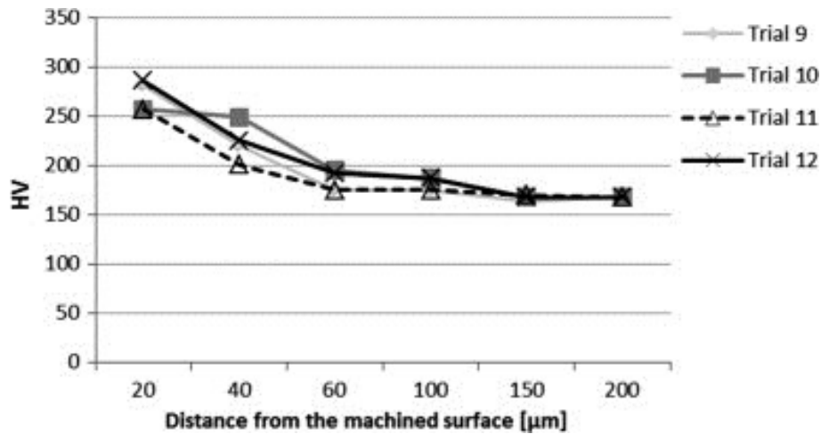
Figure 12, Vickers hardness vs. Distance from the machined surface for samples machined in a cryogenic cutting environment under different cutting conditions
