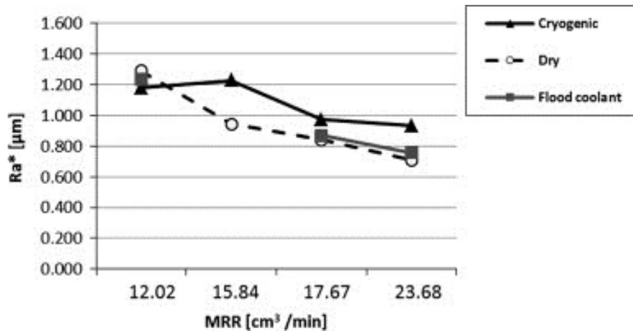
Figure 16, Influence of the material removal rate on the surface roughness when machining in different cutting environments.
