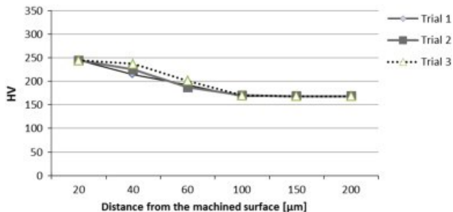
Figure 11, Vickers hardness vs. Distance from the machined surface for samples machined in a dry cutting environment under different cutting conditions
