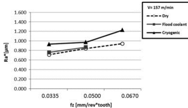
Figure 9, Influence of the feed per tooth on the surface roughness for AISI303 stainless steel machined in different environments with V=157\text{m/min} , a_p=3\text{mm} and a_e=11\text{mm} .
