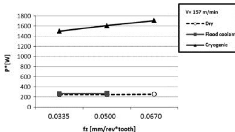
Figure 7, Influence of the feed per tooth on the average power consumption for AISI303 stainless steel machined with V = 157 m/min, a_p = 3 mm and a_e = 11 mm.
