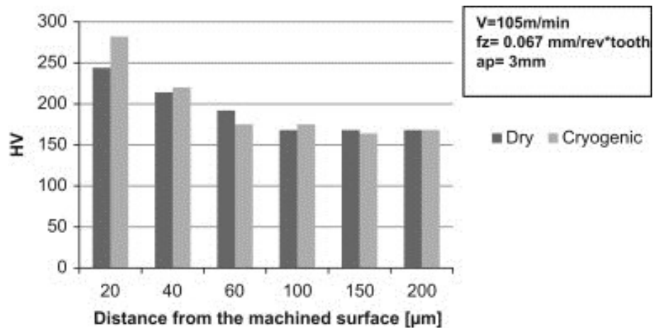
Figure 13, Vickers Hardness vs. Distance from the machined surface for samples cut in dry and cryogenic environment under the same cutting conditions
