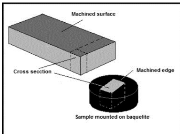
Figure 5, Scheme of metallographic preparation
