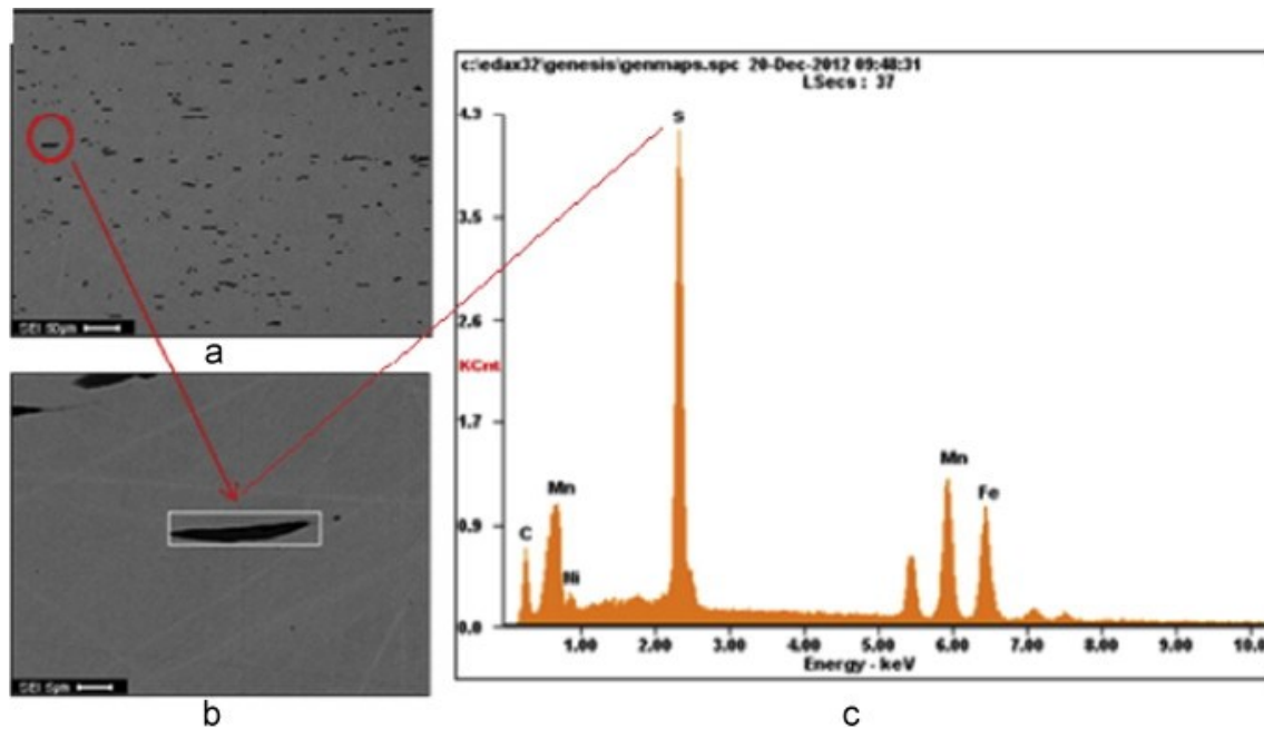
Figure 10, (a) Microstructure of AISI303 Stainless steel 50 (b) detail of elongated black spot and (c) EDAX analysis.
