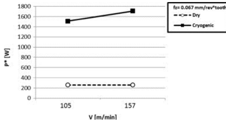
Figure 6, Influence of the cutting speed on the average power consumption for AISI303 stainless steel machined with f_z = 0.067 mm/tooth, a_p = 3 mm and a_e = 11 mm.
