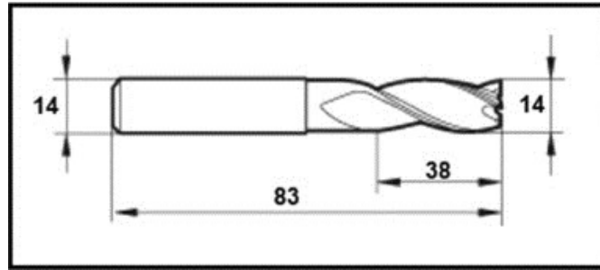
Figure 2, Scheme of the tool geometry
