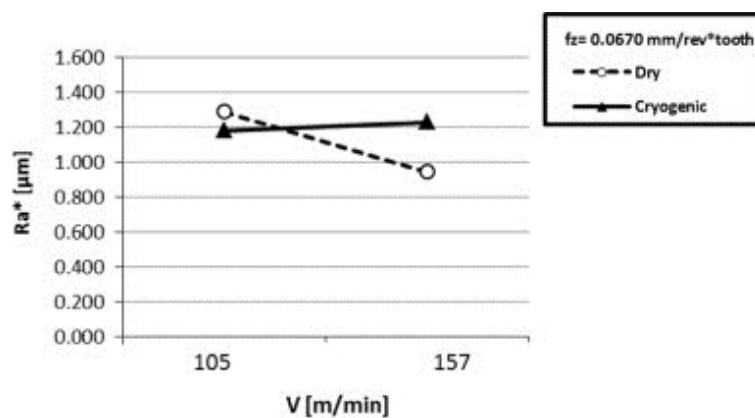
Figure 8, Influence of the cutting speed on the surface roughness for AISI303 stainless steel machined with f_z = 0.067 mm/tooth, a_p = 3 mm and a_e = 11 mm
