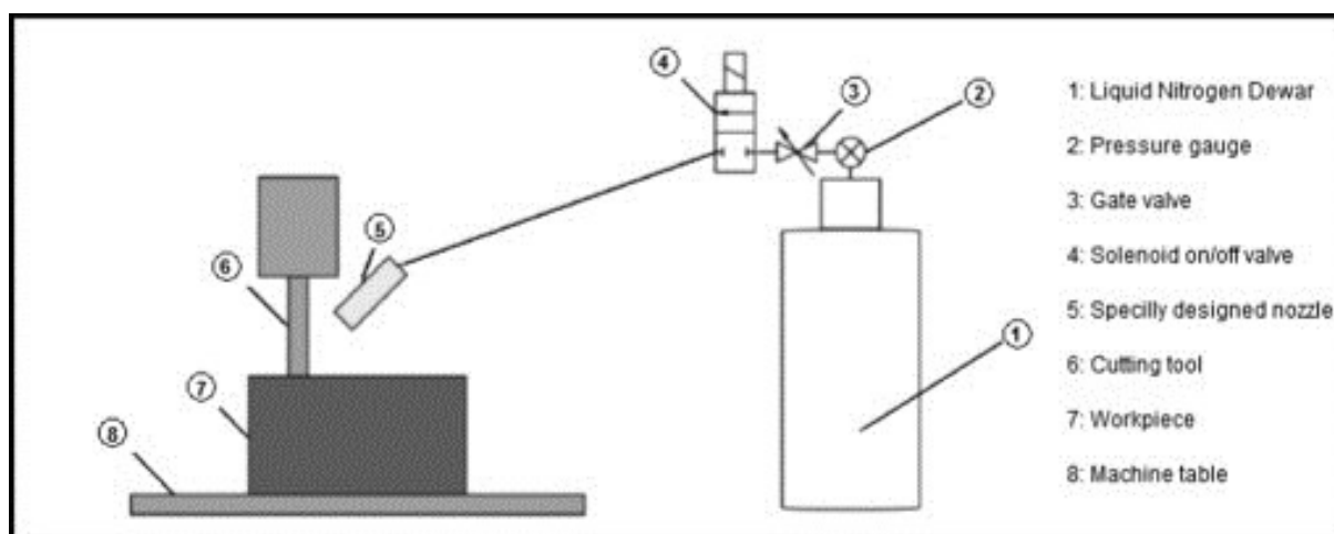
Figure 4. Schematic setup for cryogenic machining [10].
