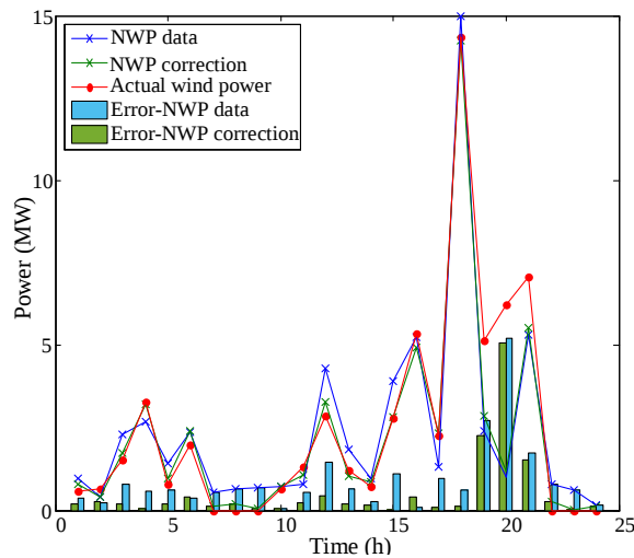
Fig. 12. Wind power forecasting value based on the corrected NWP data in summer
