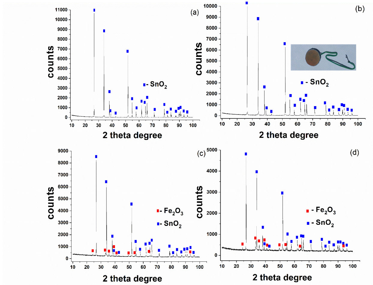
Fig.1. XRD patterns for the Fe 2 O 3 photoelectrodes grown on CuO-Sb 2 O 5 -SnO 2 ceramic substrate at different deposition time of precursor: (a) bare substrate; (b) 10 min; (c) 60 min; (d) 90 min. The inset presents the image of the front side of photoelectrode grown for 10-min.
