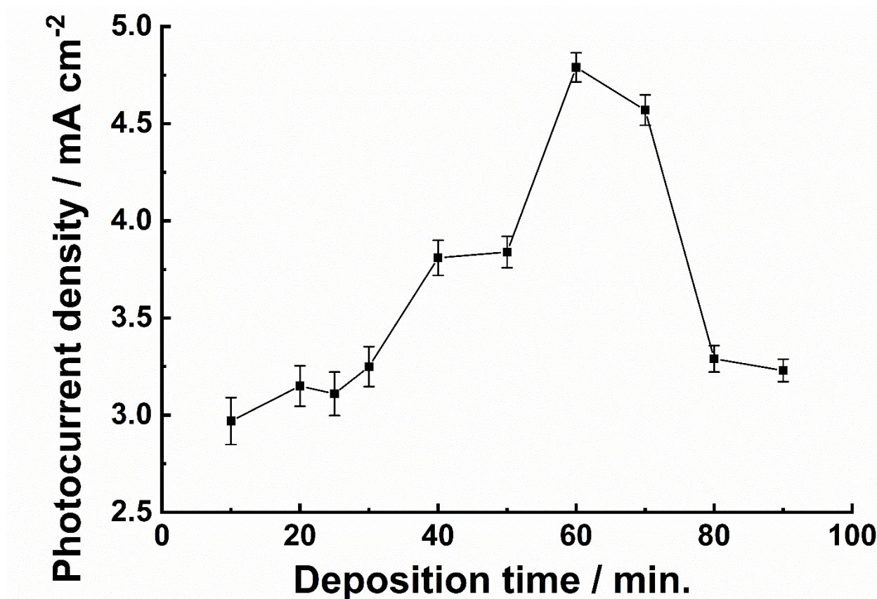
Fig.5. The photocurrent density registered at 1.23V vs. RHE under blue LED's light in 0.1 M NaOH electrolyte for hematite photoelectrodes grown at different deposition time of precursor. The bars show the deviation of photocurrent values from their average values obtained for photoelectrodes grown at the same deposition time.
