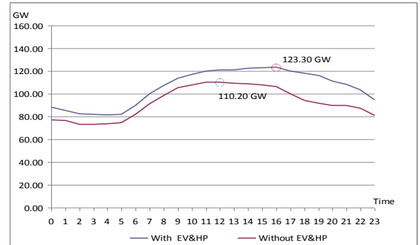
Fig.1. a typical predicted UK demand from file in 2050
