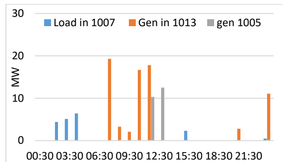
Fig. 6. Load and generation curtailment at selected busbars
