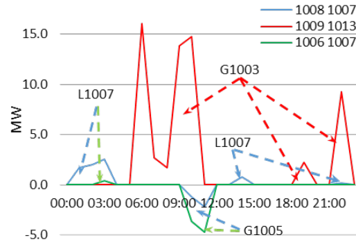
Fig. 5. Overloading levels of selected branches
