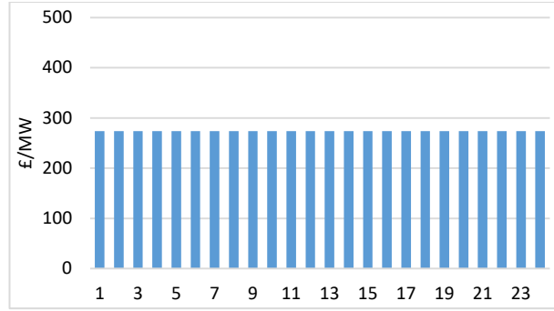
Fig. 7. The economic signal to DR on busbar 1001
