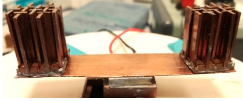
Figure 15. TEG-heatsink assembly geometry.
