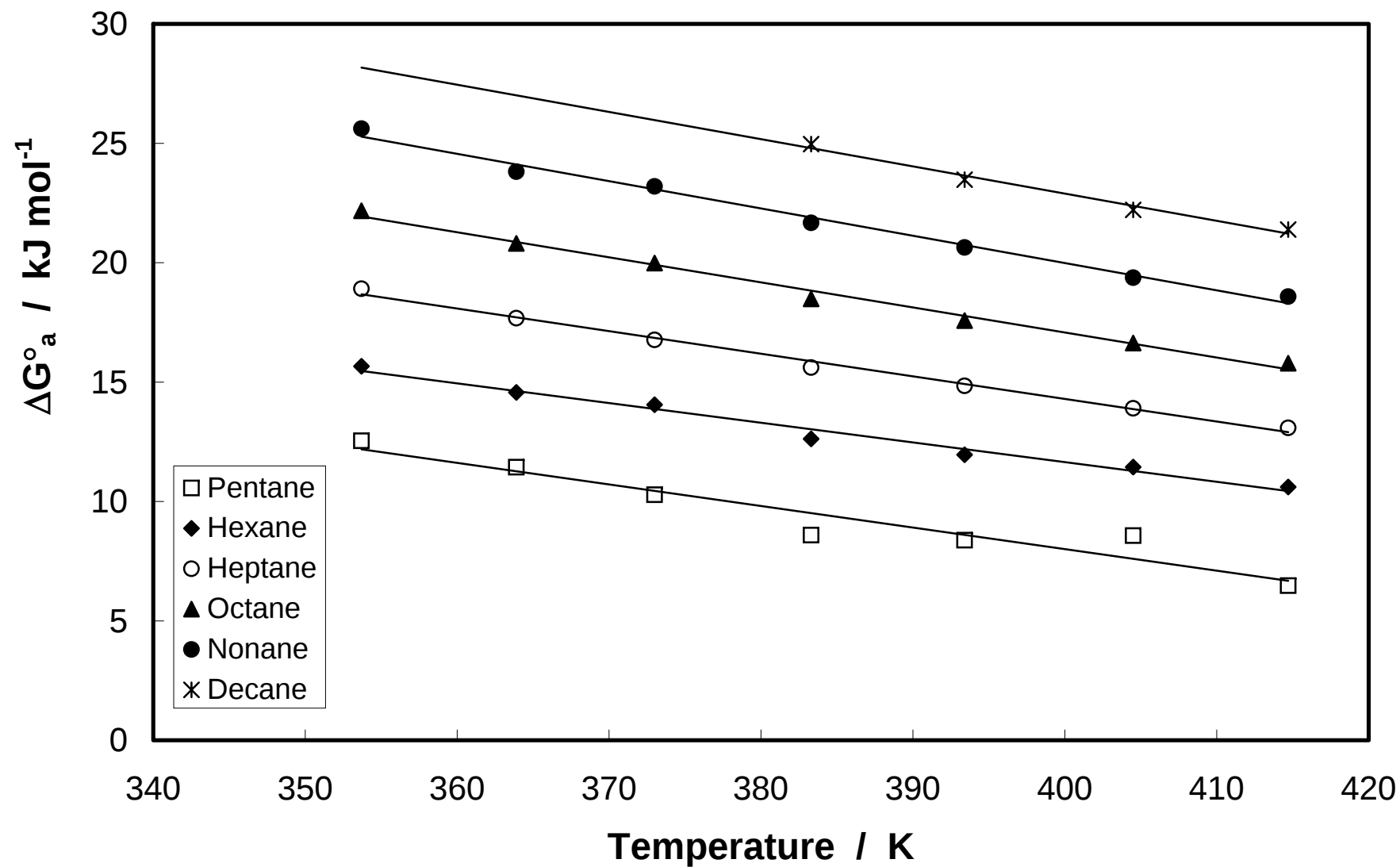
Figure 1: Plot of \Delta G_a^\circ versus temperature for alkane probes on calcined kaolinite CC1 coated with aminosilane.
