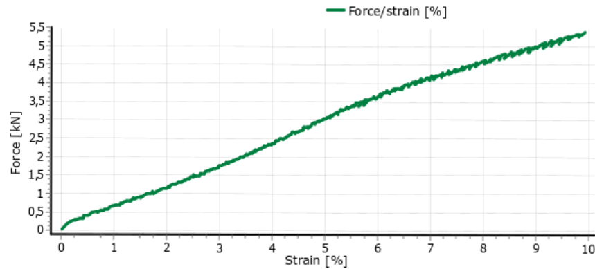
Figure 9: The strain-load relation of the Liros Magic Speed 5mm mooring lines used in the tank testing [30].
