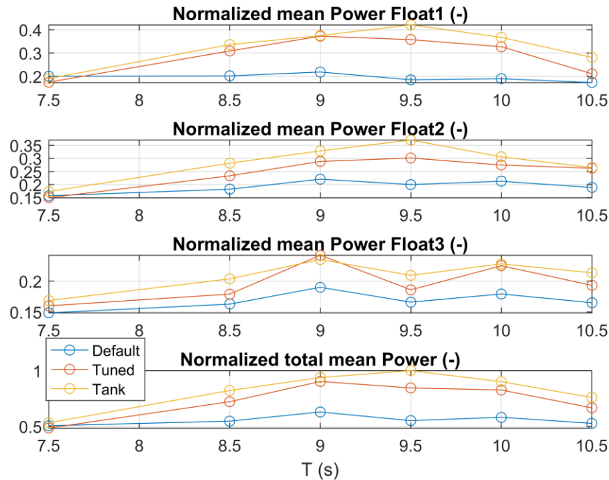
Figure 18: Normalized mean power of each float and of the total system for the default and tuned numerical models and for the tank testing at a full scale. (Single column image)
