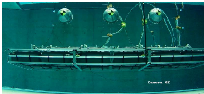
Figure 2: Multi-float model shown in its static position at a medium reactor depth and 2.25D float spacing. (Single column image)
