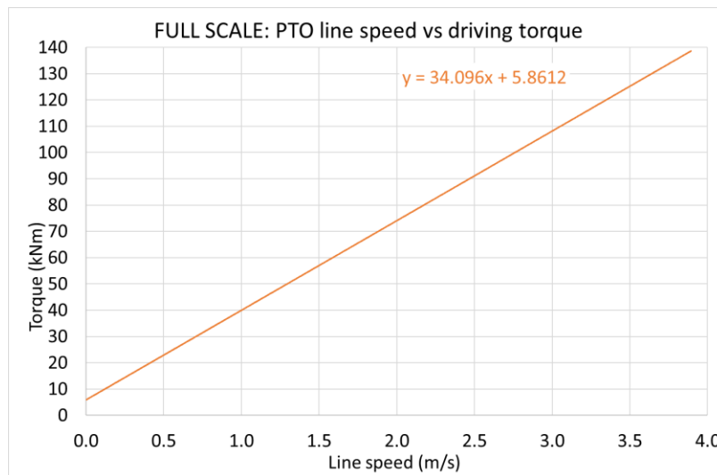
Figure 8: The full scale PTO line speed / driving torque linear relationship (Data scaled from a rig test of the 1:25 tank scale motor and load bank system). (Single column image)
